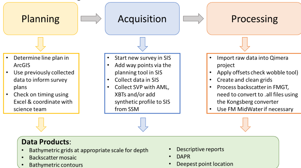
Figure 28: Multibeam processing workflow.
