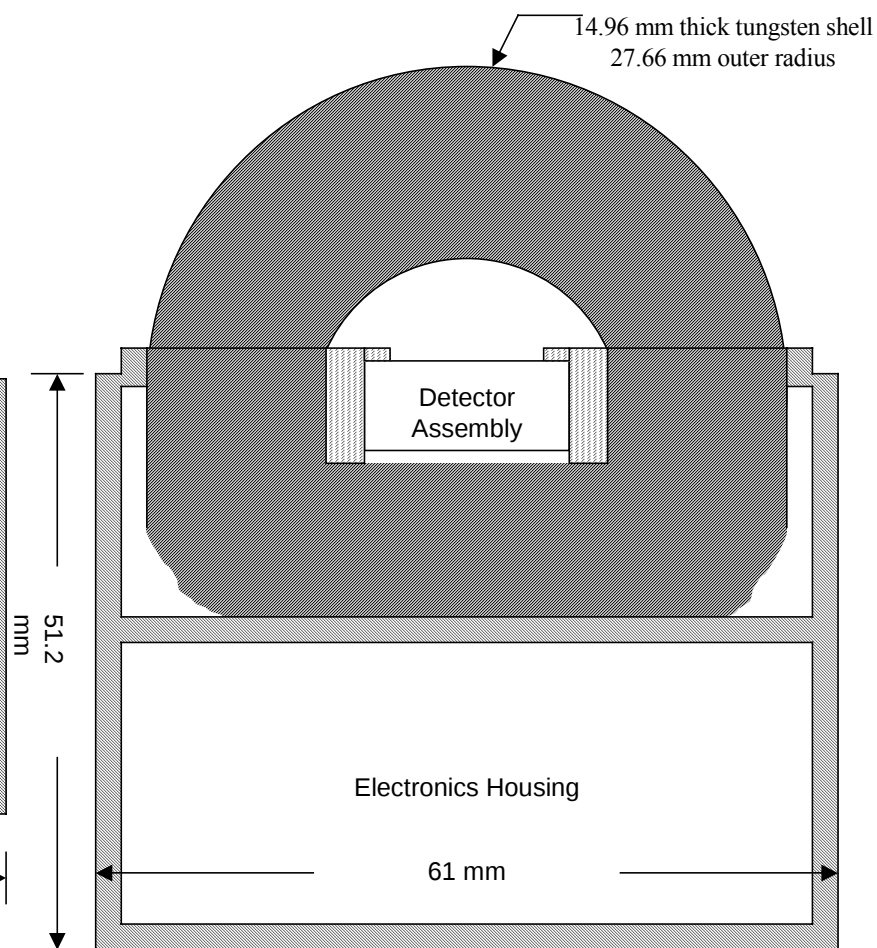
P9 Omni-directional (Dome) detector
