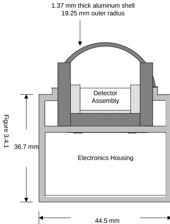
P6 Omni-directional (Dome) detector
