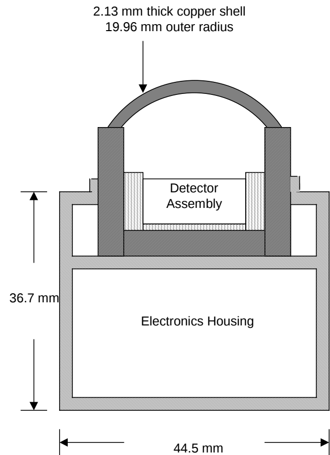
P7 Omni-directional (Dome) detector
