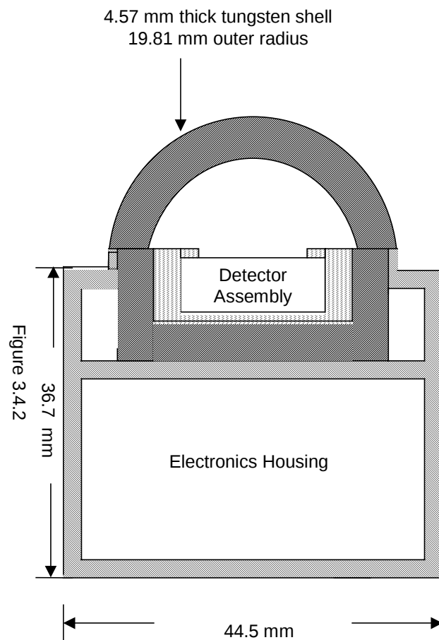
P8 Omni-directional (Dome) detector
