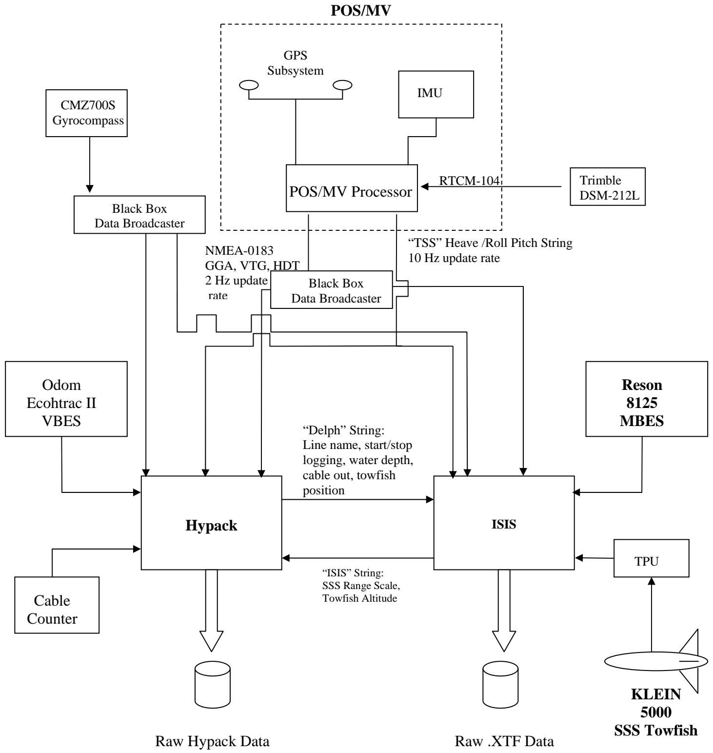
RUDE 2002 Data Acquisition Setup
