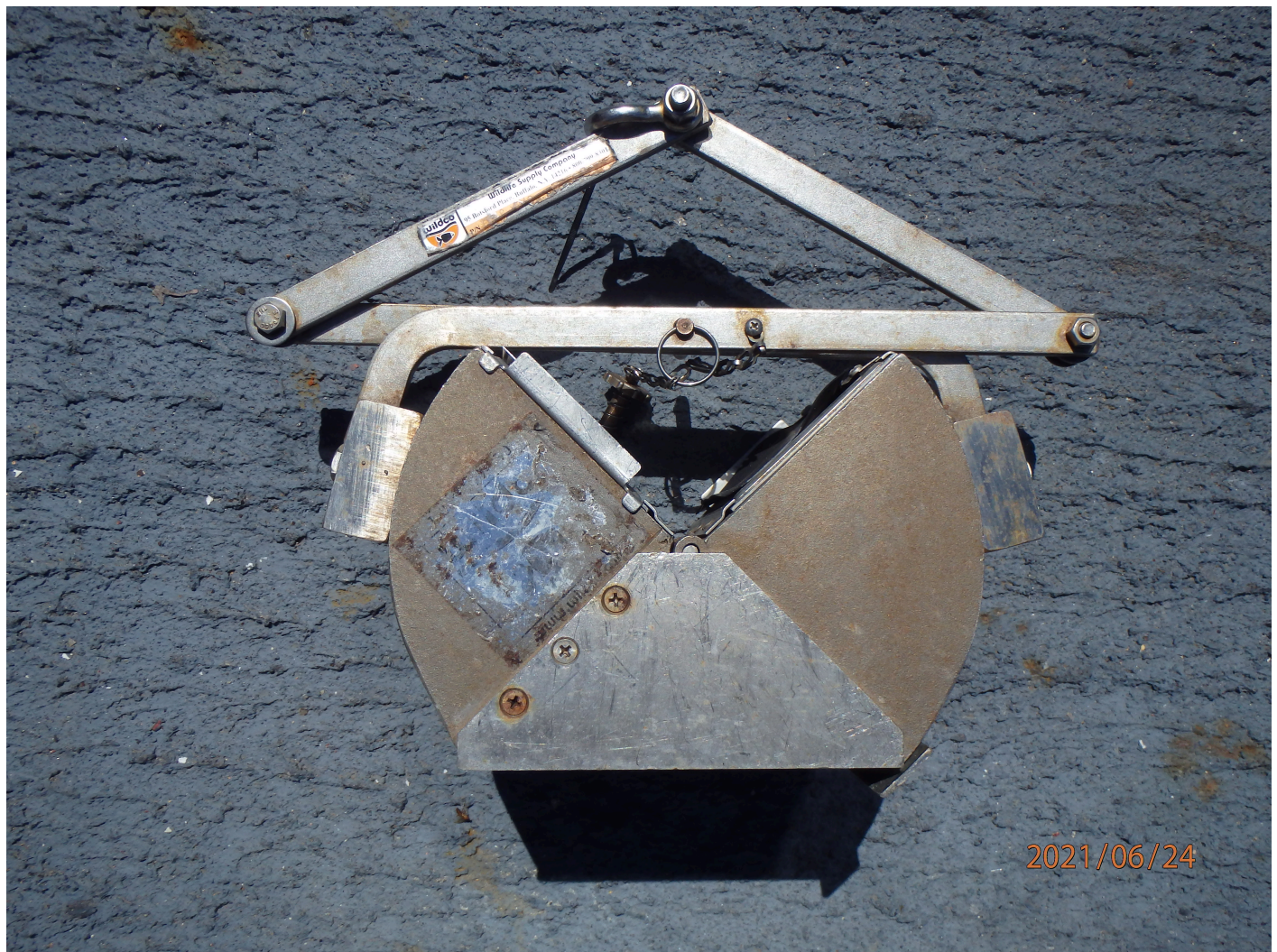
Figure 16: Petite Ponar bottom sampler in open position
