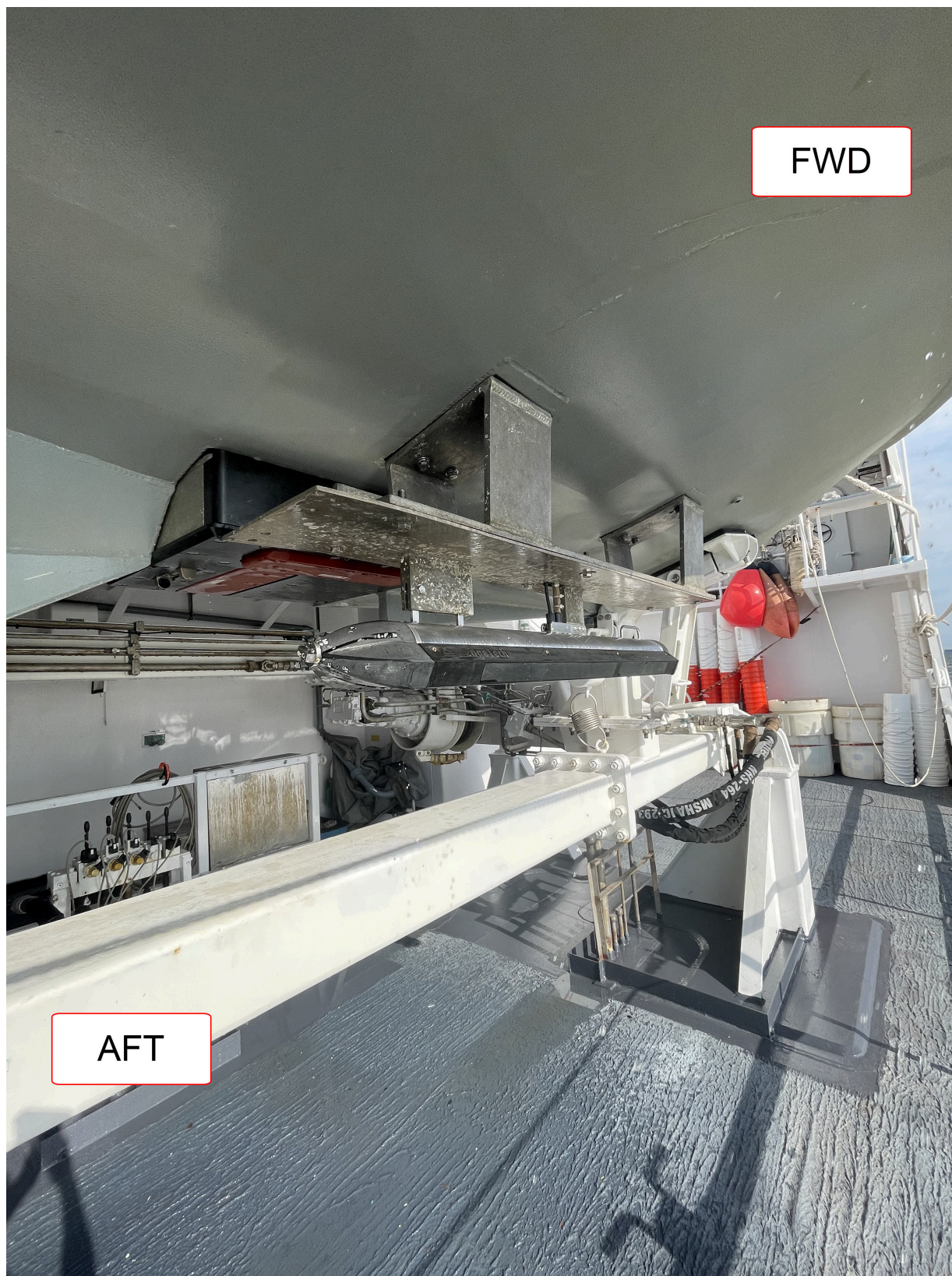
Figure 6: EdgeTech 4200 hull mounted onto 2904
