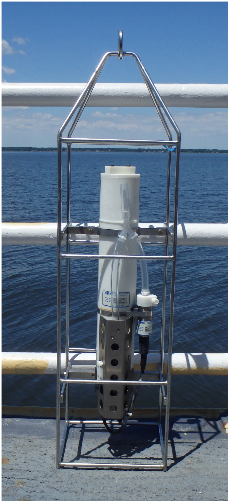
Figure 13: Sea-Bird Electronics SBE 19plus SeaCAT CTD profiler
