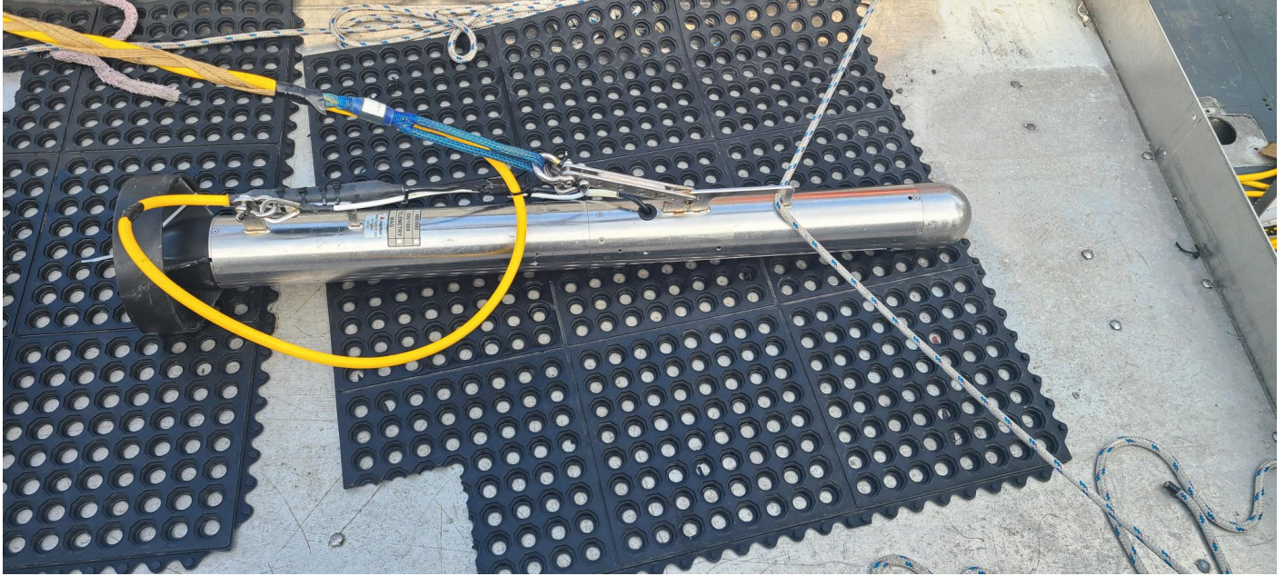
Figure 10: EdgeTech 4125 SSS
