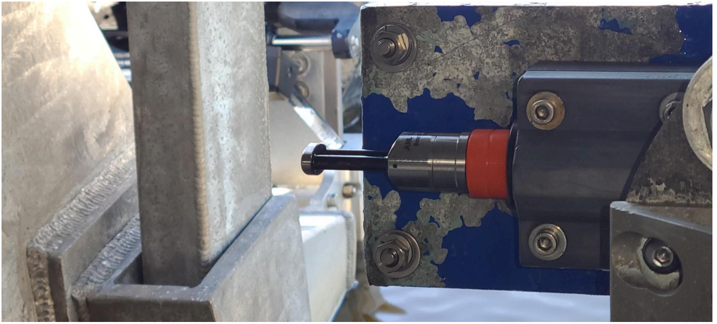
Figure 18: AML 1-RT installed on a R2Sonic 2024
