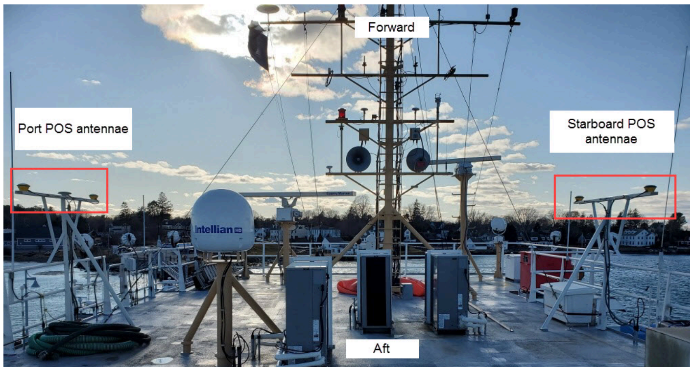
Figure 5: Antennae location on the flying bridge
