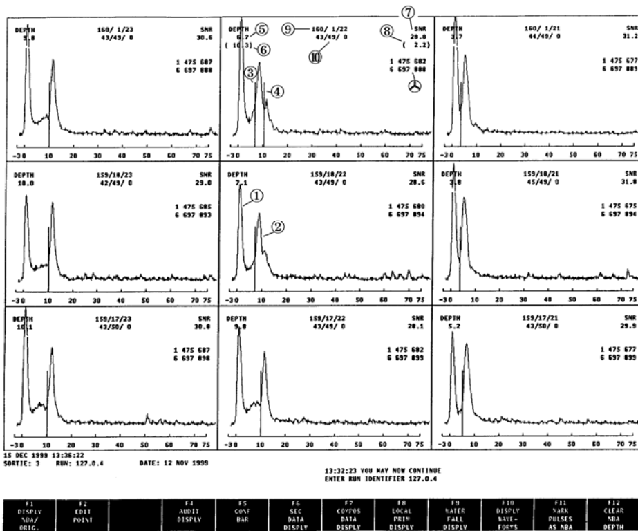
Figure 13 - Annotated Sounding Waveform Display
