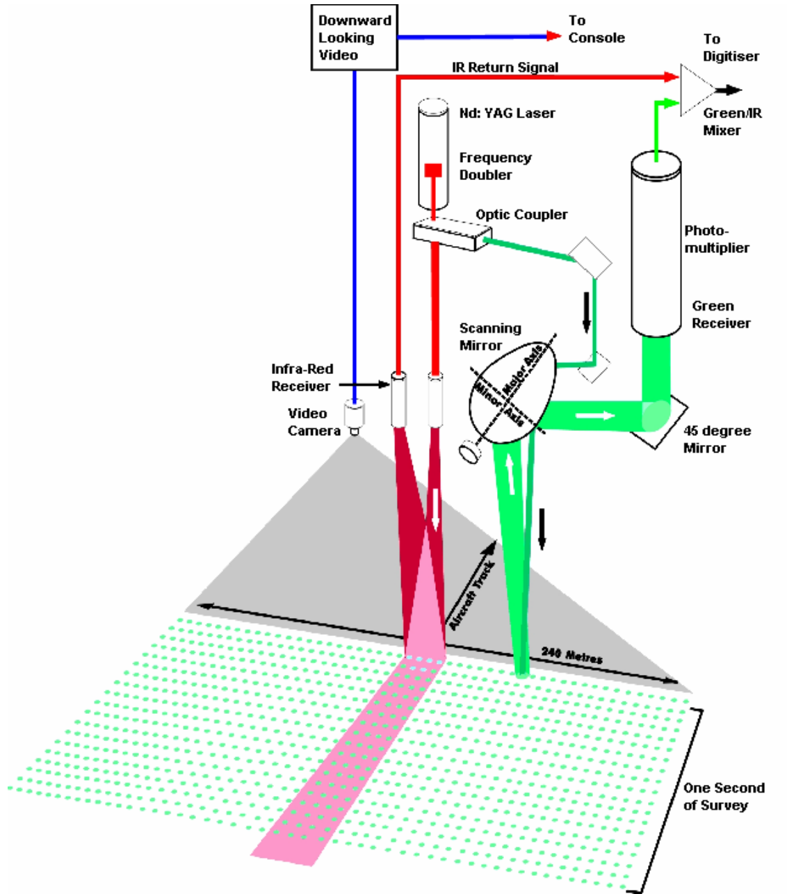
Figure 4 – The Airborne System Scanner, Laser and receivers
