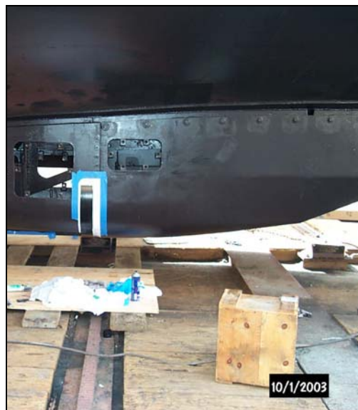
Figure 2: RESON SeaBat 8111ER MBES on FAIRWEATHER
