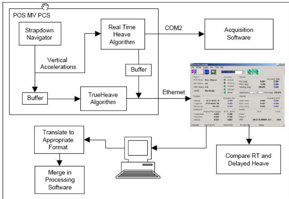
Figure 9: TrueHeave Functional Block diagram
