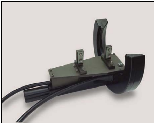
Figure 1: RESON SeaBat 8111ER MBES
