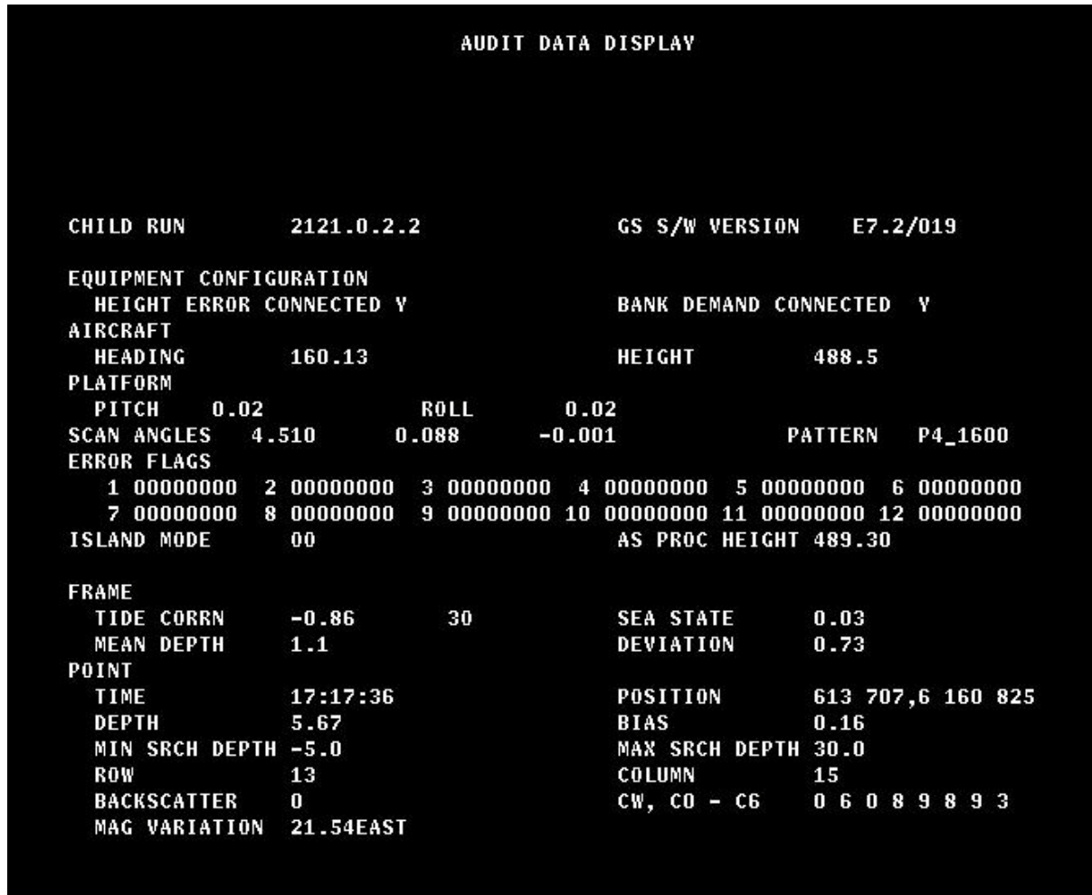
Figure 14 – Audit Display
