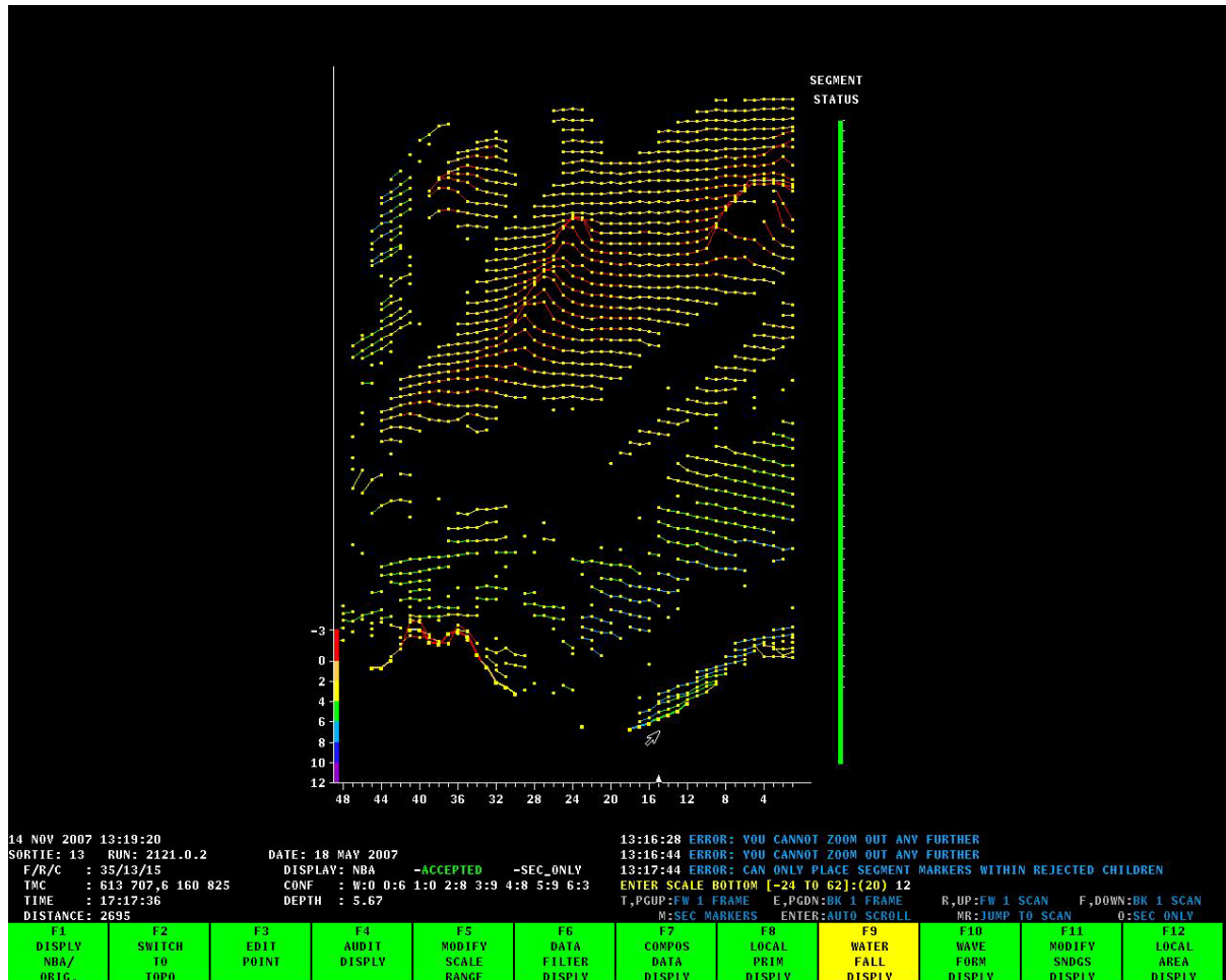
Figure 9 – Waterfall Display
