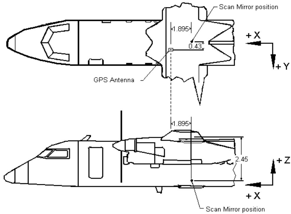
Figure 17 – Laybacks
