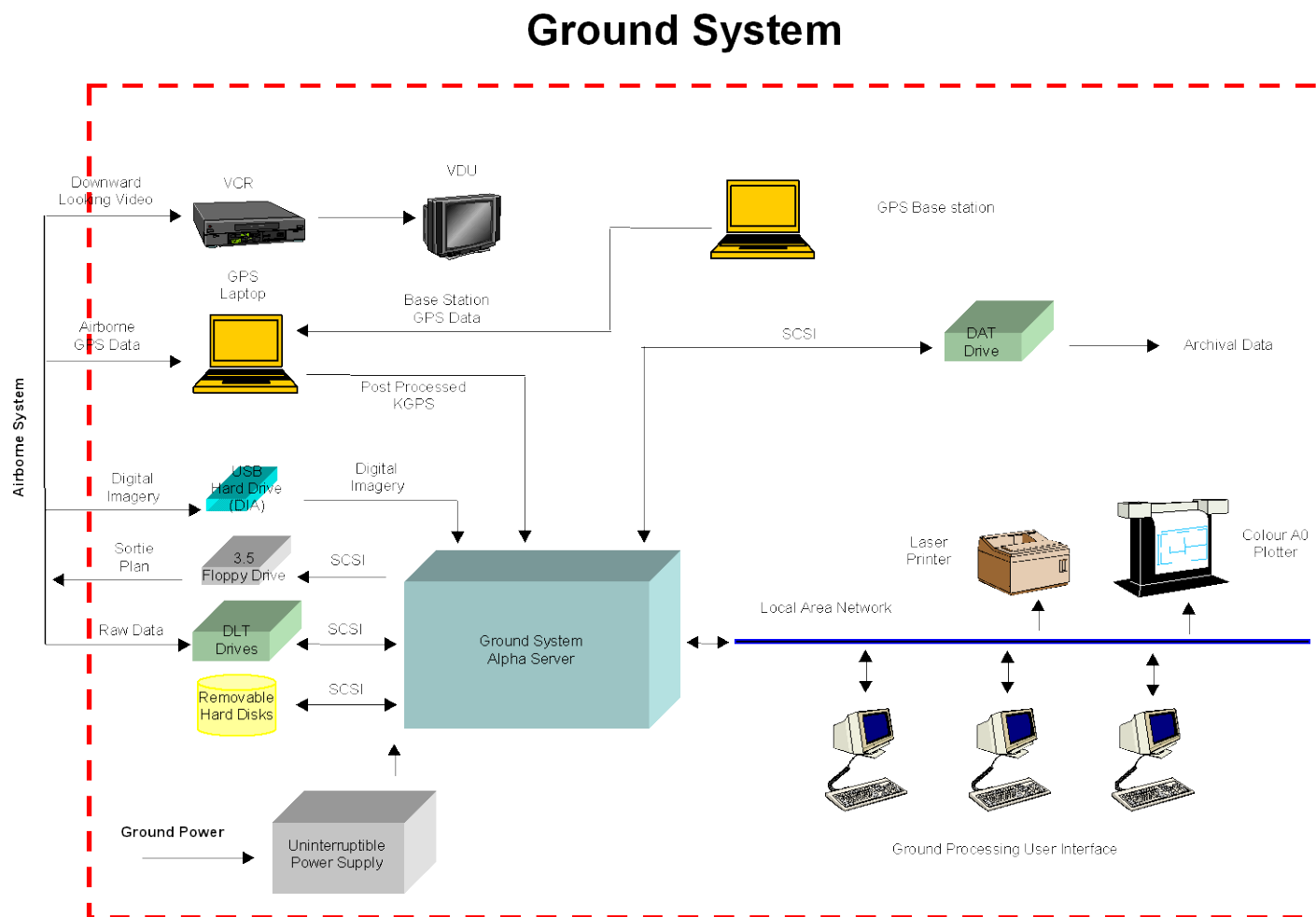
Figure 5 – Block Diagram of the LADS Mk II GS
