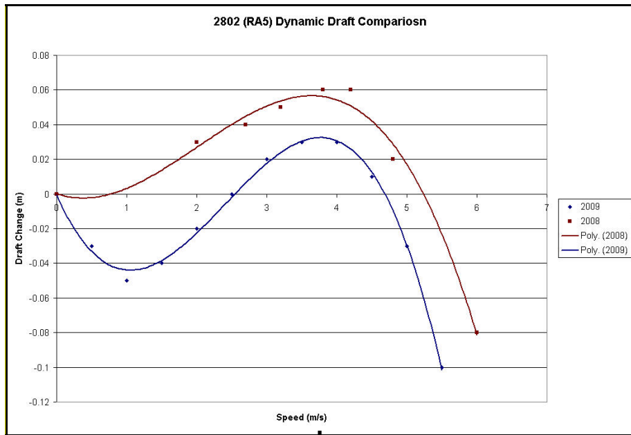
Figure 3: Dynamic Draft Curve Comparison
