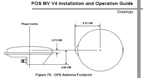
Figure 79: GPS Antenna Footprint
