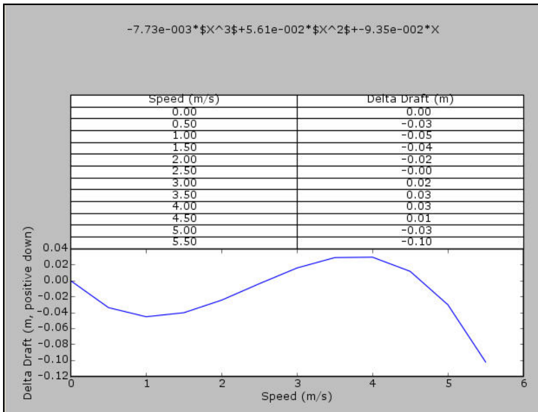
Figure 2: Dynamic Draft Curve and Values Table Generated using the ERDDM Method
