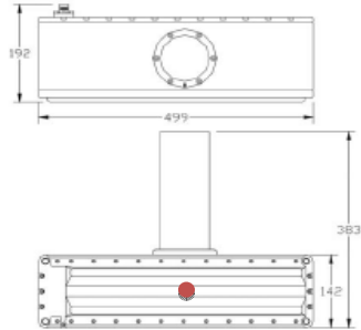
Figure 3 - Transducer array outline dimensions
