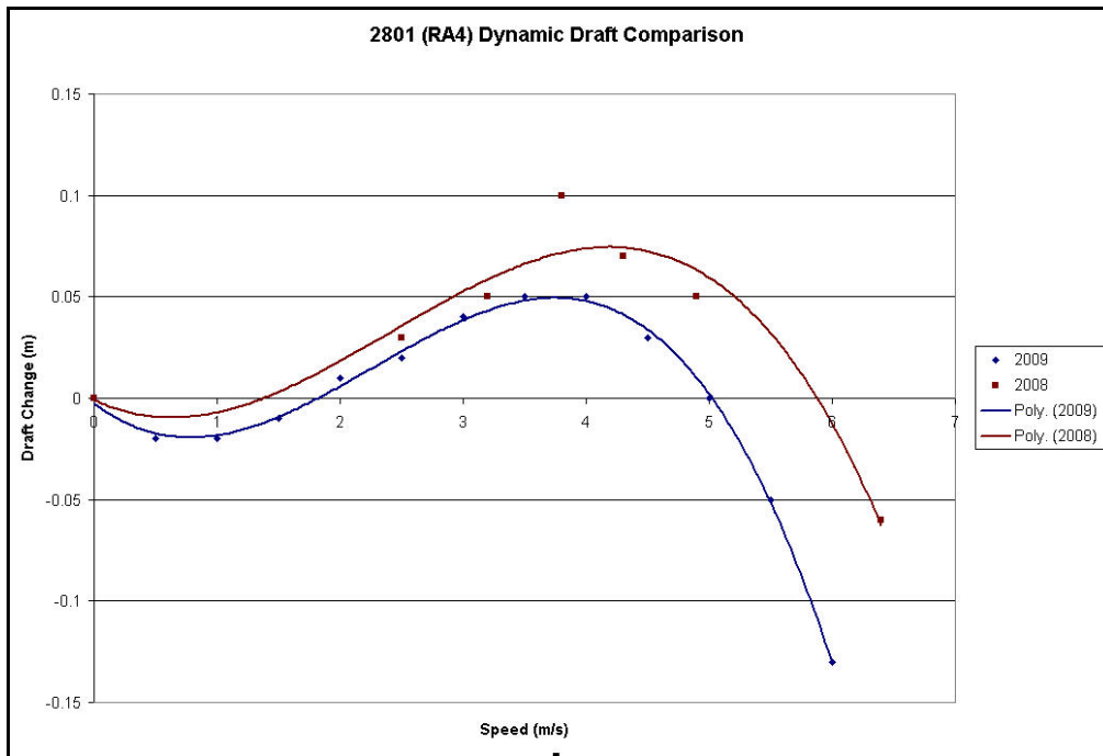
Figure 3: Dynamic Draft Curve Comparison
