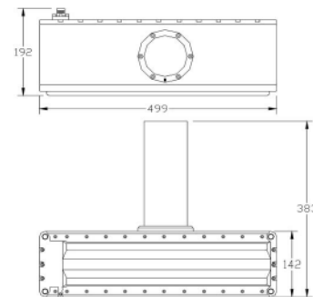
Figure 3: Sonar Head Dimensions
