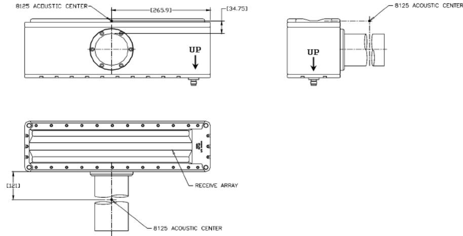
Figure 8: Sonar Head Acoustic Center
