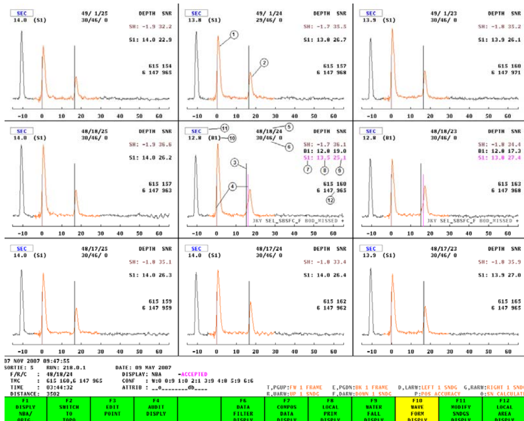
Figure 15 – Annotated Sounding Waveform Display
