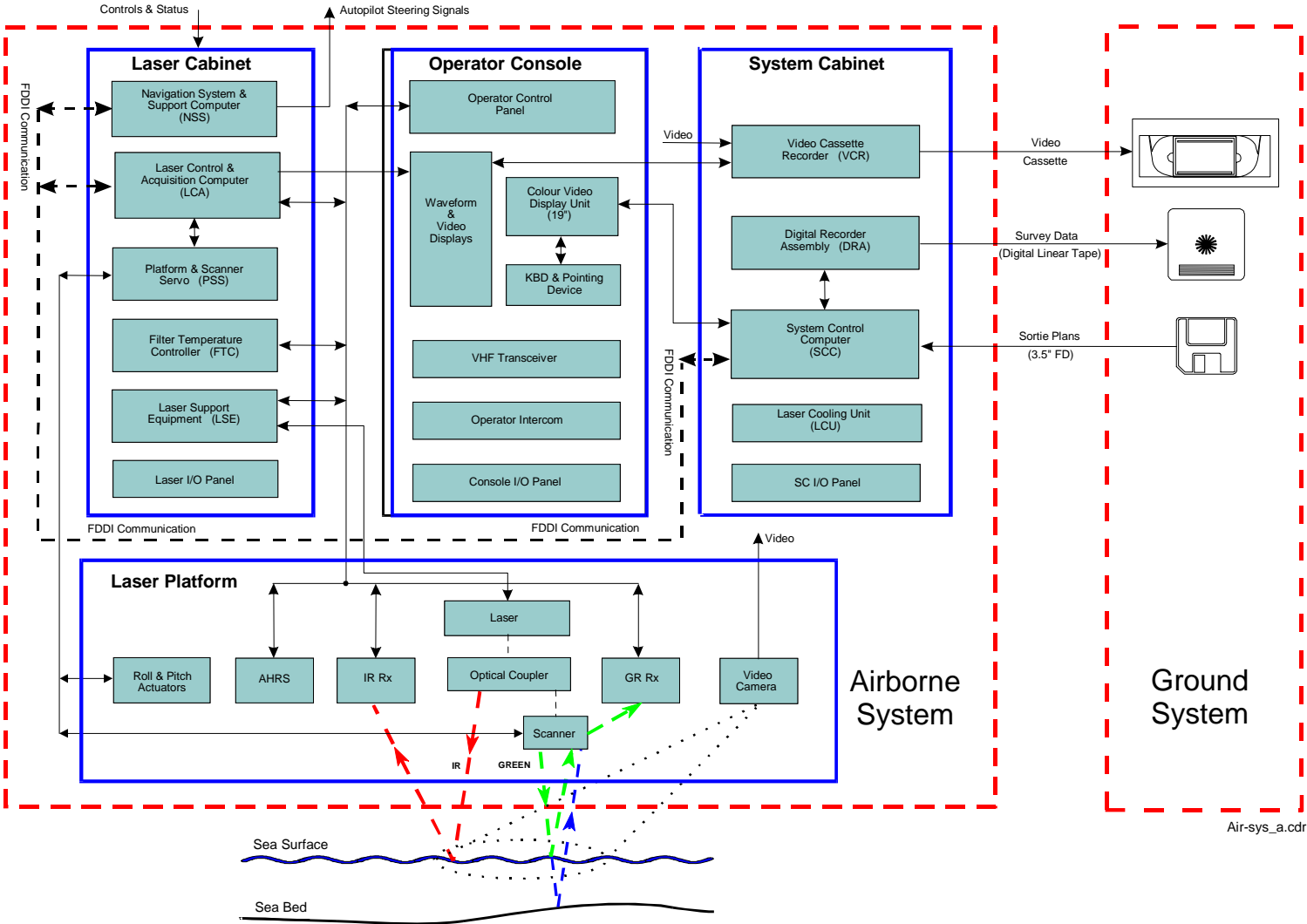
Figure 2 – AS Functional Block Diagram
