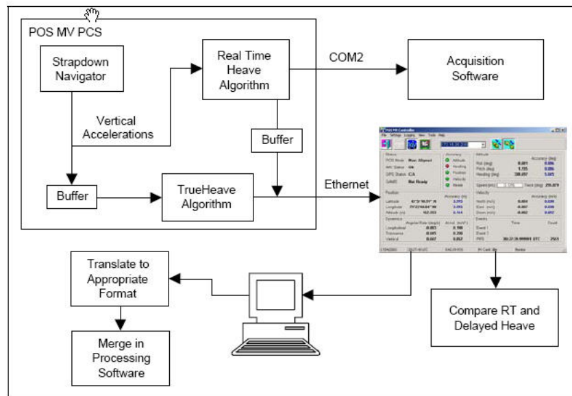
Figure 14: TrueHeave Functional Block diagram 1
