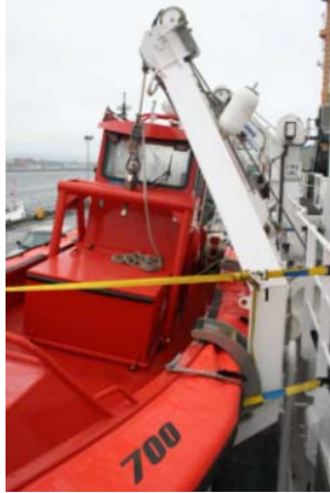
Figure 15: Vest Davit
