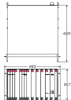
Transceiver
