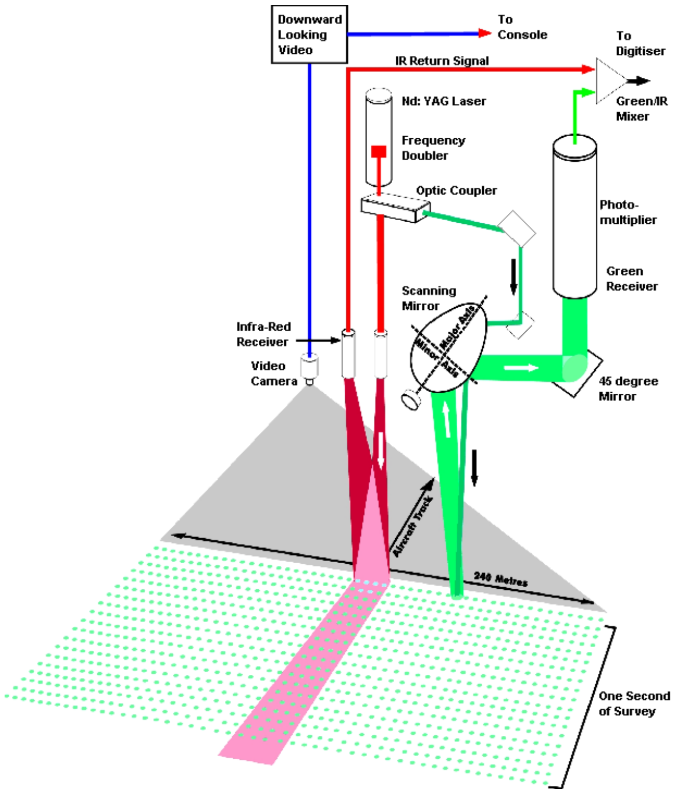
Figure 4 – The Airborne System Scanner, Laser and Receivers
