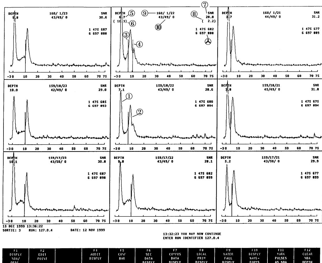
Figure 13 – Annotated Sounding Waveform Display
