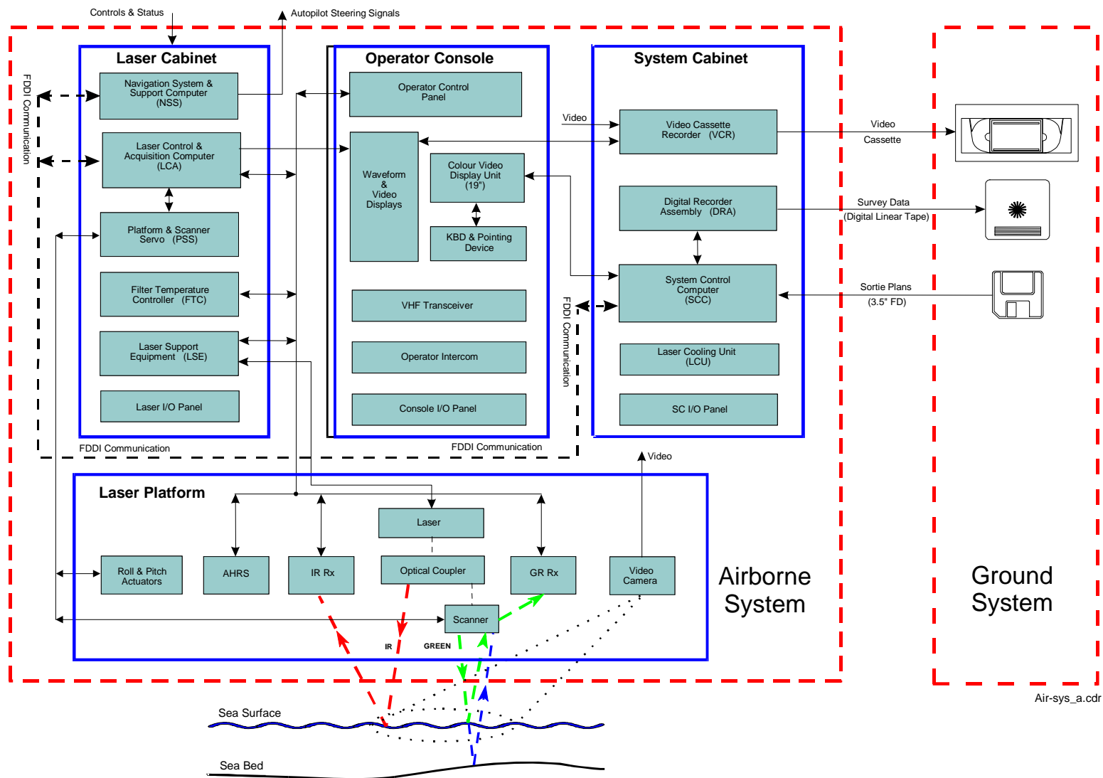
Figure 2 – Airborne System Functional Block Diagram
