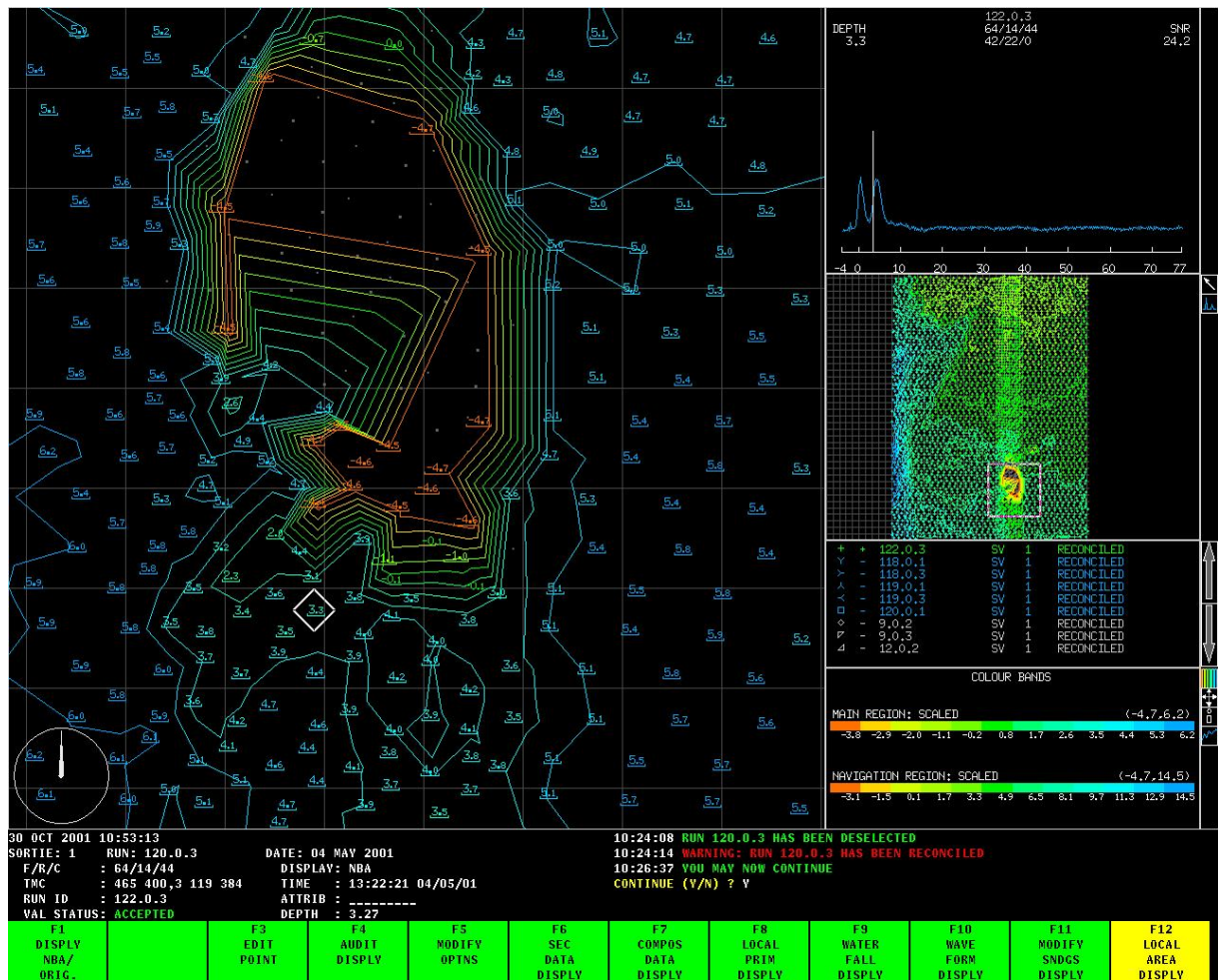
Figure 12 – Local Area Display – Medium Scale
