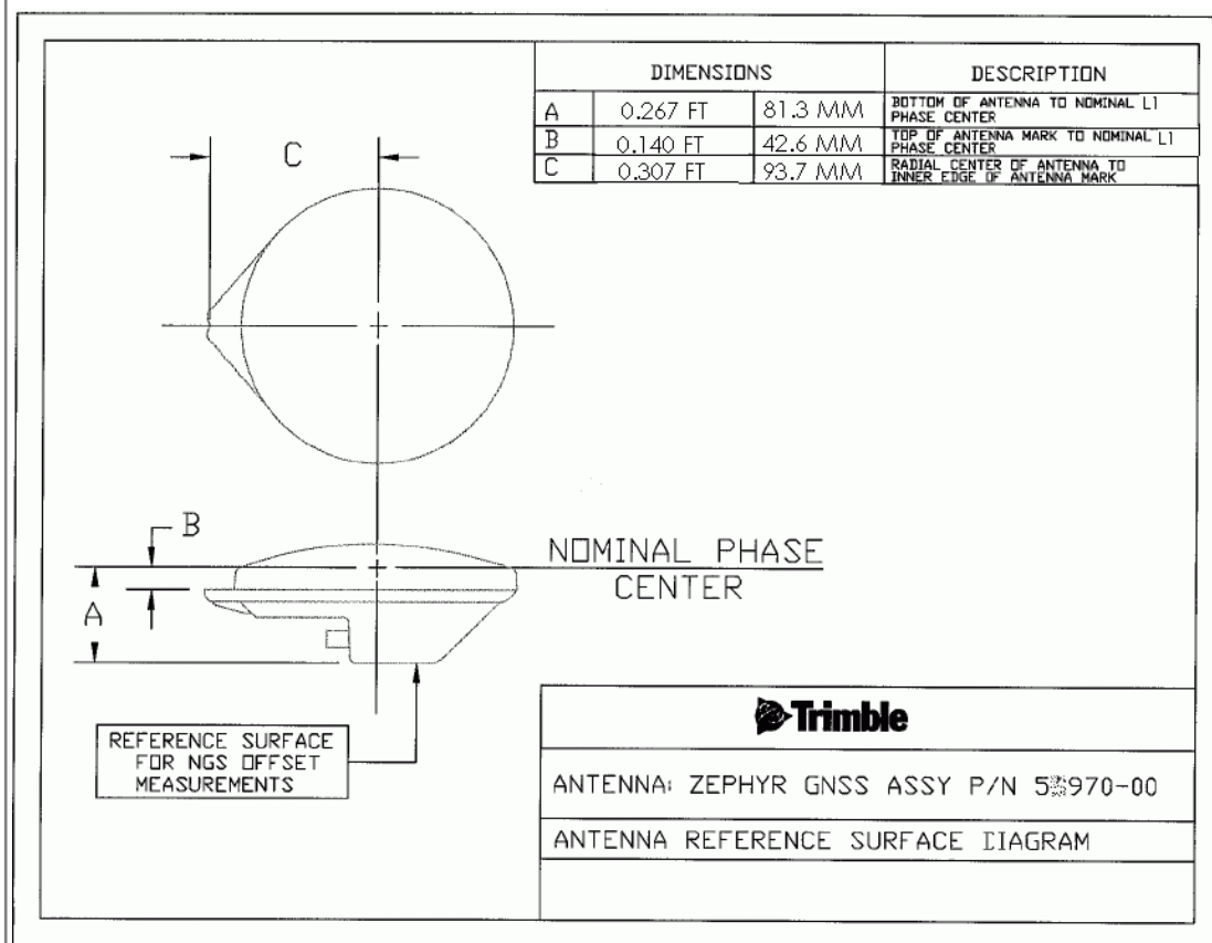
Figure 11: Zephyr II diagram
