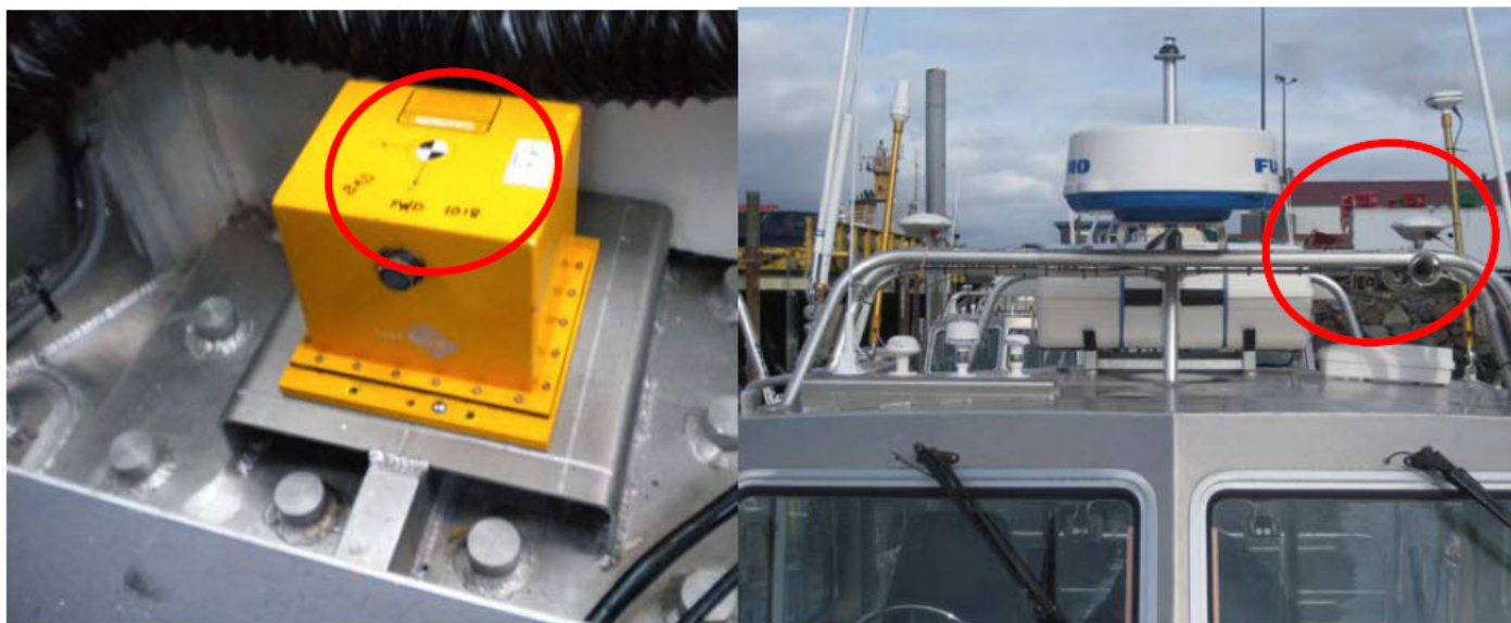
Figure 38: Vessel Reference Point (Top of POS MV IMU) & Primary GNSS Antenna (port side).
