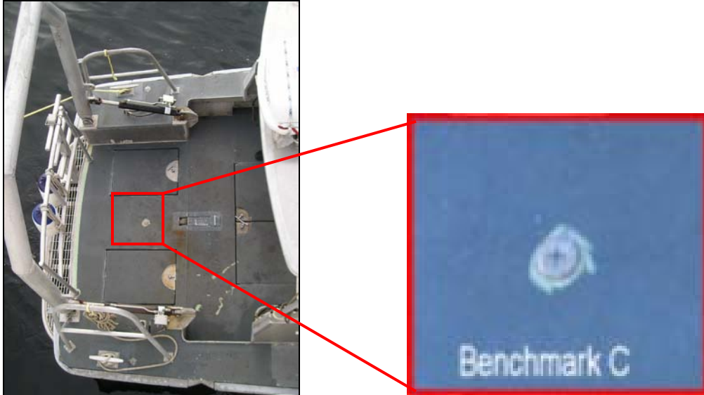
Figure 5: Permanent Control Point "Benchmark C" on launch 1018
