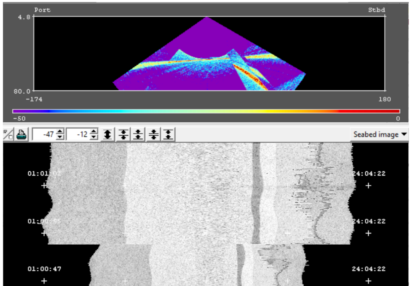
Figure 5: An example of the Kongsberg EM710 starboard beam dropout issue, as yet unexplained.
