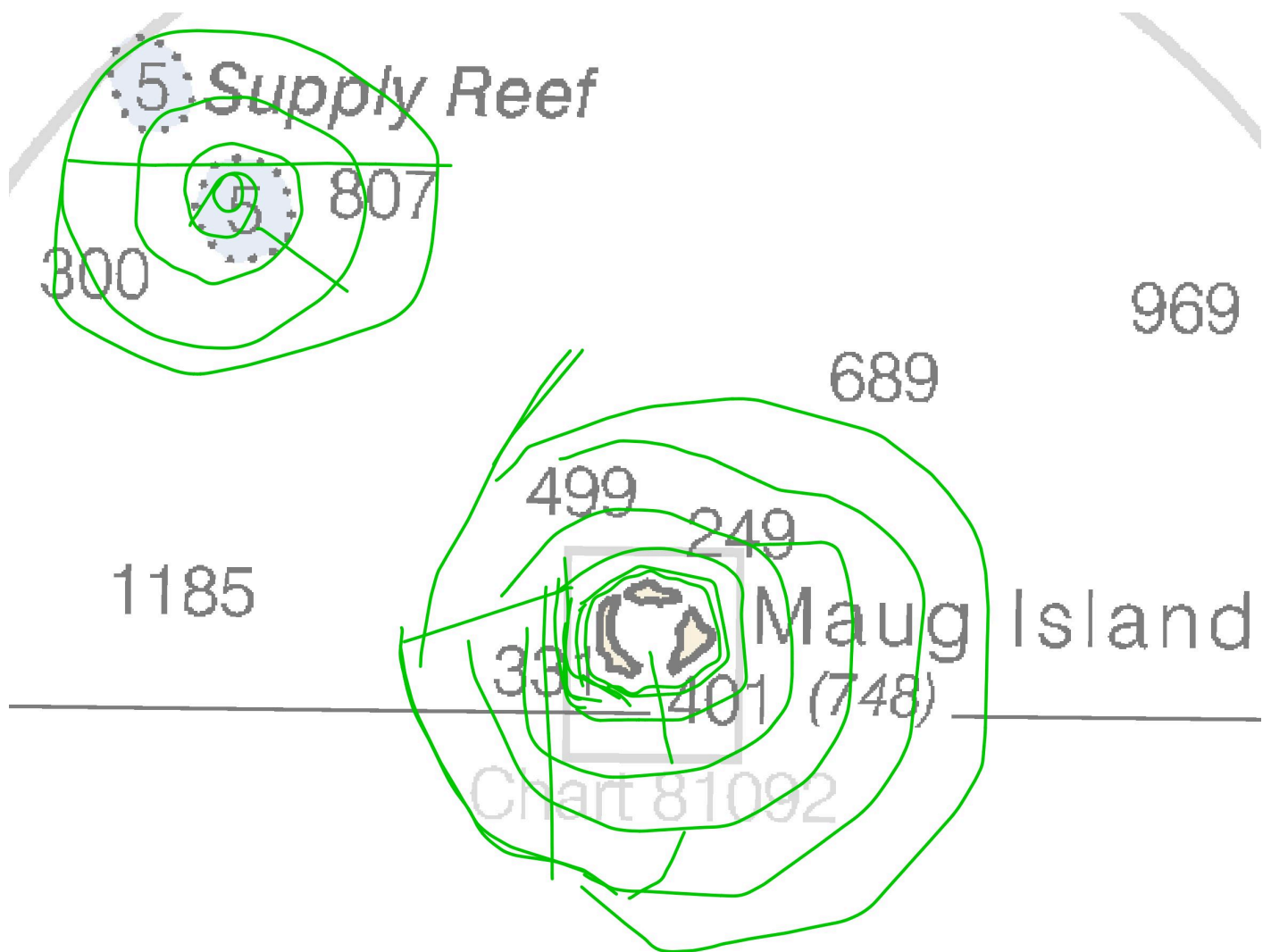
Figure 12: Examples of Rainier EM710 lines run around shoal areas in both concentric rings and an inward spiral "jellyroll" pattern.
