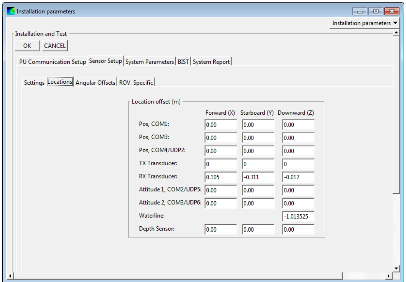
Figure 9: Offsets of Tx to Rx in SIS
