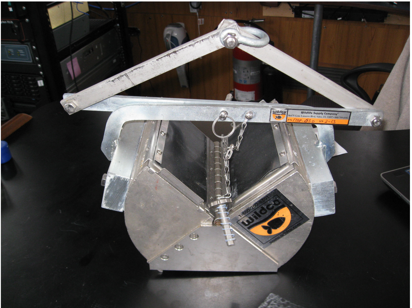
Figure 8: Petite Ponar Grabber
