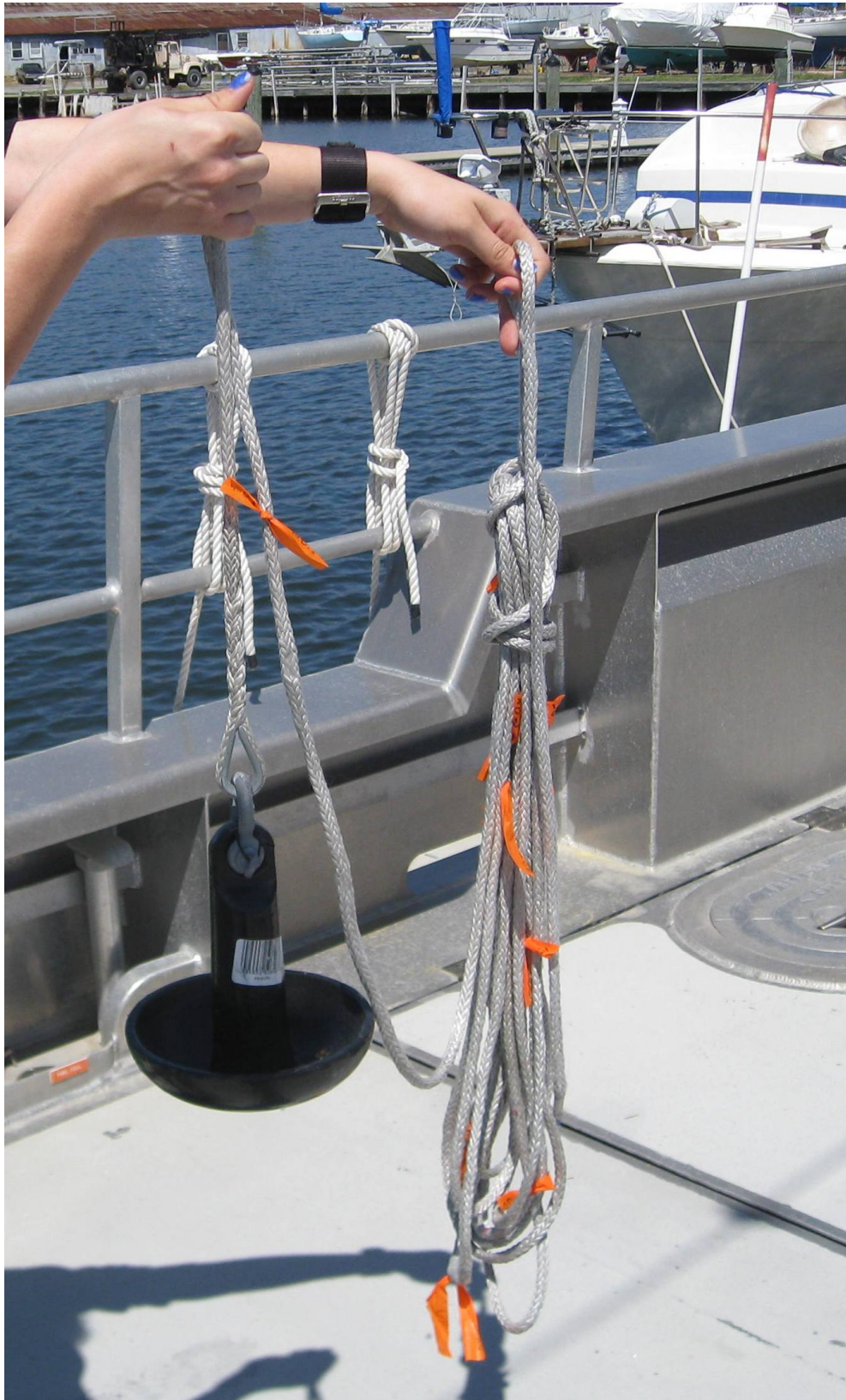
Figure 4: Bay Hydro II's non-traditional lead-line with orange meter incrementation.
