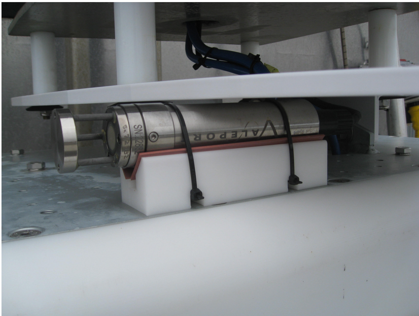
Figure 7: Valeport MiniSVS mounted to the MBES case.
