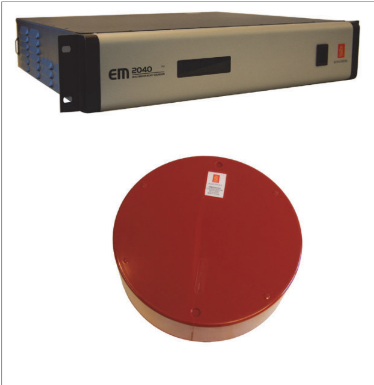
Figure 2: Kongsberg EM2040C
