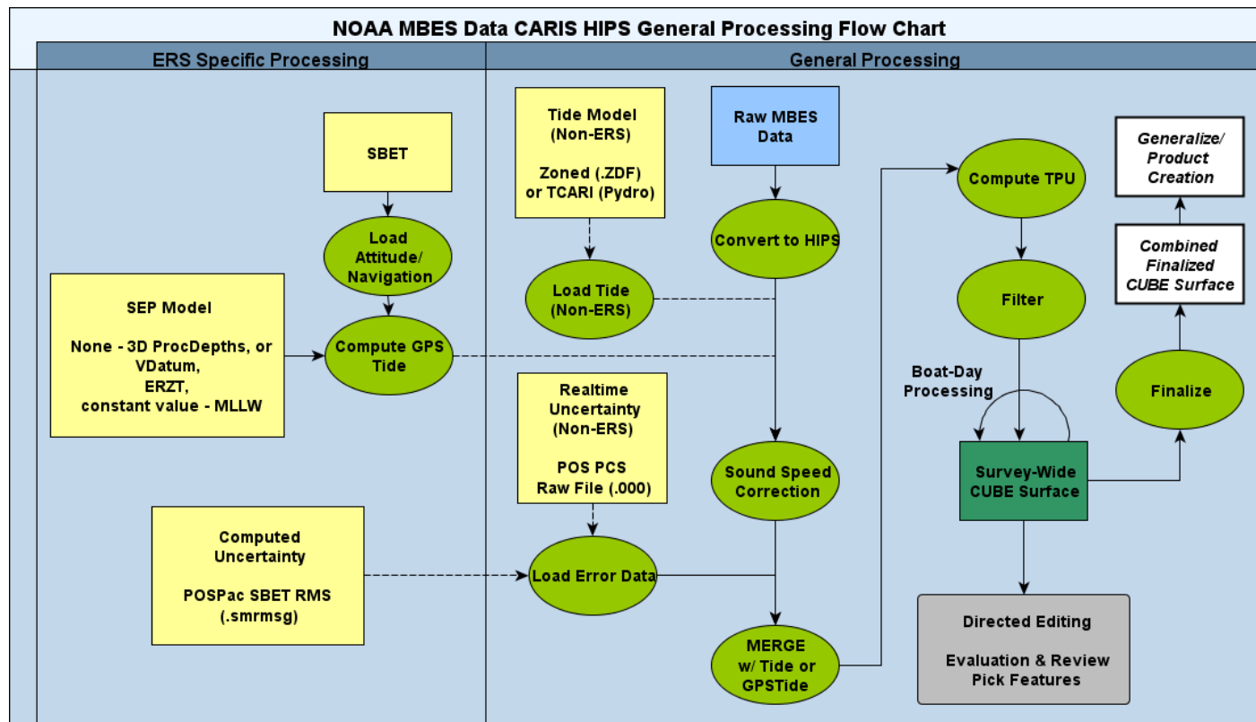
Figure 19: MBES Workflow
