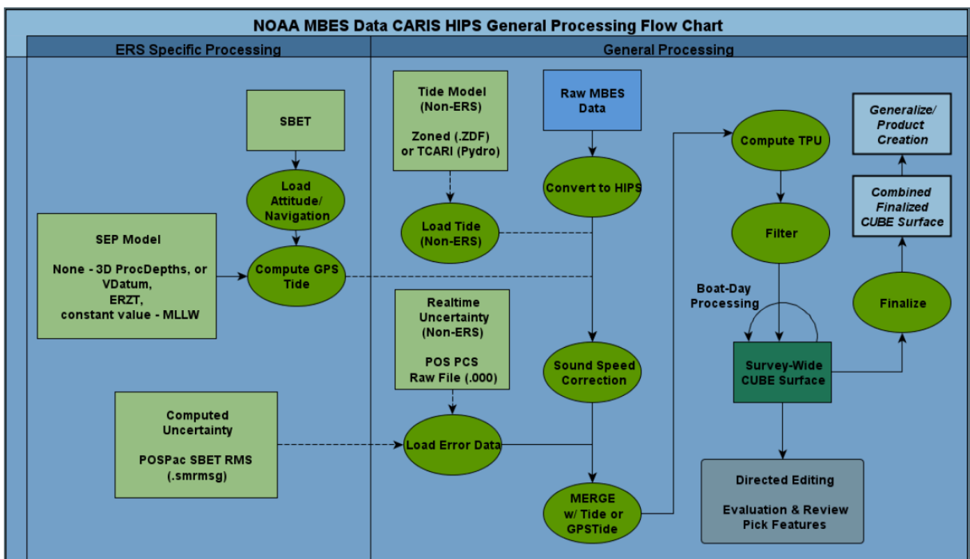
Figure 10: NRT4 MBES Workflow
