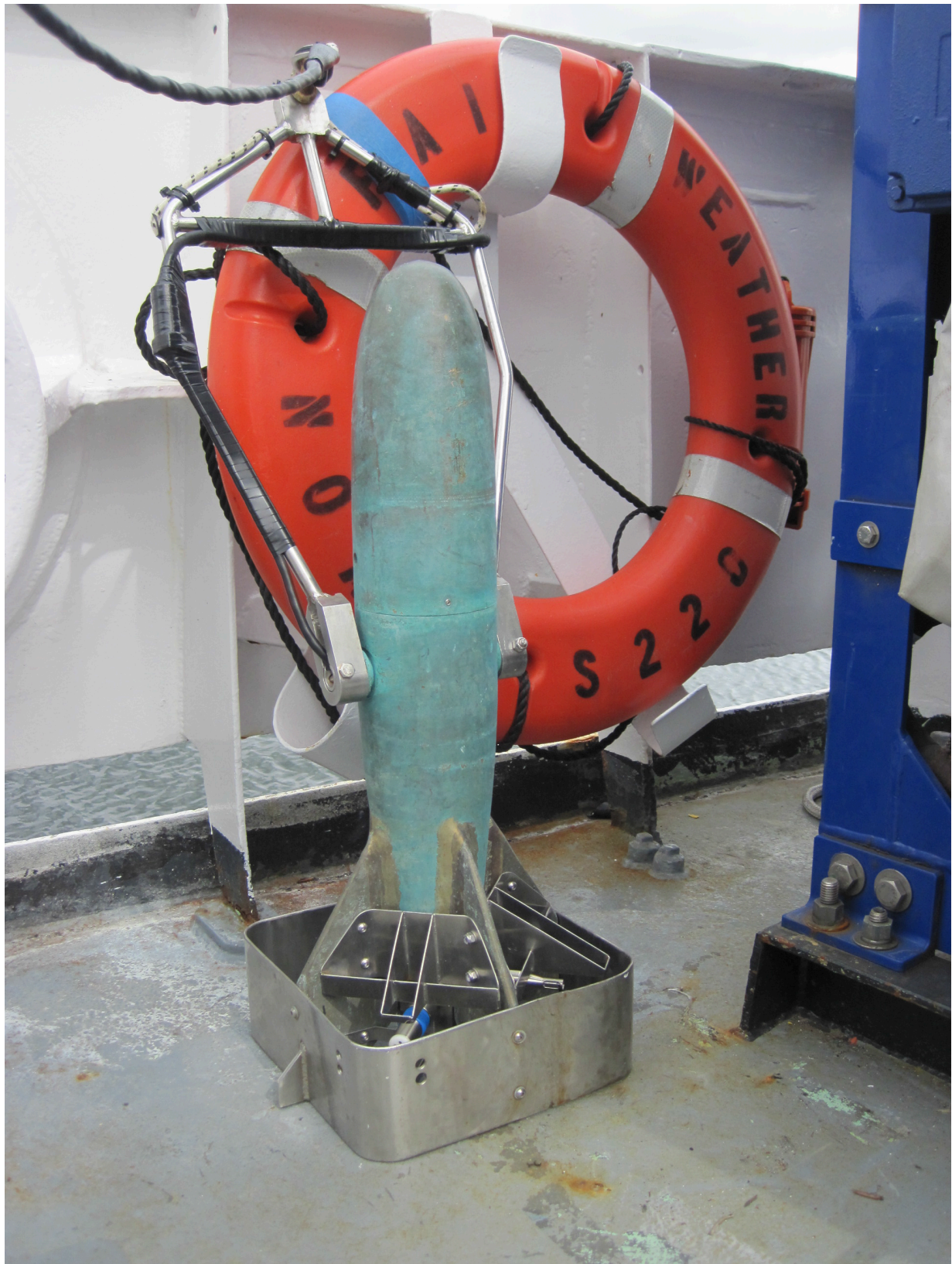
Figure 5: Single sensor free fall fish
