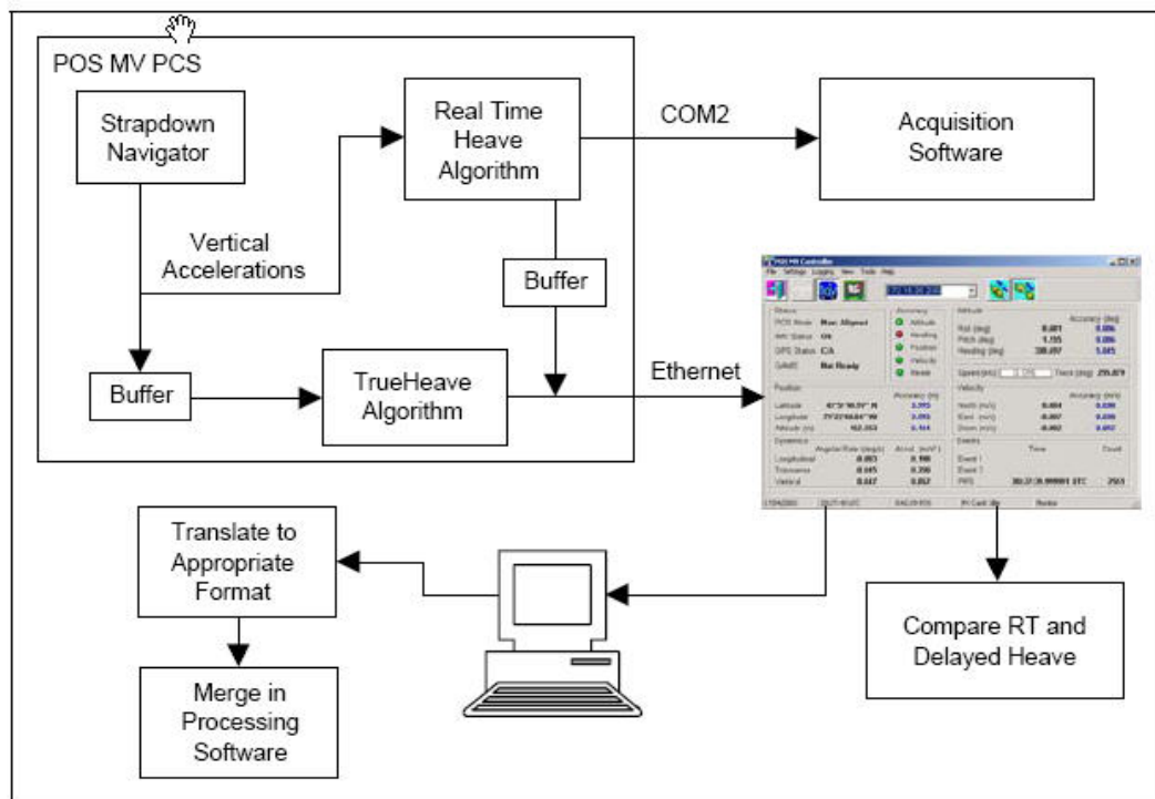
Figure 8: TrueHeave Functional Block diagram 1
