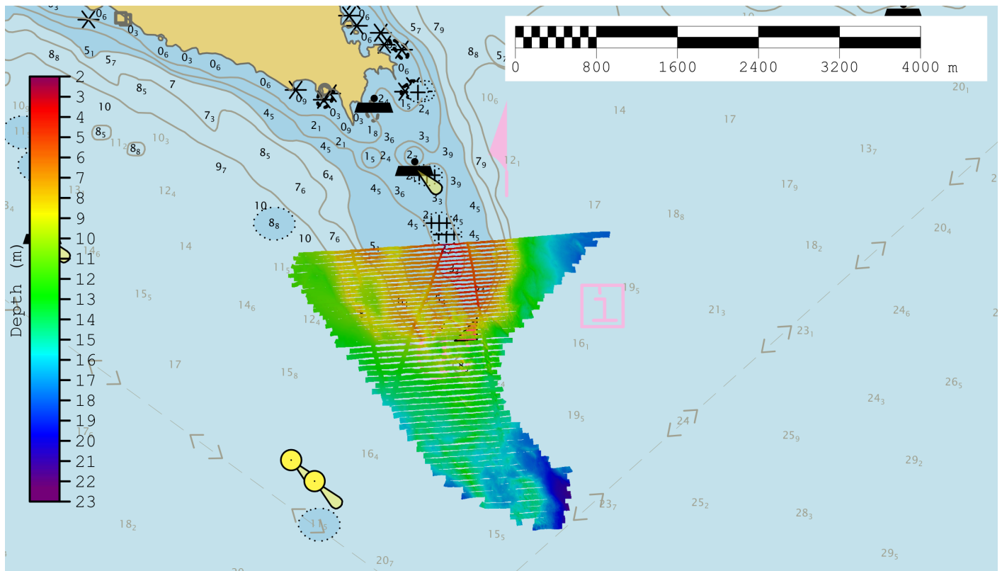
Figure 2: Survey MBES coverage overlaid on ENC US4MI66M.
