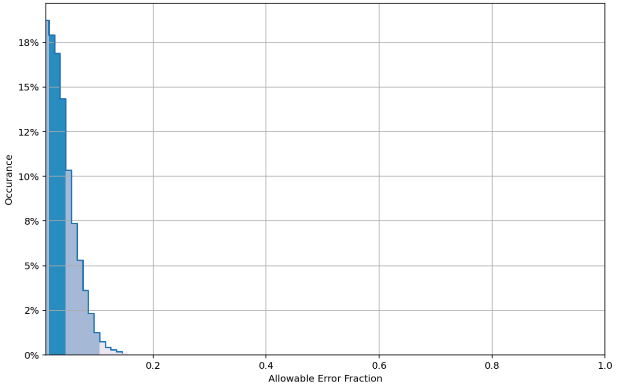
Figure 5: Pydro generated graph showing comparison between mainscheme and crosslines in F00862.
