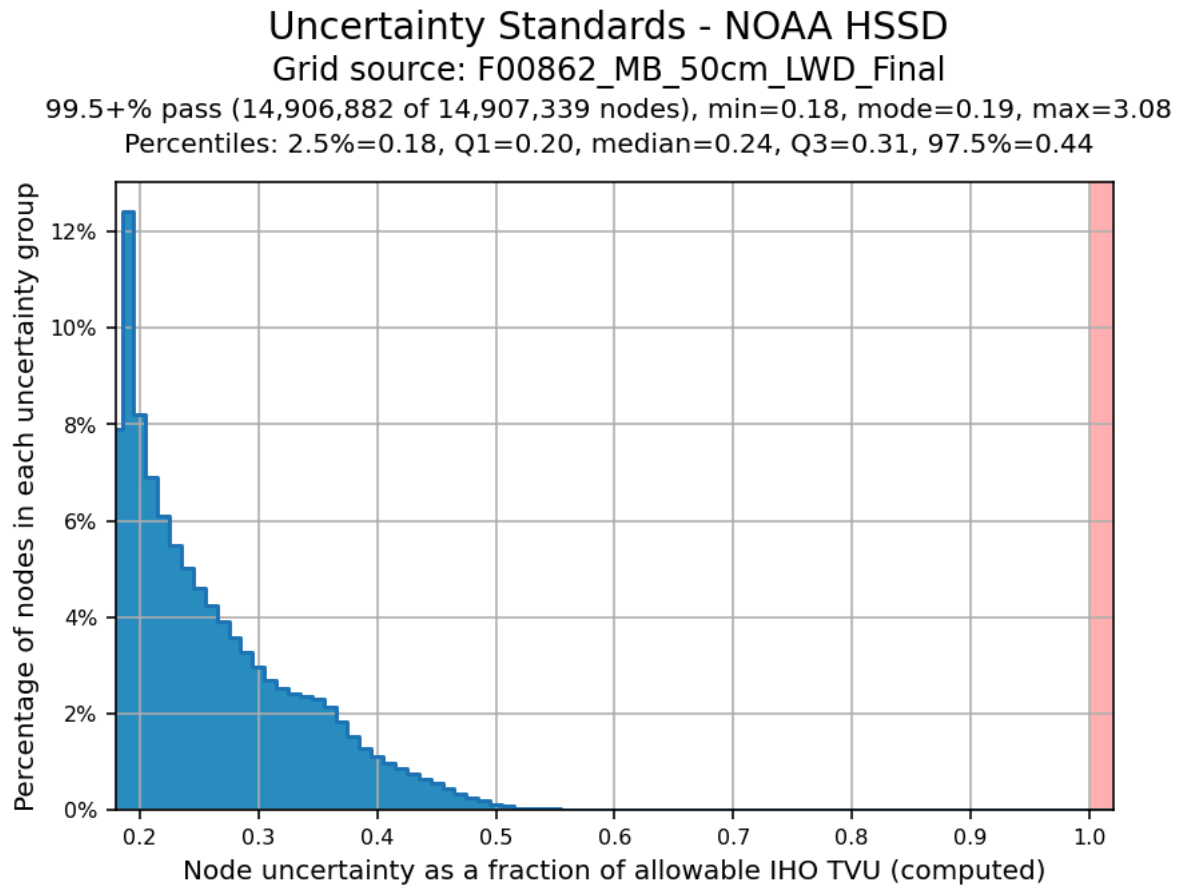
Figure 6: Pydro derived histogram plot showing HSSD Uncertainty Standards compliance of F00862 MBES data within the CUBE 50cm surface.
