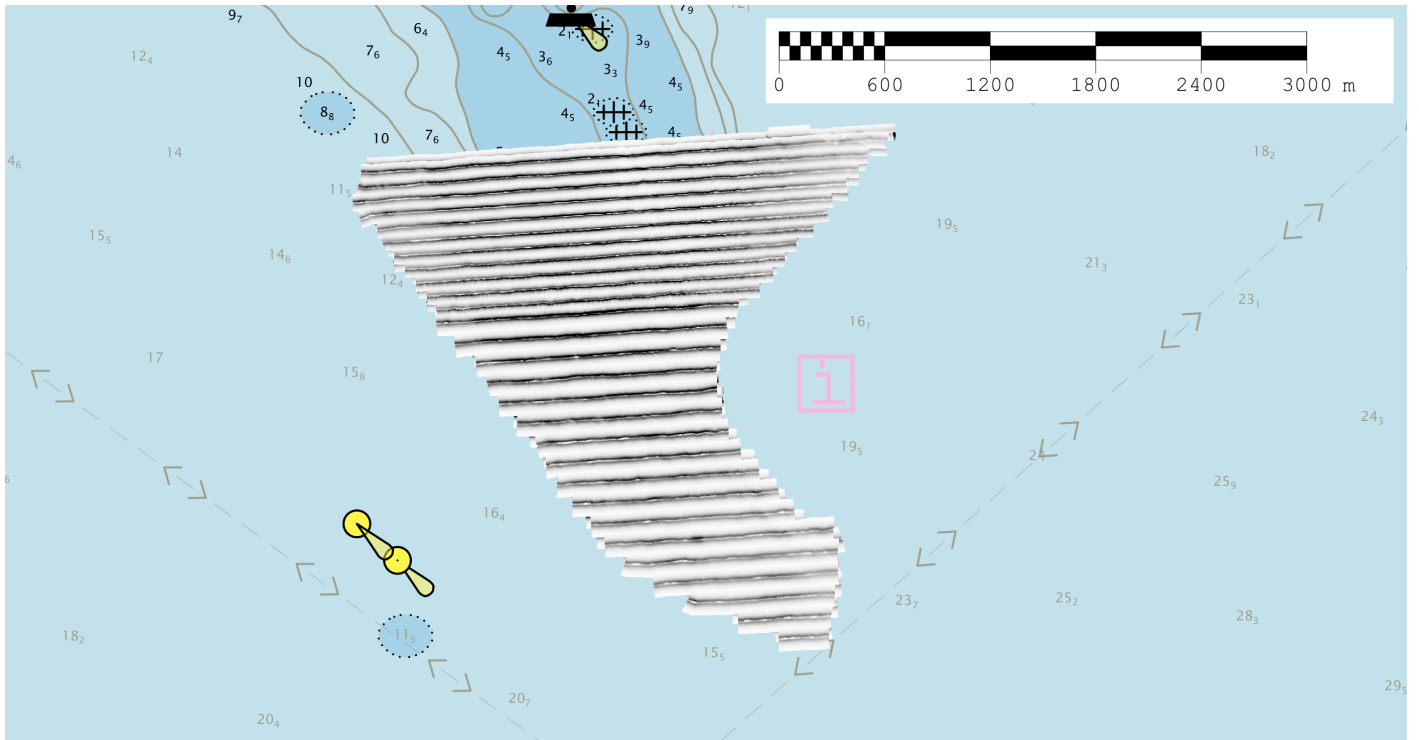
Figure 3: Survey 200% SSS coverage overlaid on ENC US4MI66M.
