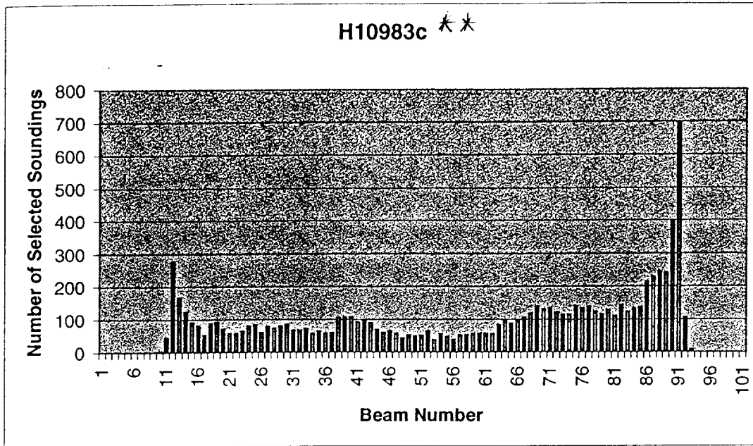
Figure R-1. Histogram of Selected Soundings by Beam Number – H10983c
