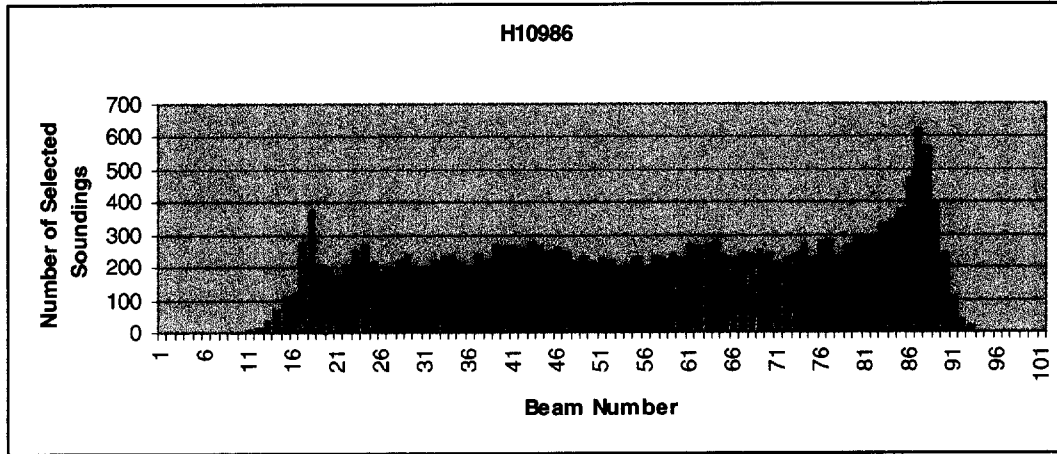
Figure R-1. Histogram of Selected Soundings by Beam Number – H10986
