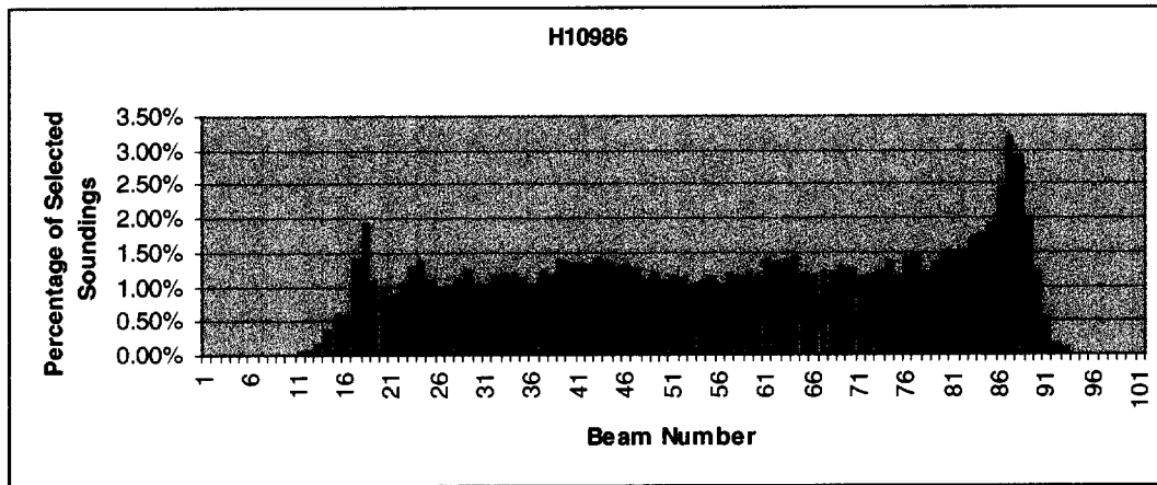
Figure R-2. Histogram of Percentage of Selected Soundings by Beam Number - H10986
