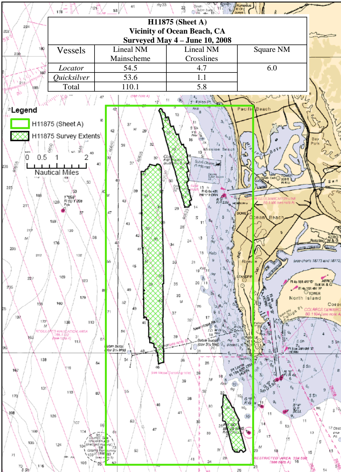
Figure 1 H11875 Area Surveyed
