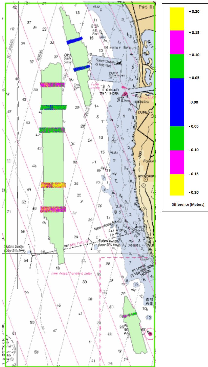
Figure 4 H11875 Difference Surface – Tidal minus GPSTide
