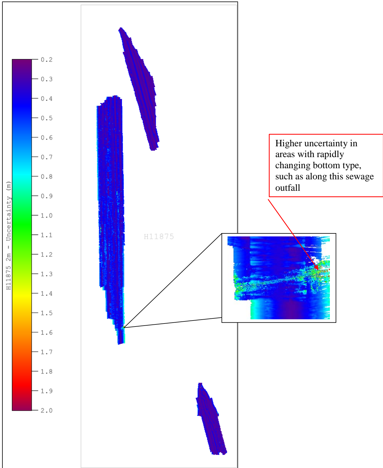
Figure 2 Uncertainty DTM
