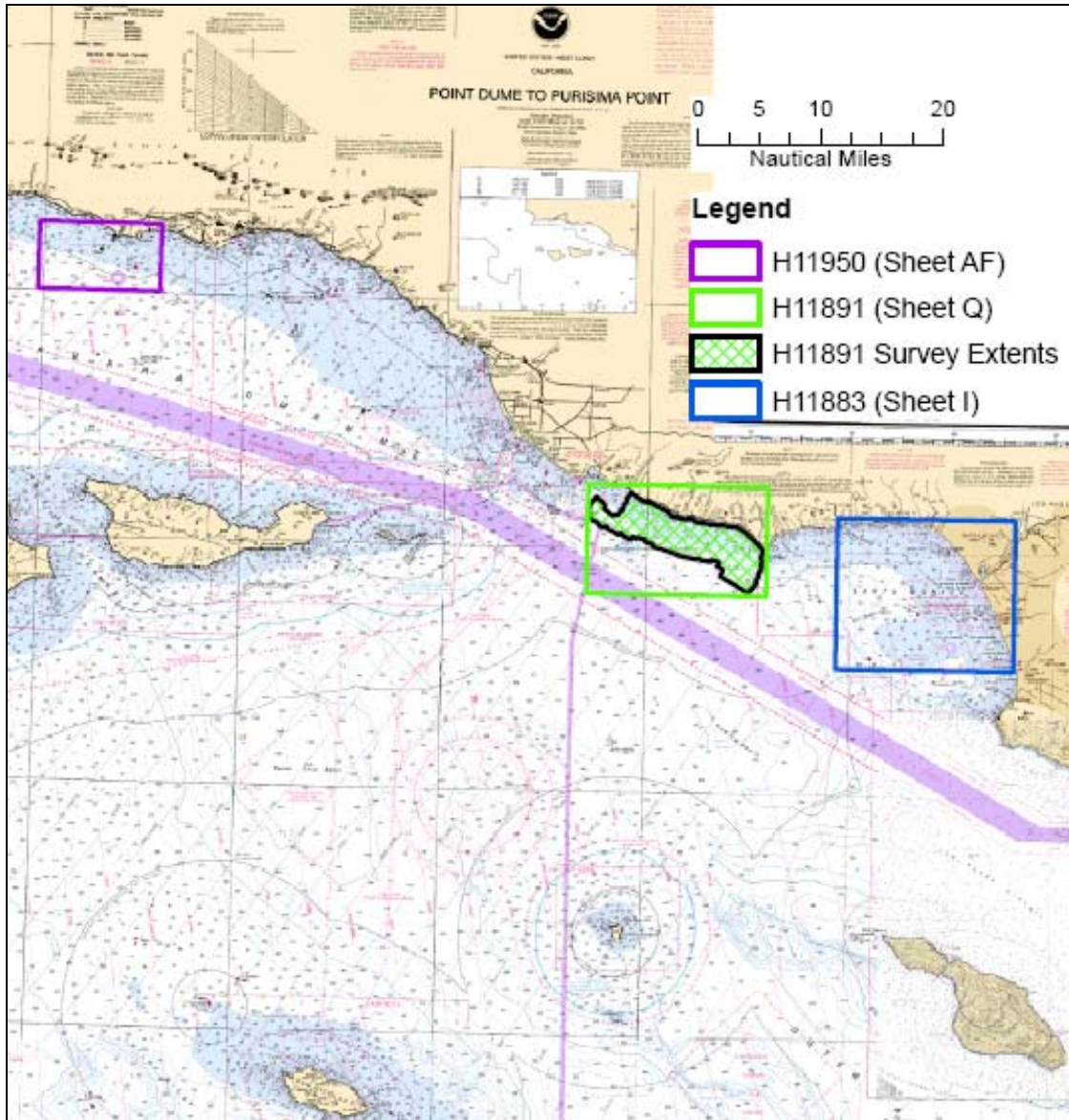
Figure 3 H11891 Survey Junctions
