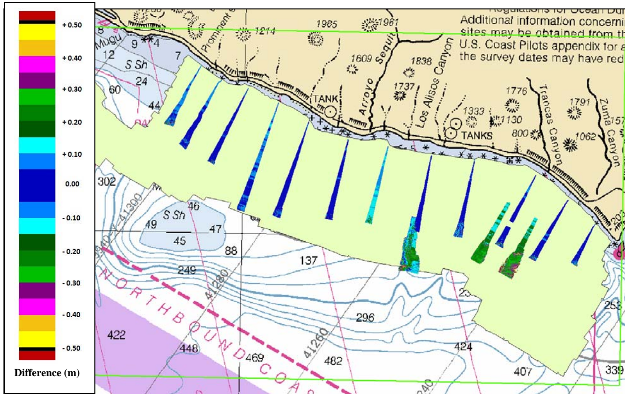
Figure 4 H11891 Difference Surface – Tidal minus GPSTide
