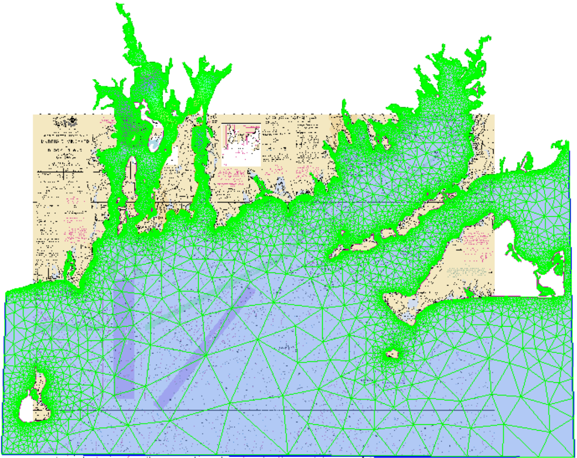
Figure B-8: Final Tide Zoning
