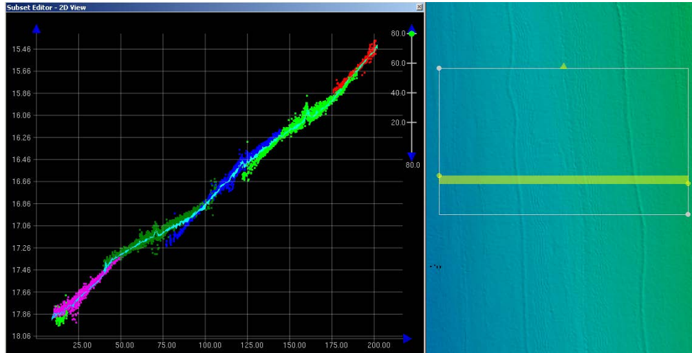
Figure 4 – Example from CARIS subset and BASE surface of multibeam lines showing along-track nadir artifact. Vertical grid size is 0.20 m.
