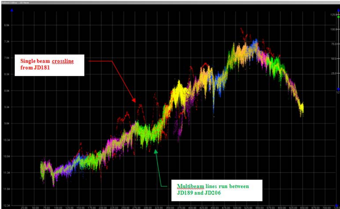
Figure 2 – Example from CARIS subset of a SBES vs MBES crossline comparison that fails due to bottom change. The crossline (single beam 3B-02-SB02470a shown in red) differs from the multibeam
