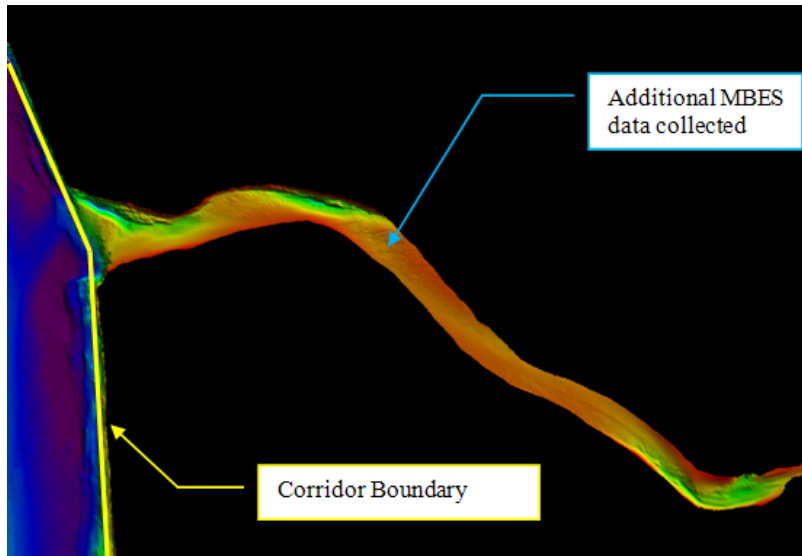
Figure 10 – Additional data collected in channel outside of the MBES corridor.
