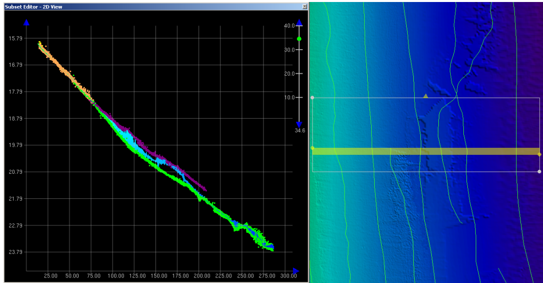
Figure 5 – Example from CARIS subset and BASE surface of lines in H12165 showing up to 0.50 m of bottom change over a 16 day period. Purple lines are Julian day 206 infills. Green and orange lines were run on Julian days 189 and 190. BASE surface shown in light blue. Vertical scale is 1 meter.
