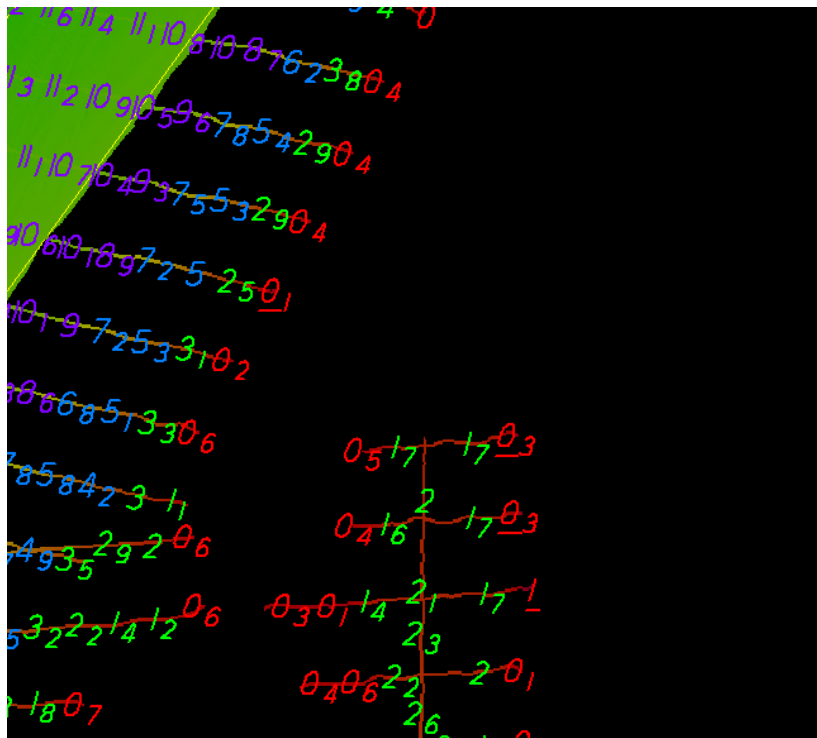
Figure 9 – SBES soundings do not achieve 1 meter. Area deemed navigationally insignificant. Soundings 1 meter or shallower shown in red. See correspondence in Appendix V.
