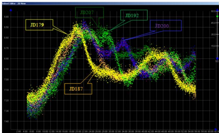
Figure 7 – Example from CARIS subset of JD179 to JD207 echosounder comparisons. Lines are colored by day. Matchup is poor – sand waves shift up to 4 meters, causing up to 0.50 meters of vertical shift. Vertical grid spacing is 0.10 m.
