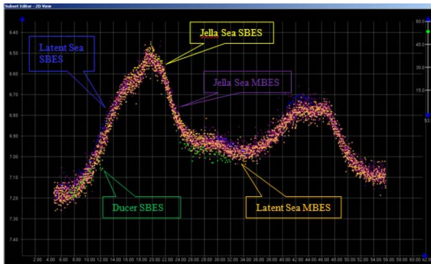
Figure 8 – Example from CARIS subset of JD179 echosounder comparison data only, same area as above figure. Lines are colored by vessel, and consist of the three single-beam echosounders and two multibeam sonars, showing good agreement. Vertical grid spacing is 0.10 m.
