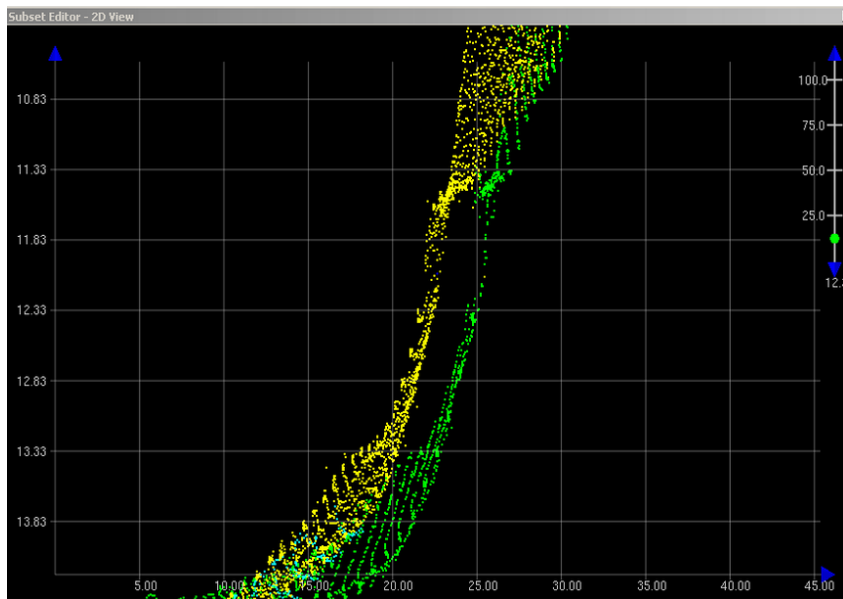
Figure 6 – Example from CARIS subset of lines in H12165 showing up to 2.0 m of vertical and 3 m of horizontal bottom change over a 15 day period. Green line is an infill from Julian day 206, the yellow line was collected on Julian day 191. Vertical scale is 0.5 meter.
