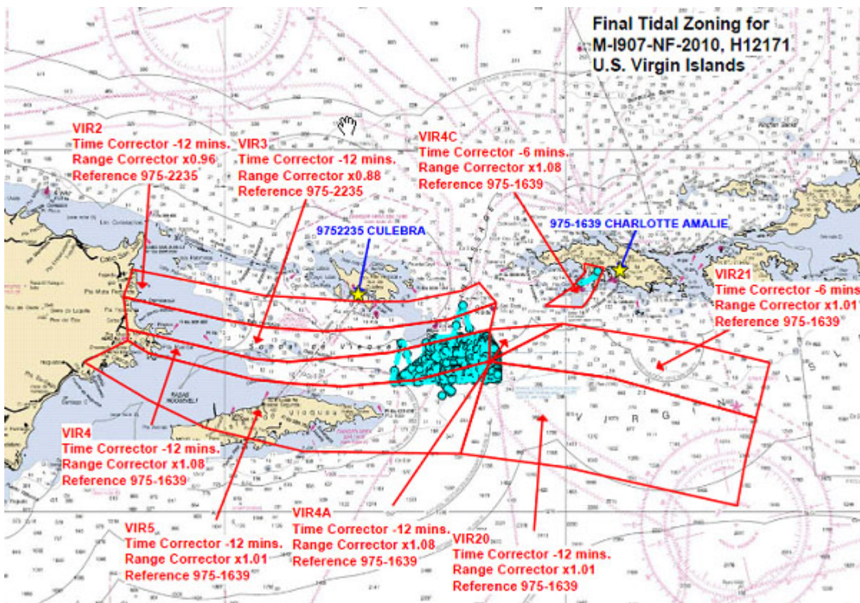
Fig3. Final Tide Zoning H12171
