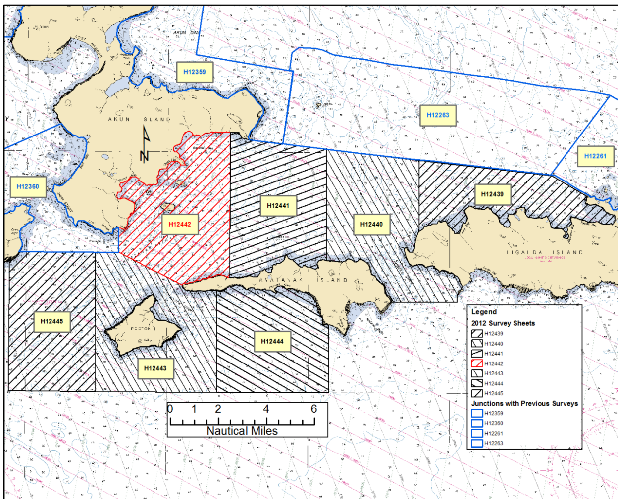
Figure 7 H12442 Survey Junctions
