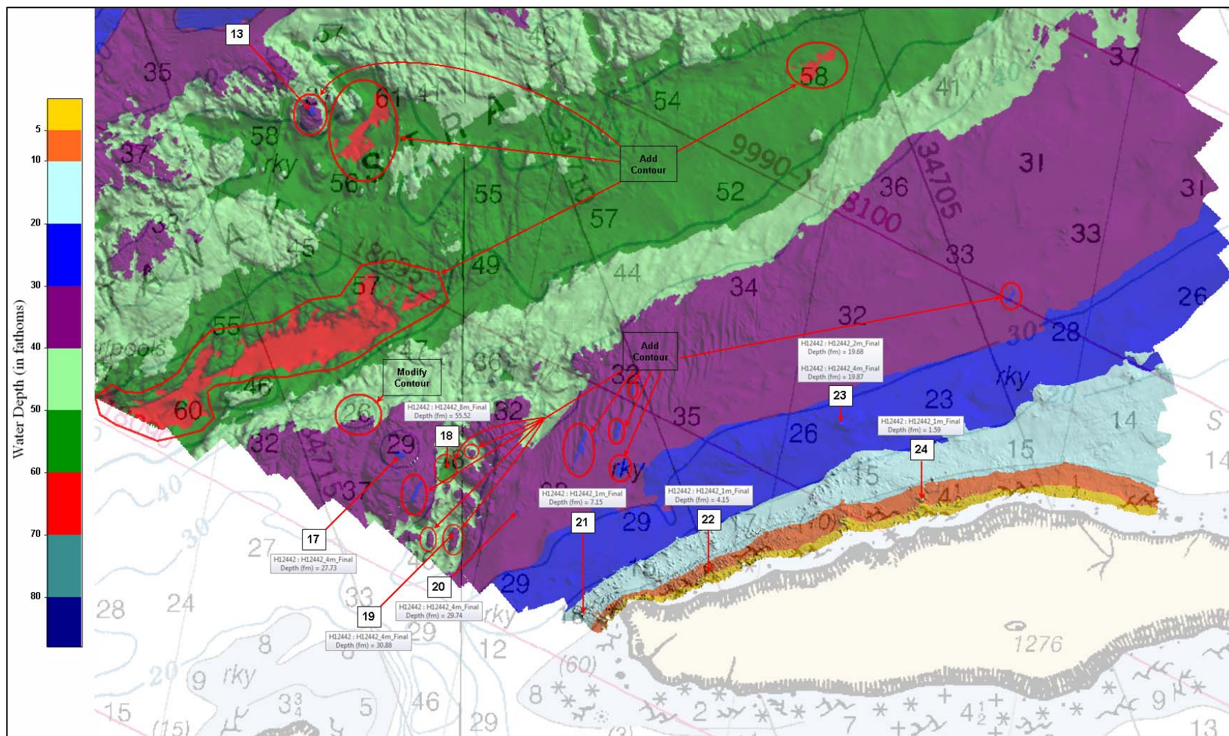
Figure 10 Contours and Charted Soundings to be Modified in the ENC and RNC
