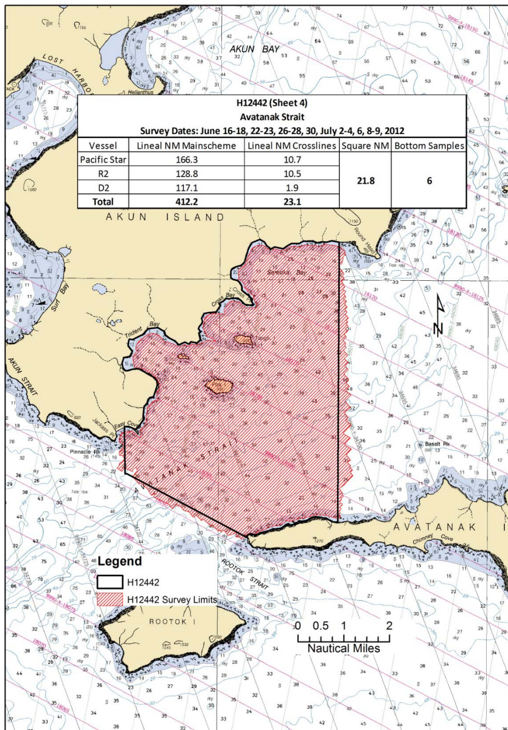
Figure 1 H12442 Area Surveyed
