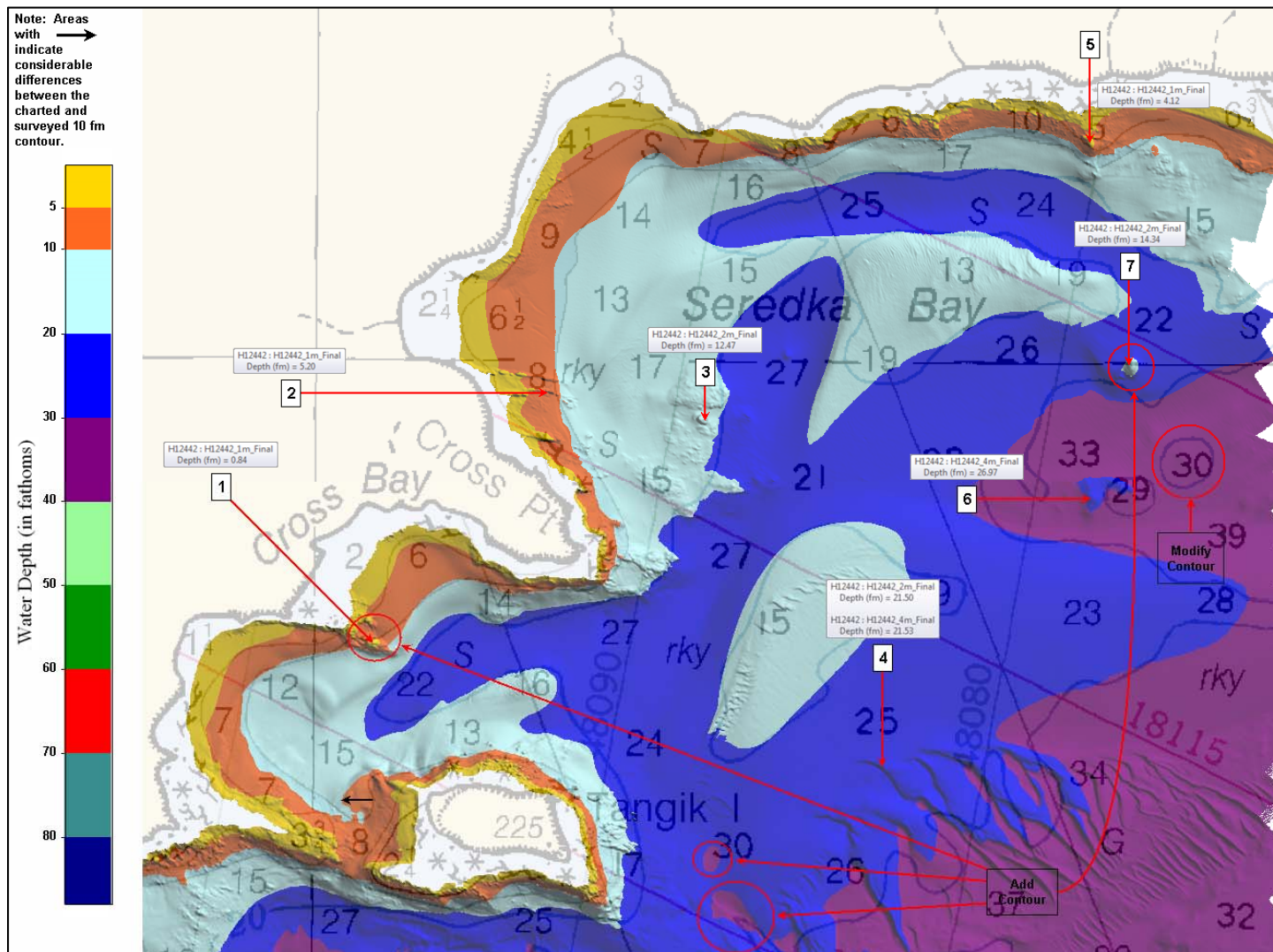
Figure 8 Contours and Charted Soundings to be Modified in the ENC and RNC
