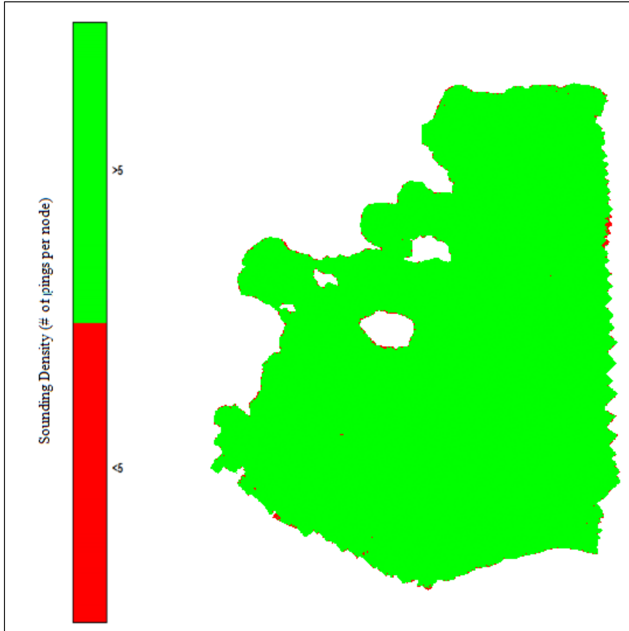
Figure 5 Density DTM
