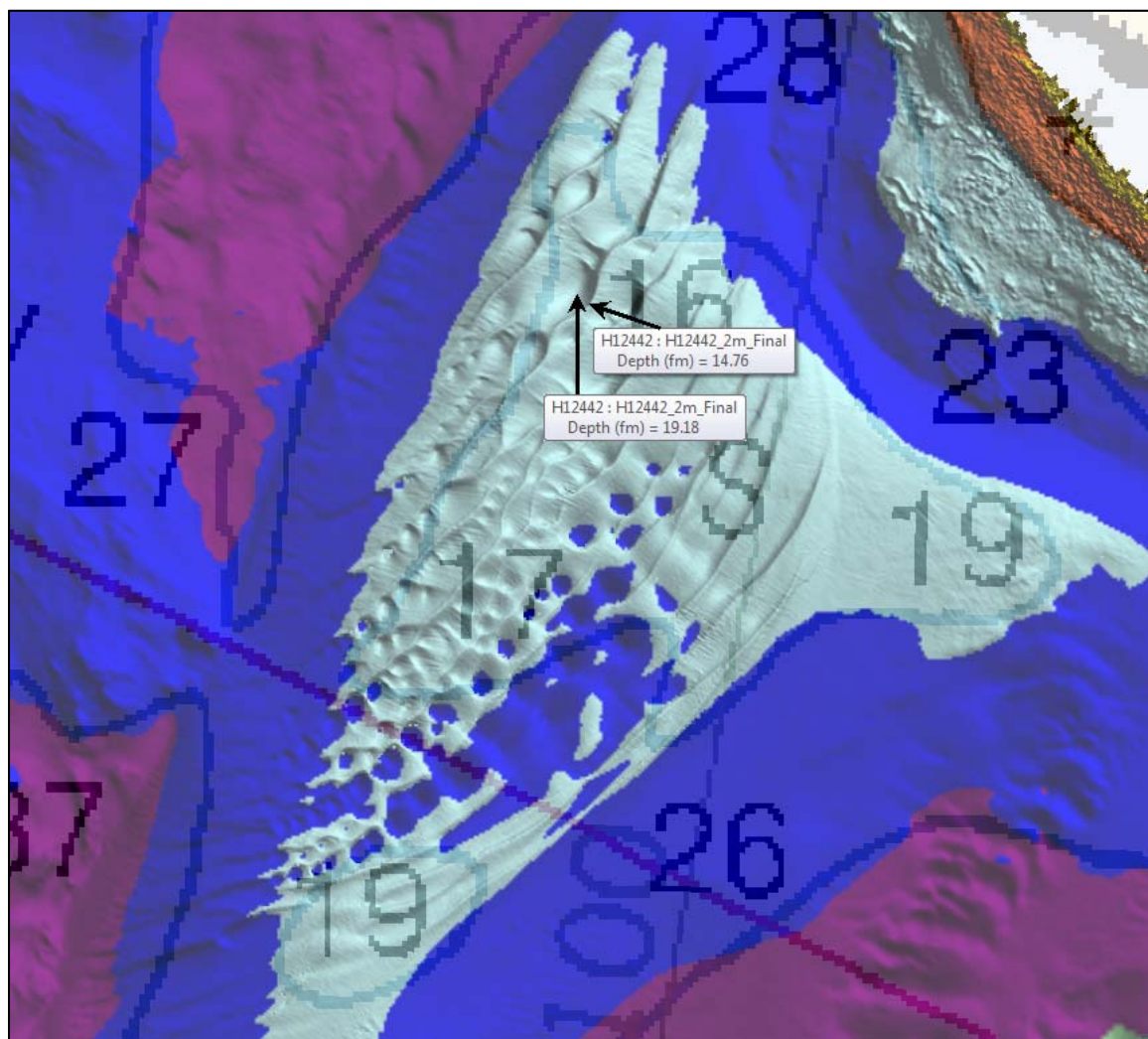
Figure 16 Sand Waves
