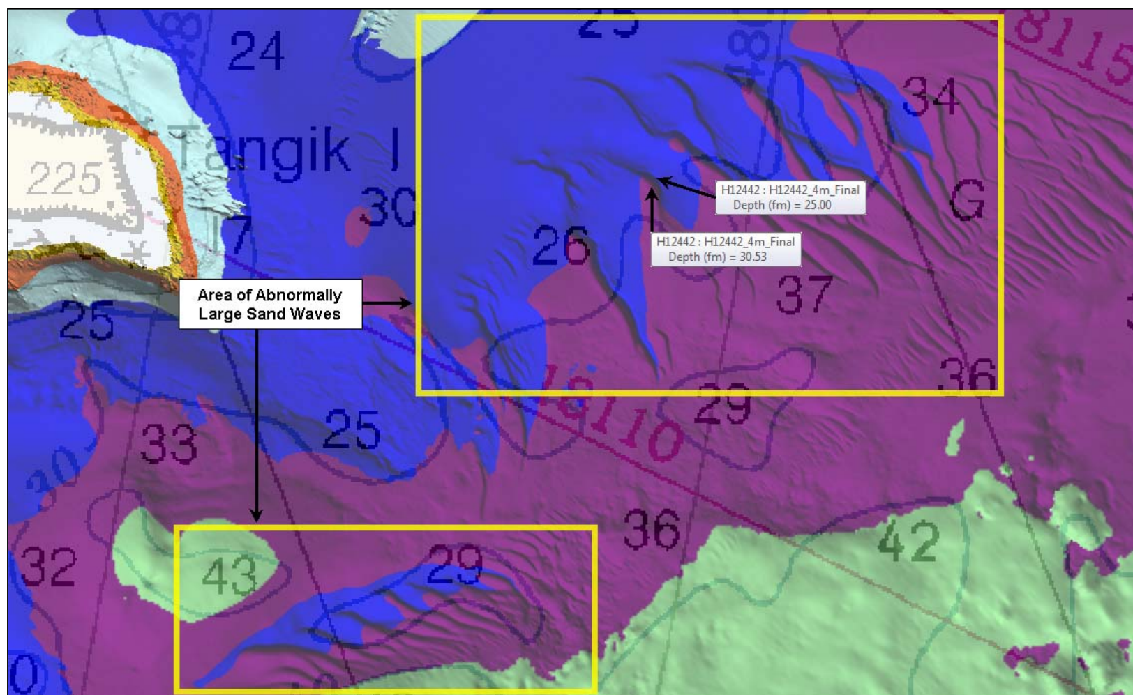
Figure 15 Sand Waves
