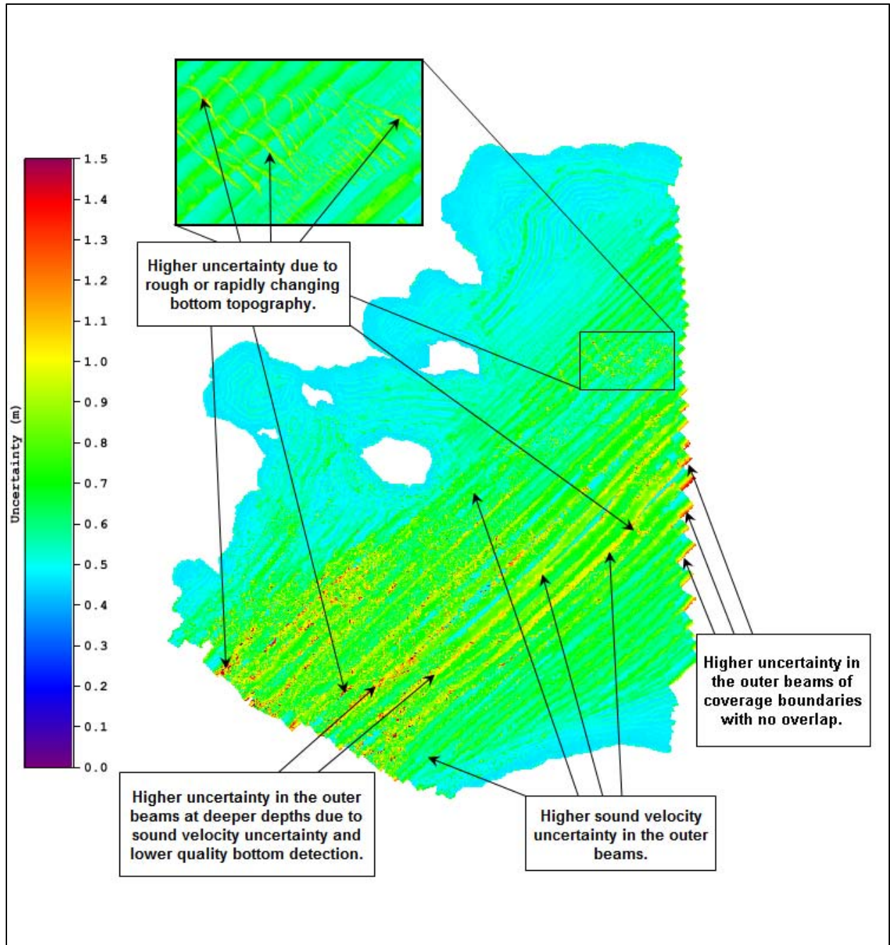
Figure 4 Uncertainty DTM
