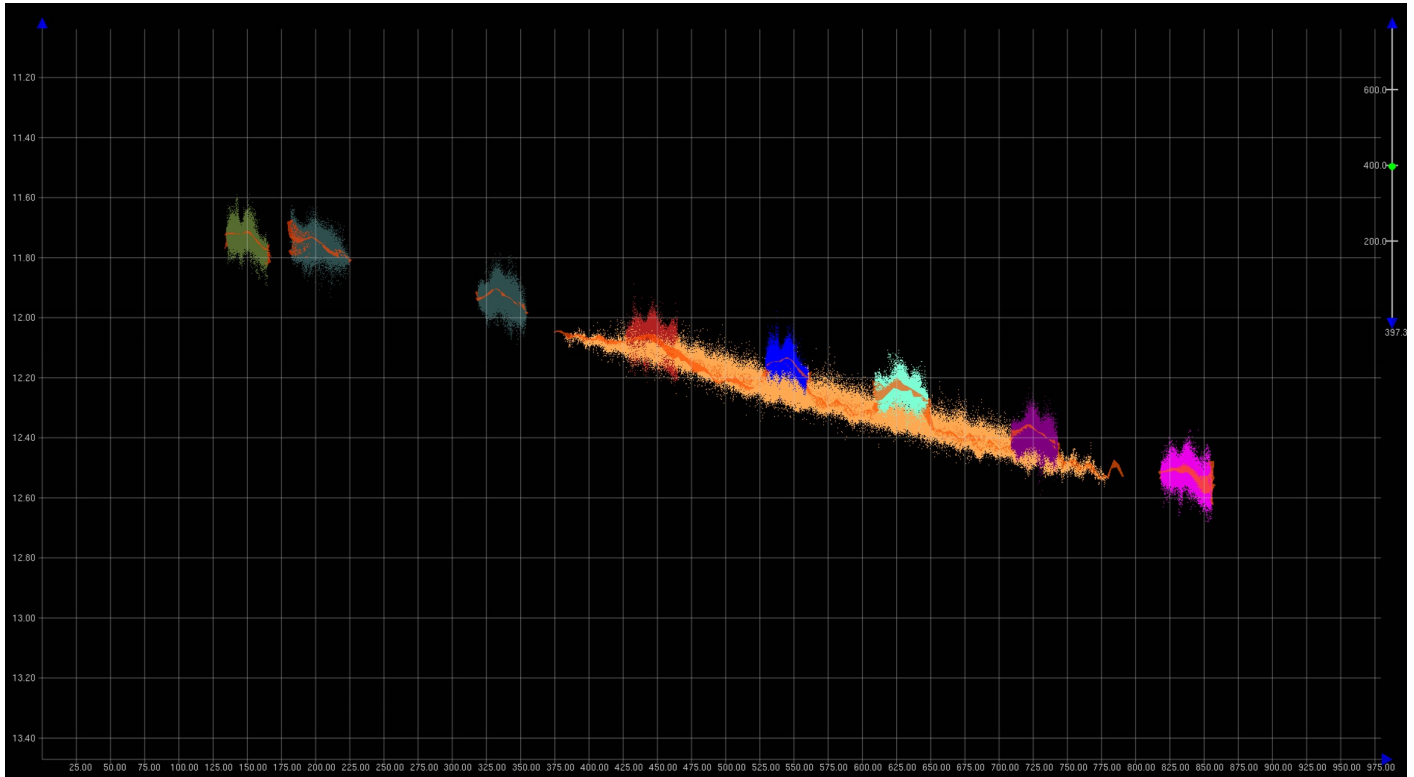
Figure 4: Example of tide bust of up to 0.10 m between a crossline (orange) and mainscheme lines.
