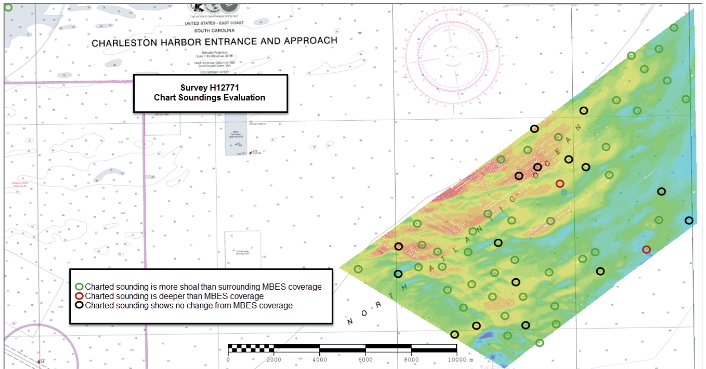
Figure 8: Charted soundings that fall between MBES lines
