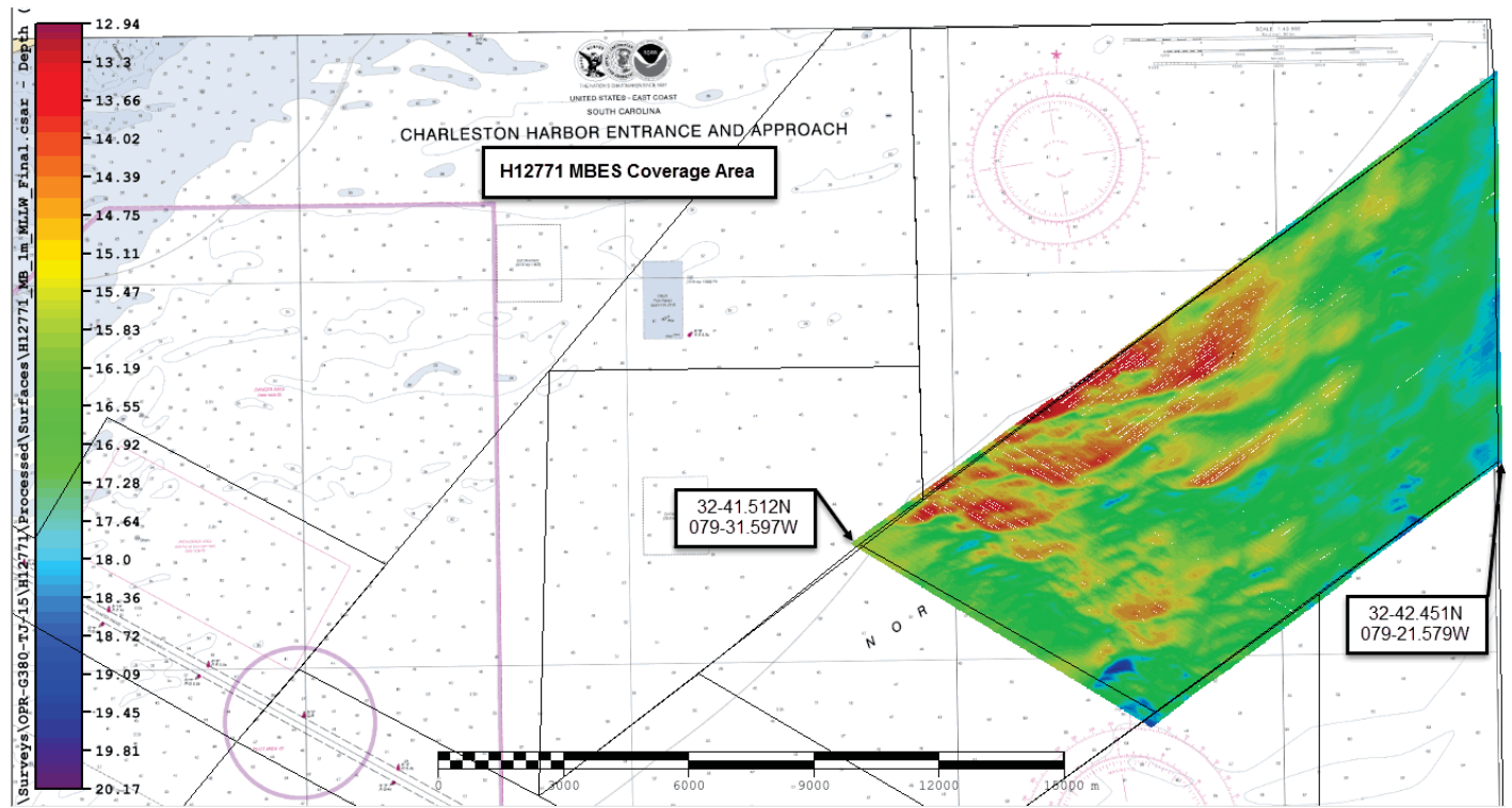
Figure 2: H12771 MBES Coverage
