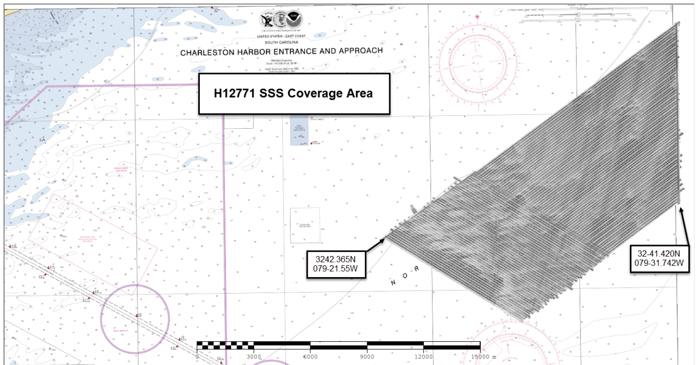
Figure 3: H12771 200% SSS Coverage
