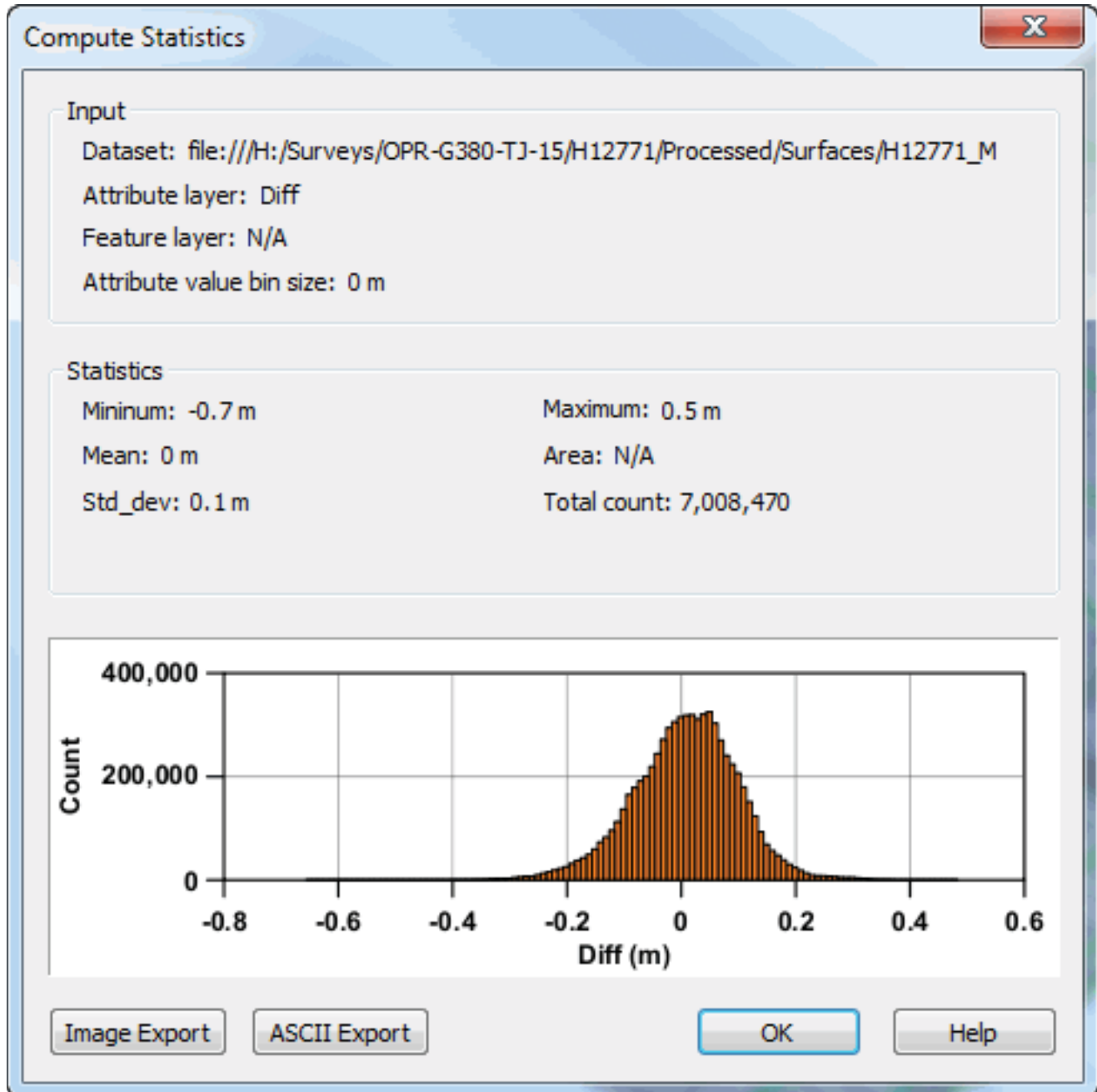
Figure 4: Survey H12771 Crossline to Mainscheme Depth Comparison
