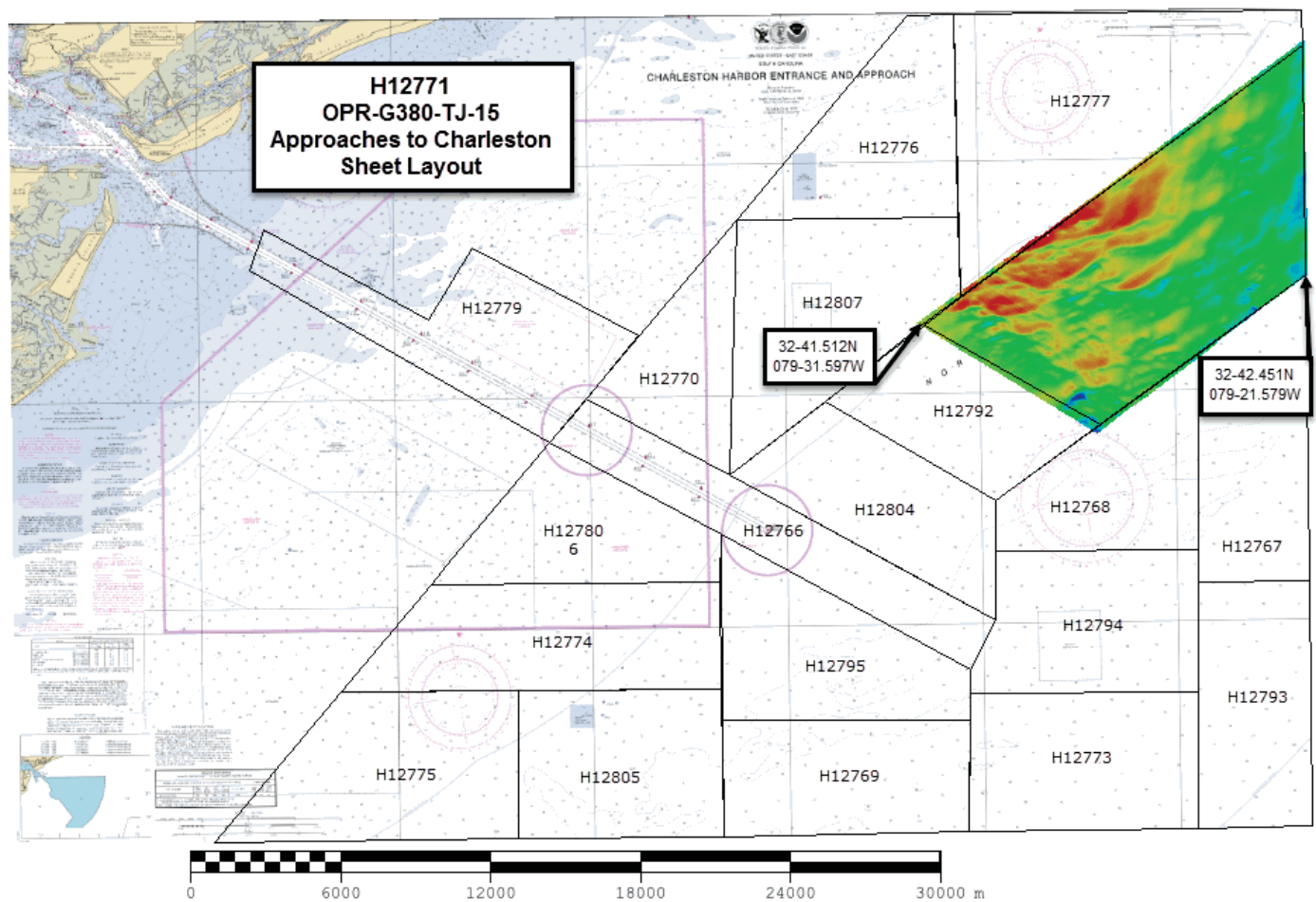
Figure 1: H12771 Survey Layout and Coverage are for OPR-G380-TJ-15, overlaid on RNC 11528
