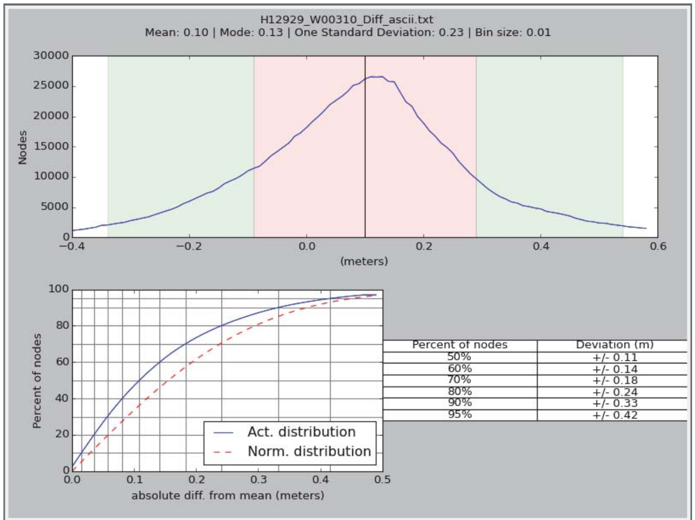
Figure 7: Difference Surface Statistics for H12929 and W00310 Junction.
