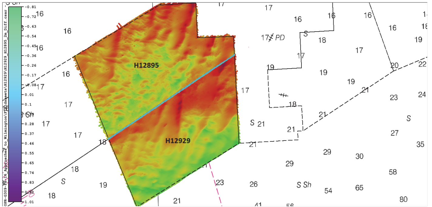
Figure 8: H12929 and H12895 Junction. The legend represents the difference surface values.
