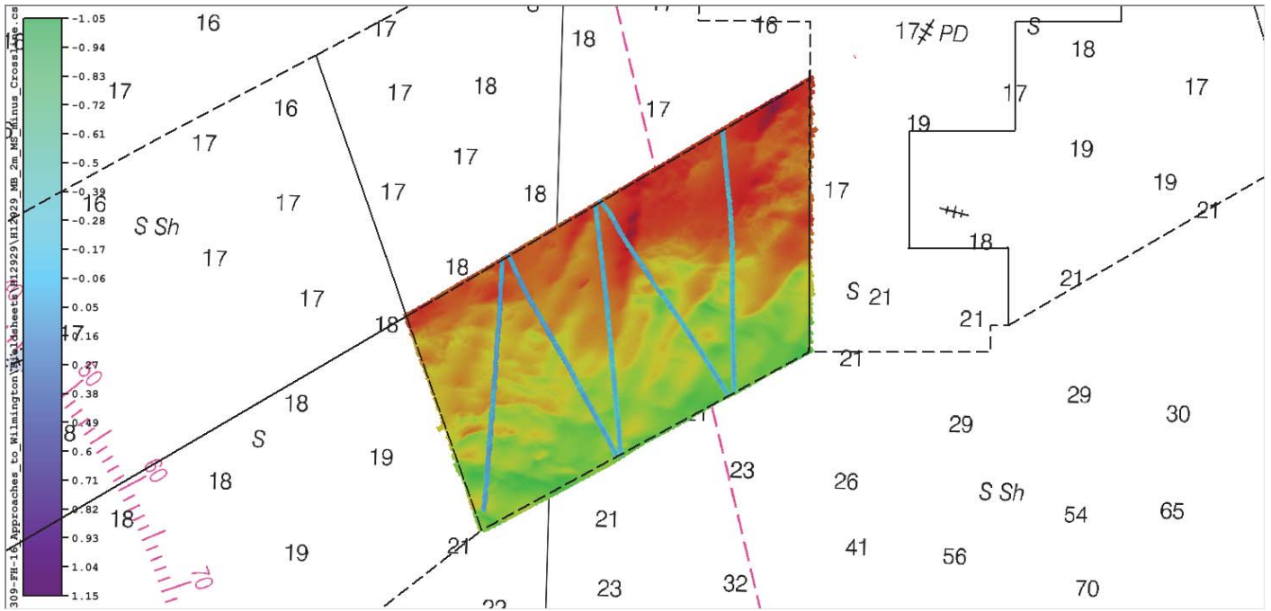
Figure 4: H12929 MBES crossline data overlaid on mainscheme data. The legend represents the difference surface value.
