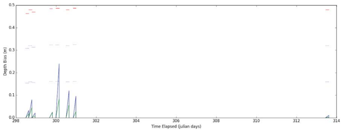
Figure 14: Ray Tracing Uncertainty Check for survey H12929. No casts in the graph exceeded the uncertainty limits shown by the red lines.
