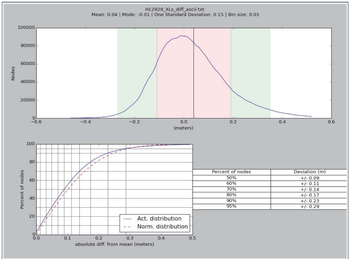
Figure 5: H12929 Crossline difference statistics: mainscheme minus crosslines.
