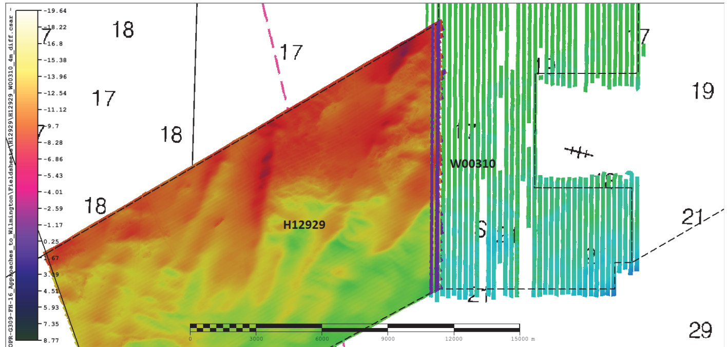
Figure 6: H12929 and W00310 junction. The legend represents the difference surface values.
