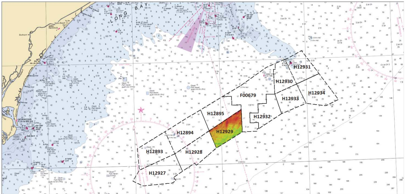
Figure 1: H12929 Survey Limits
