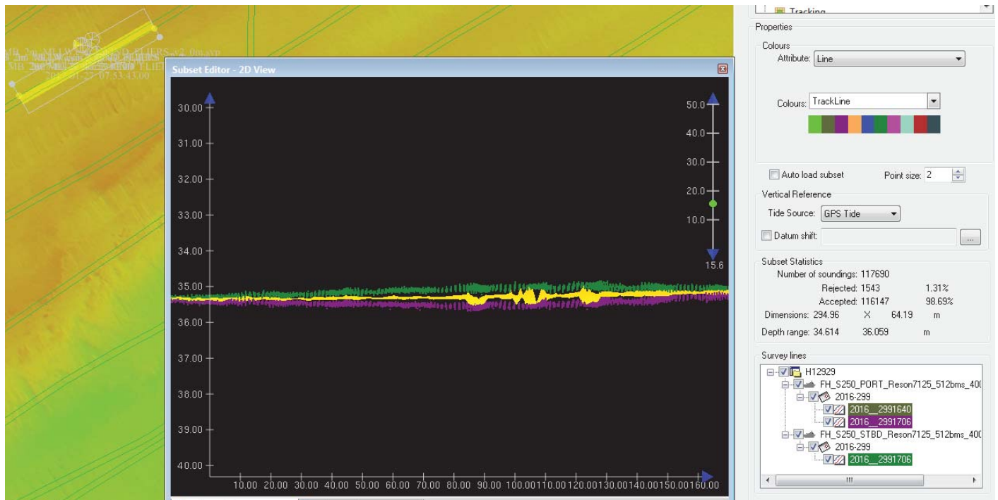
Figure 10: Example of SBET anomaly
