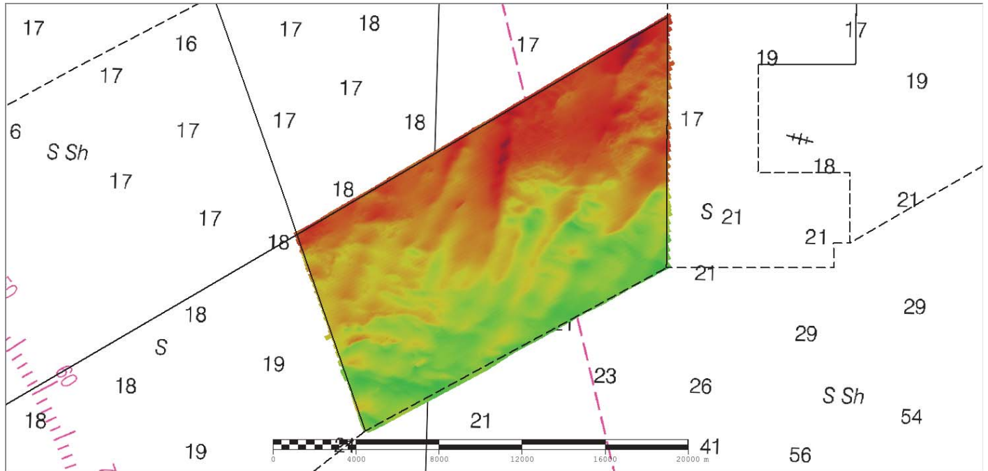
Figure 2: Survey Layout for survey H12929 overlaying RNC 11520.
