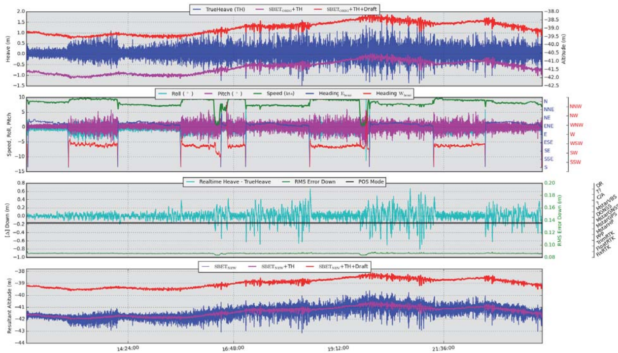
Figure 11: SBET corresponding to survey lines in figure 10
