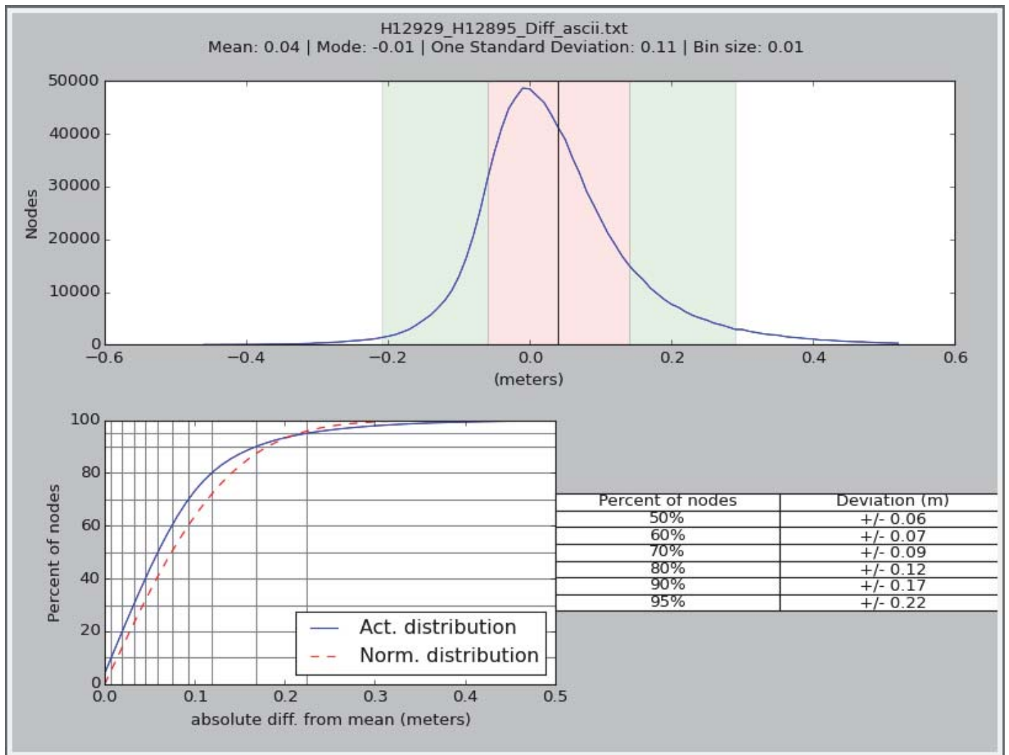
Figure 9: Difference Surface Statistics for the H12929 and H12895 junction.
