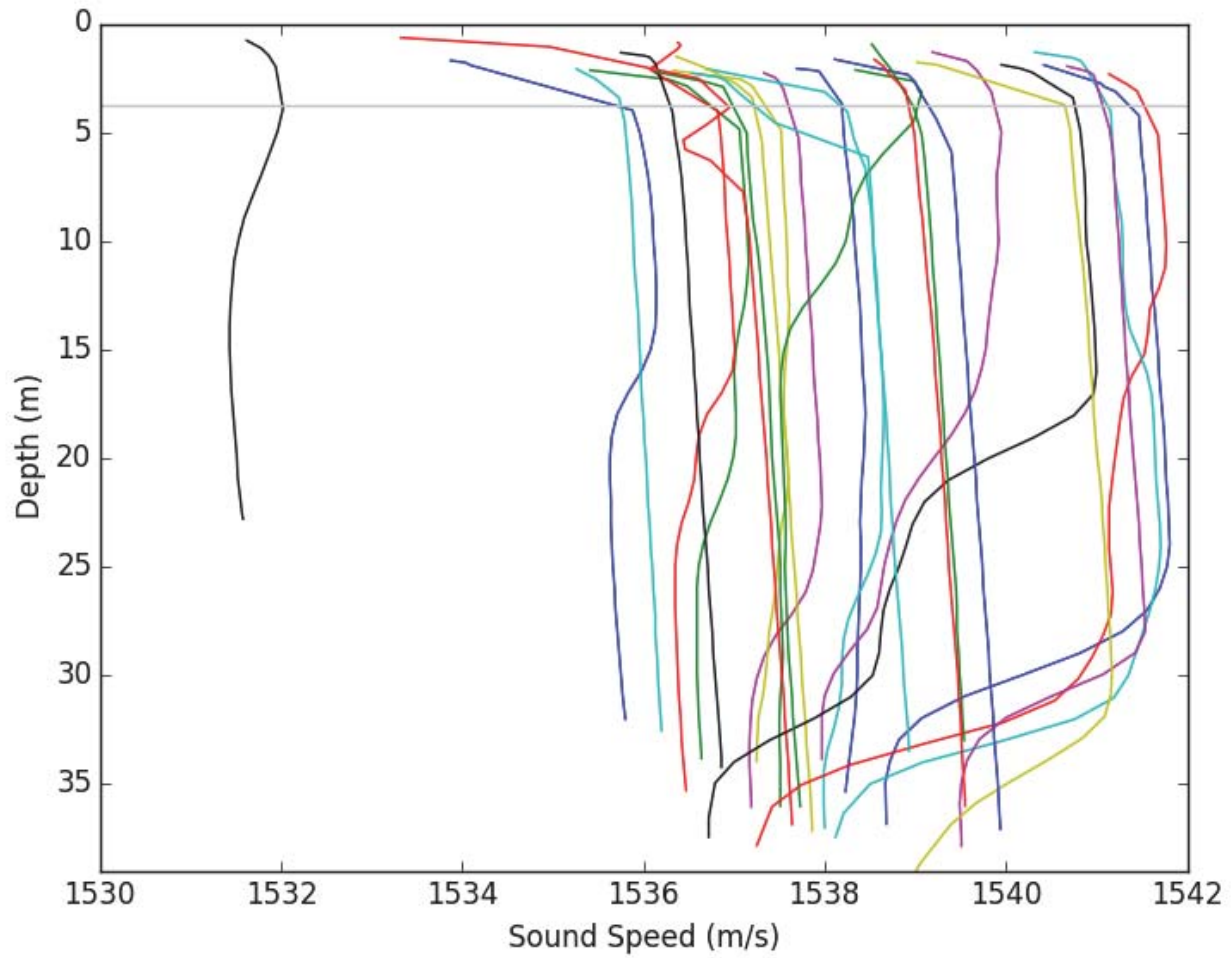
Figure 13: Sound Speed Profiles for survey H12929
