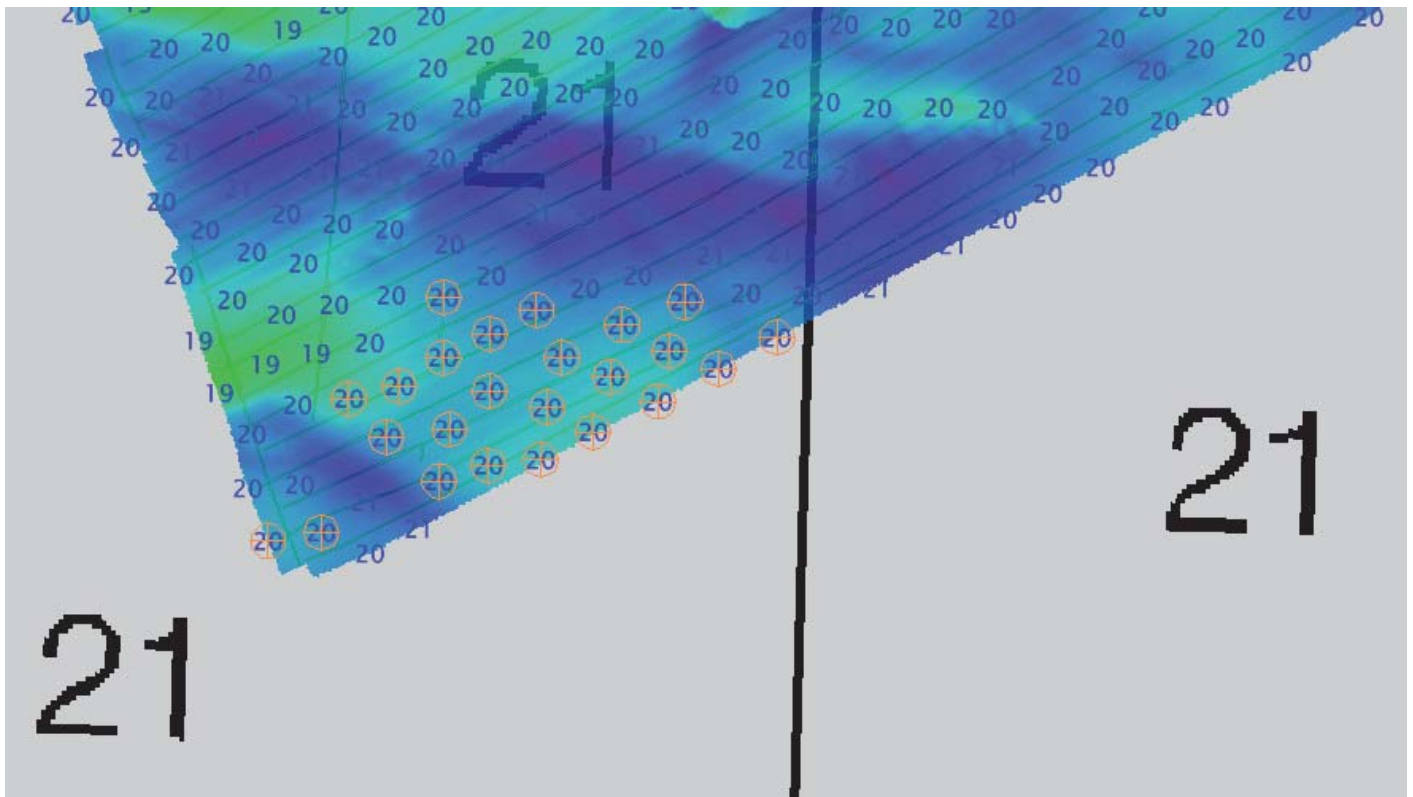
Figure 21: Zoom showing minor shoaling in the region of 33-05-20 N and 78-01-02 W. Soundings flagged in orange are approximately 1 fathom shallower than currently charted nearby soundings.
