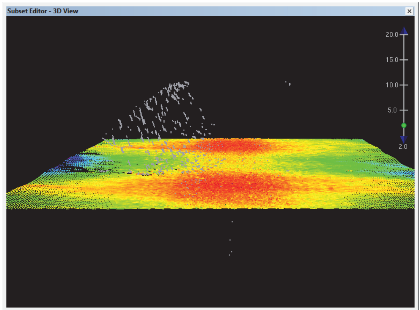
Figure 9: CARIS HIPS 3D View of Rejected Biomass
