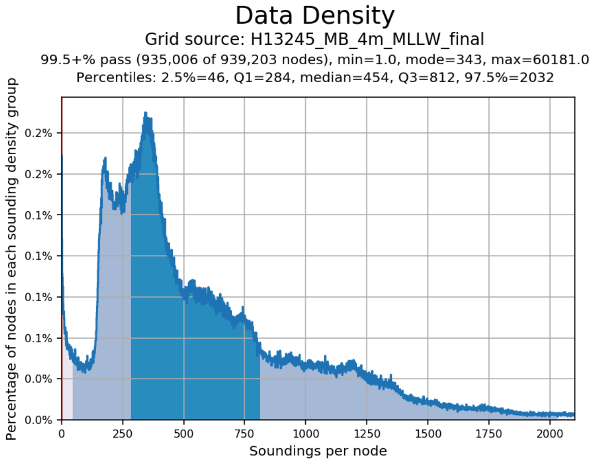
Figure 11: H13245 Data density statistics
