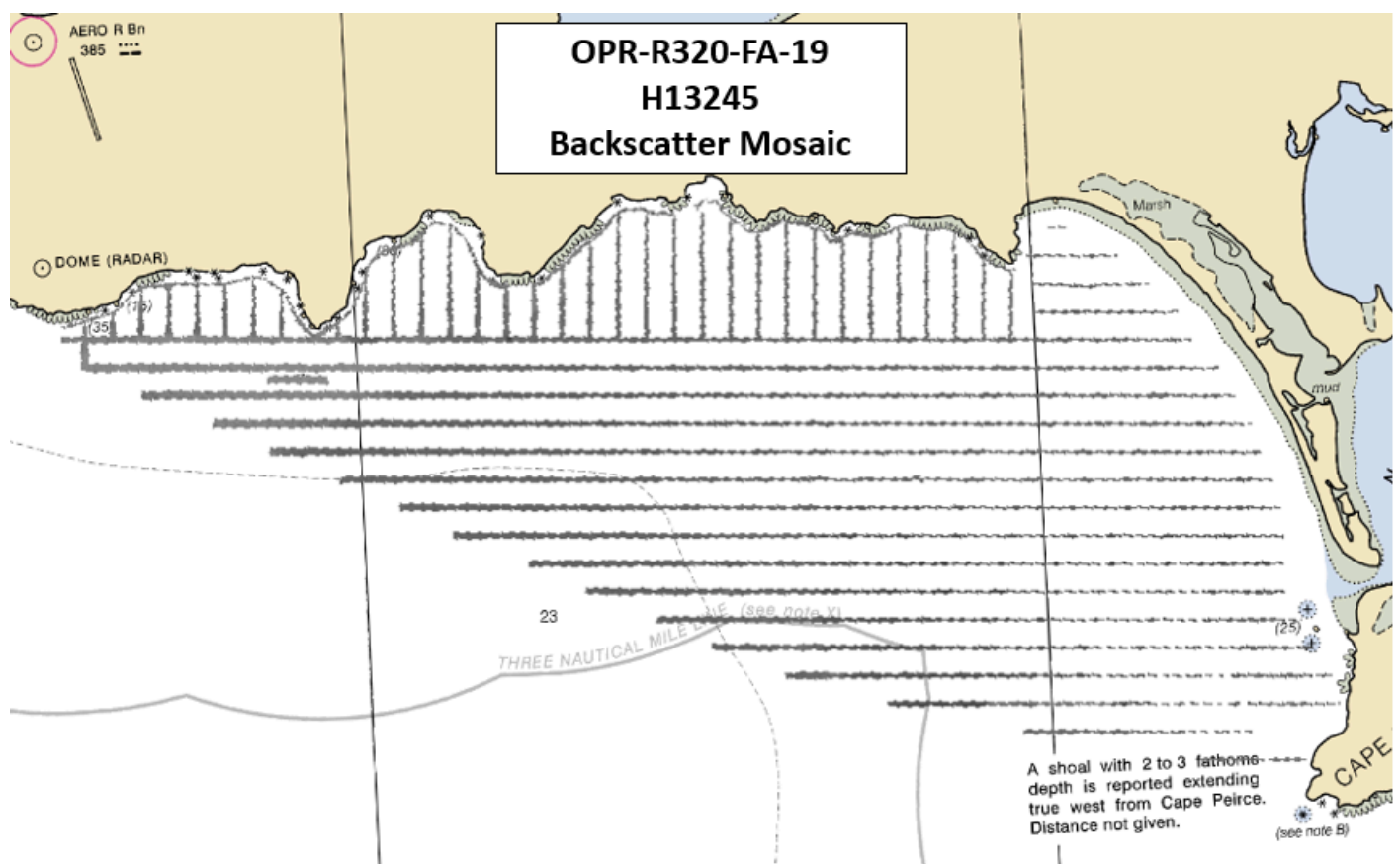
Figure 12: Backscatter Mosaic for H13245
