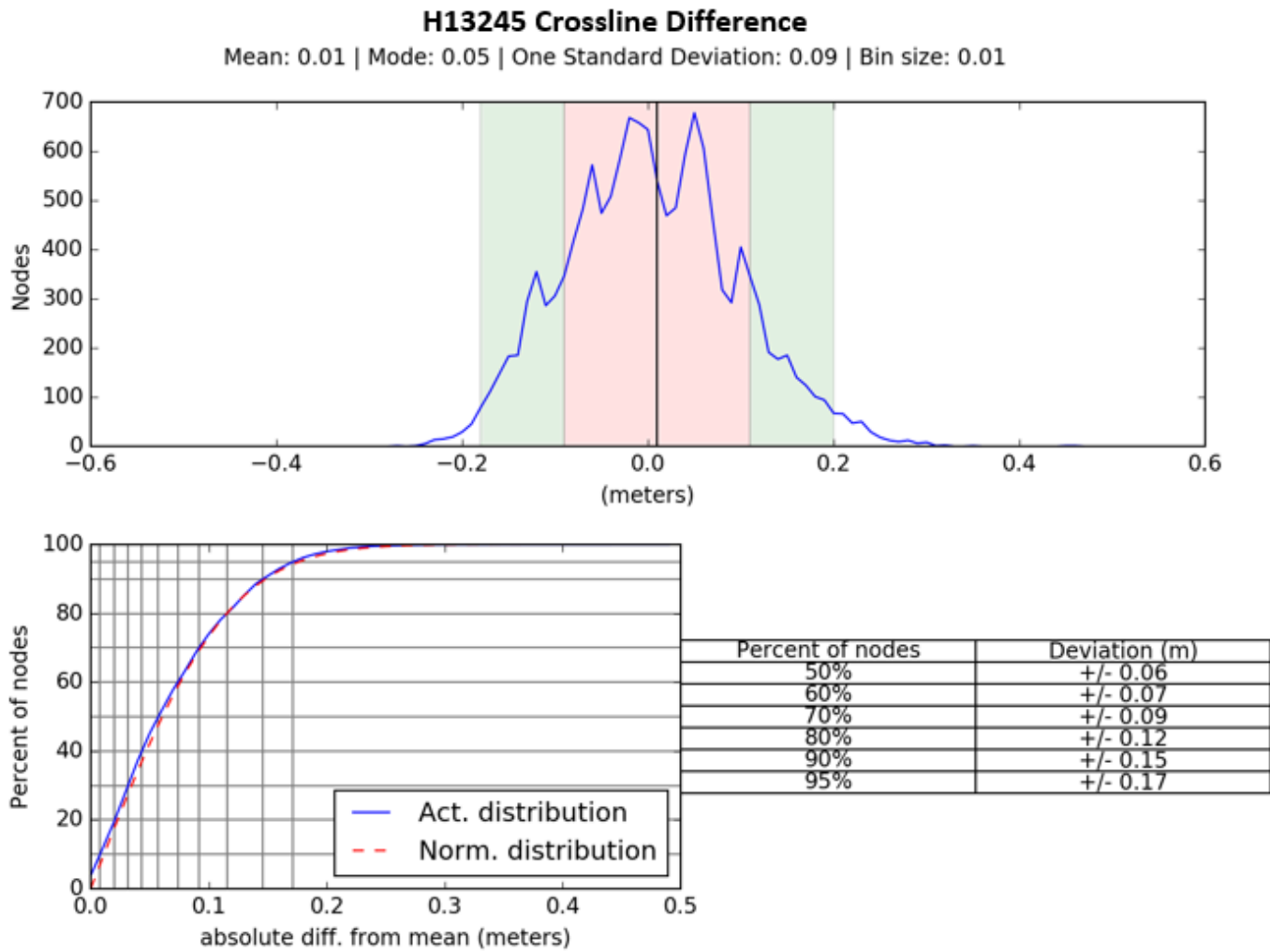
Figure 4: H13245 Crossline and Mainscheme Difference Statistics
