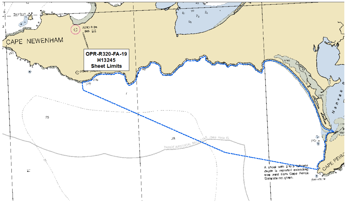
Figure 1: H13245 sheet limits (in blue) overlaid onto chart 16305
