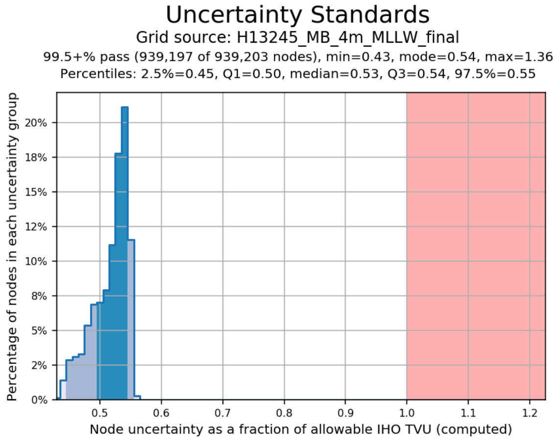
Figure 10: H13245 Allowable uncertainty statistics
