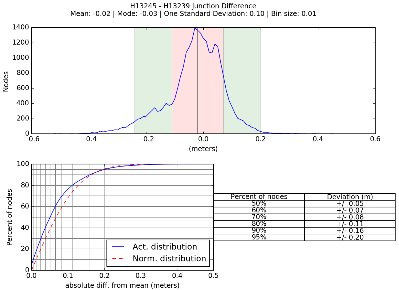
Figure 9: Difference surface statistics between H13245 and H13239 (4 meter surface)
