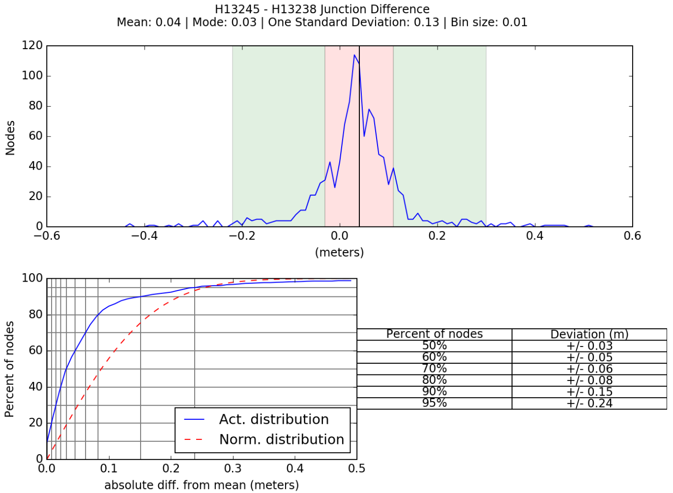
Figure 7: Difference surface statistics between H13245 and H13238 (4 meter surface)
