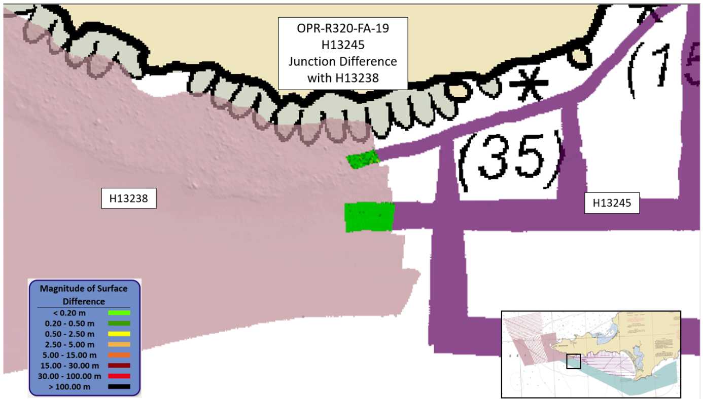
Figure 6: Difference surface between H13245 (purple) and junctioning survey H13238 (pink)
