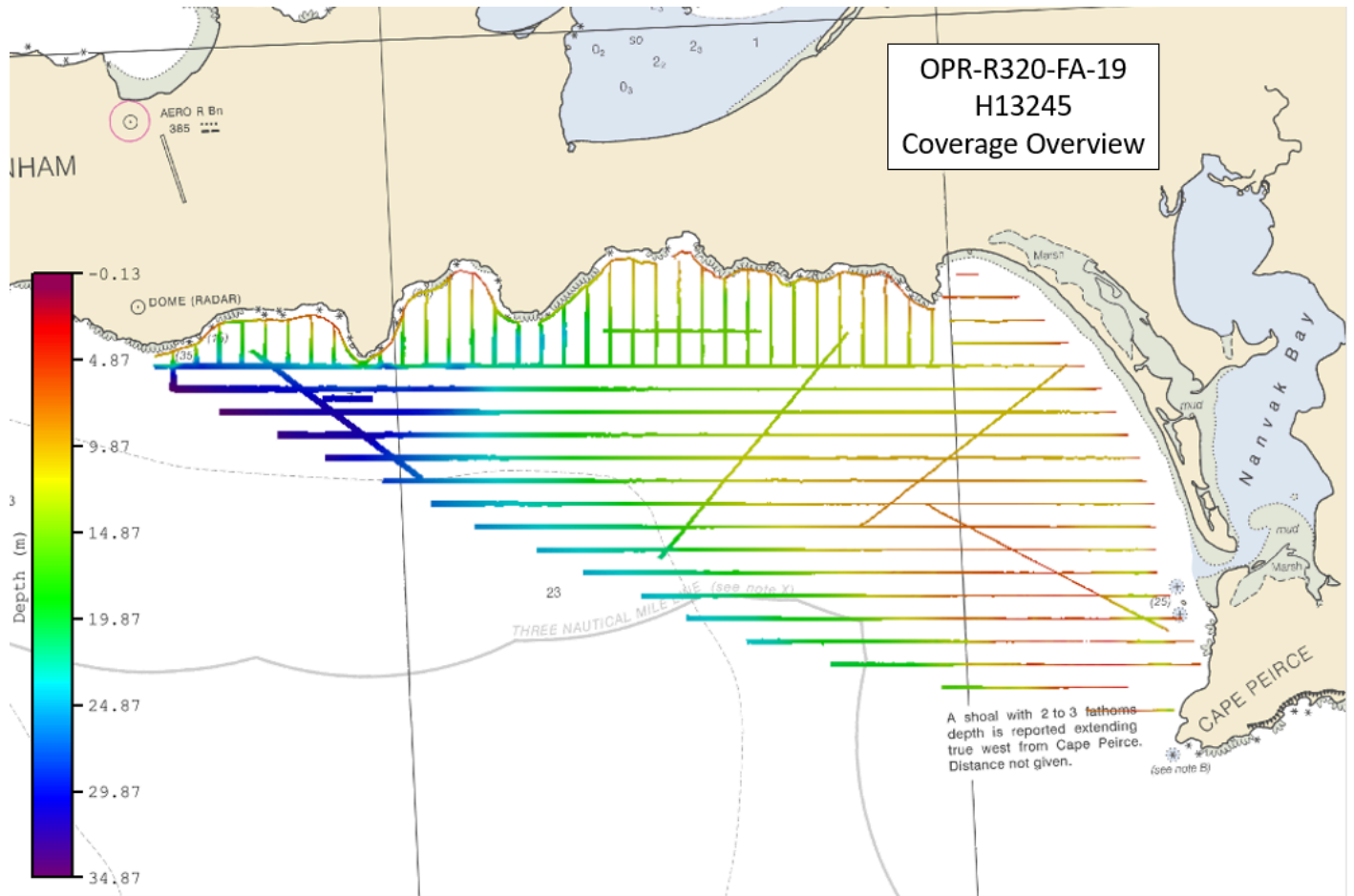
Figure 2: H13245 survey coverage overlaid onto Chart 16305
