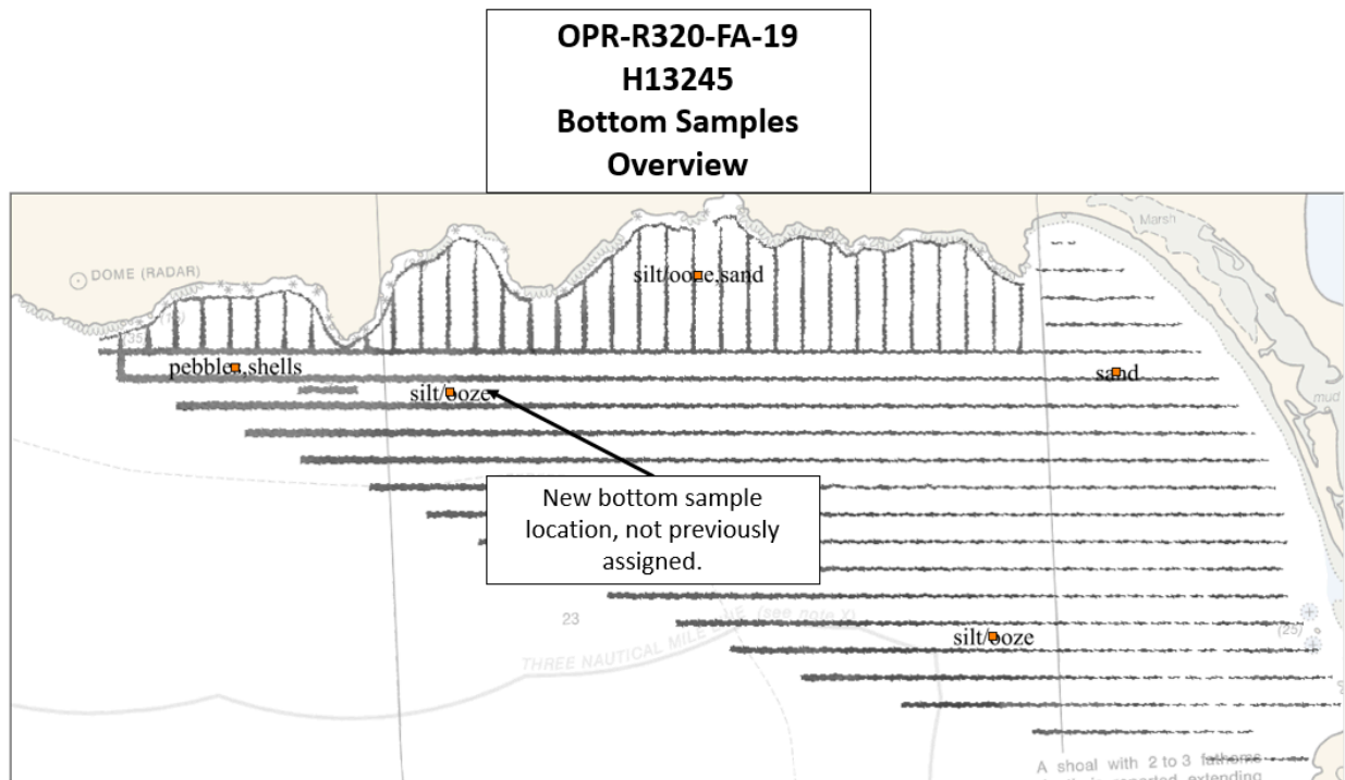
Figure 14: H13245 Bottom sample locations
