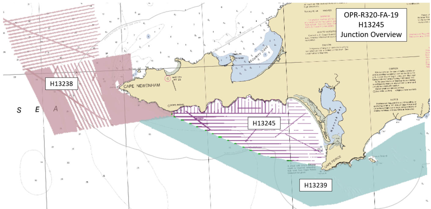
Figure 5: Overview of H13245 junction surveys
