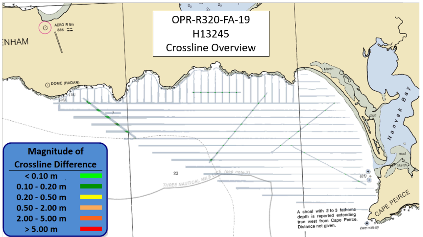
Figure 3: Overview of H13245 Crosslines
