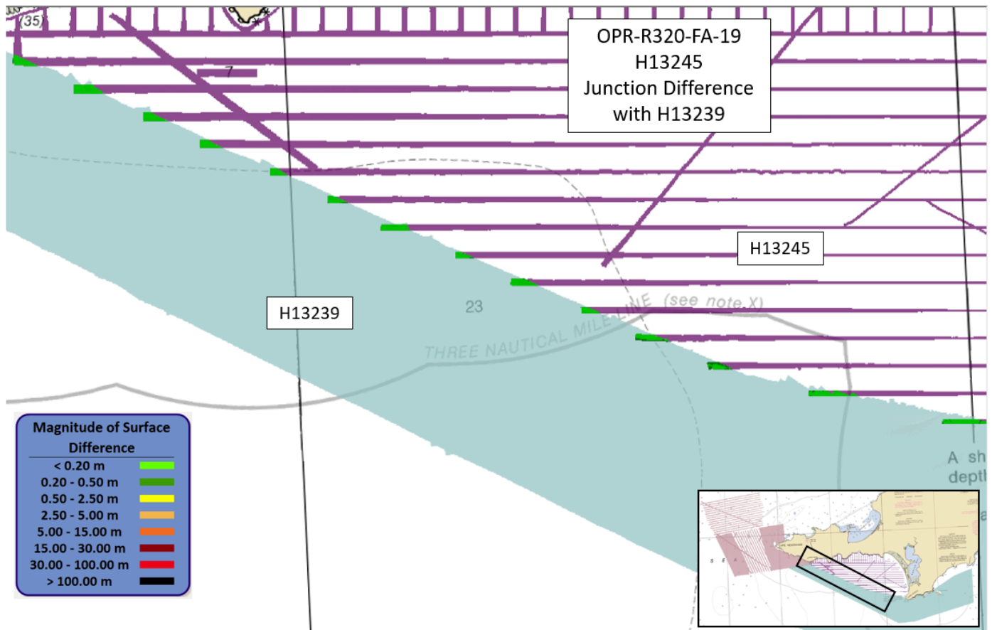
Figure 8: Difference surface between H13245 (purple) and junctioning survey H13239 (light blue)
