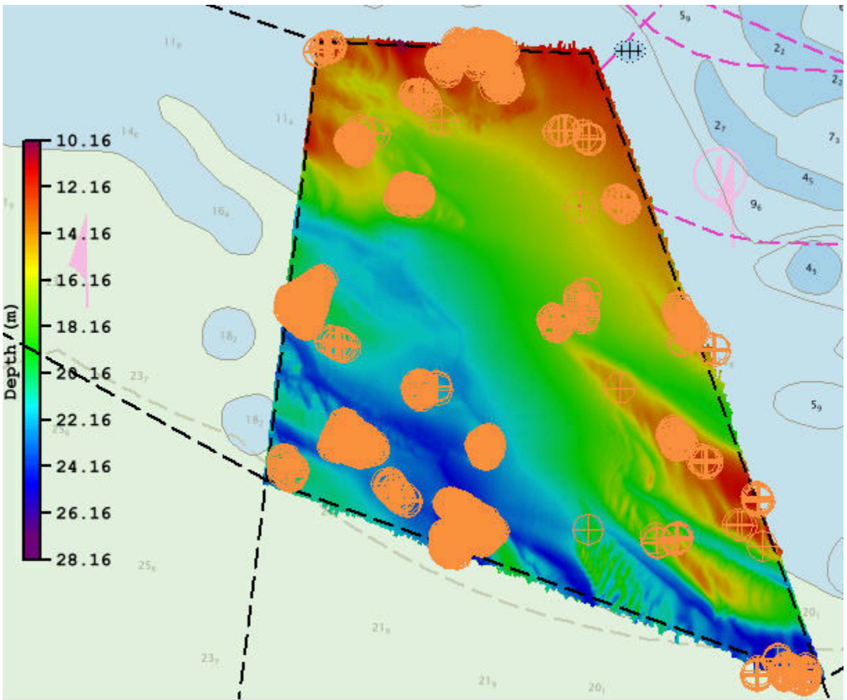
Figure 15: Pydro QC Tools output of areas of shoaling greater than 1ft
