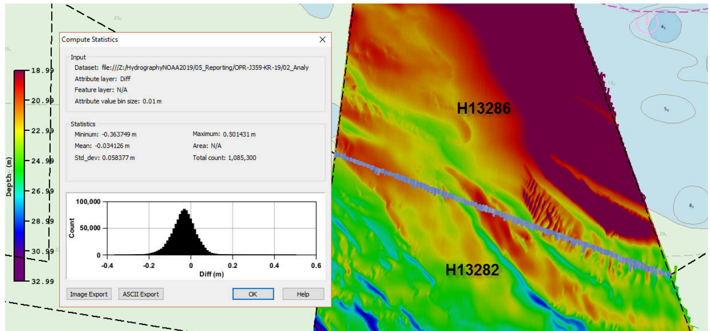
Figure 10: Survey H13286 junction with Survey H13282
