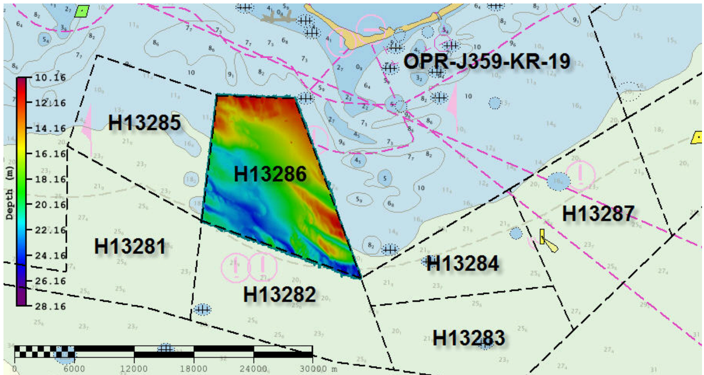
Figure 1: Survey H13286 relative to overall sheet limits of OPR-J359-KR-19
