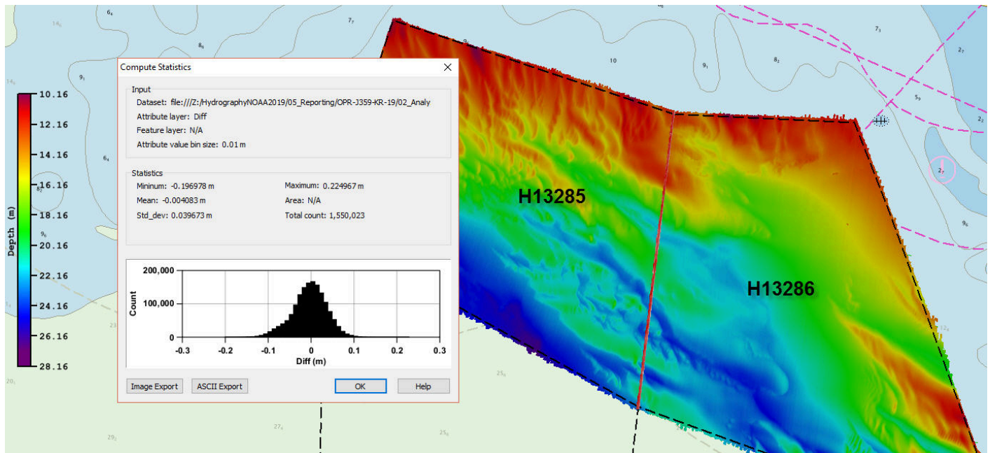
Figure 11: Survey H13286 junction with Survey H13285
