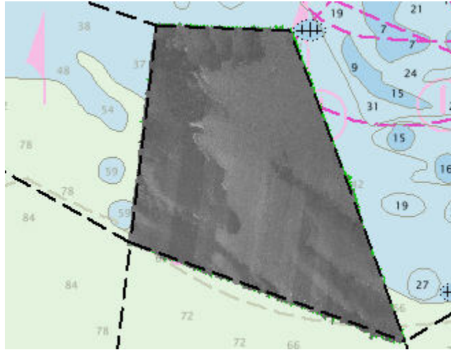
Figure 13: Survey H13286 backscatter coverage
