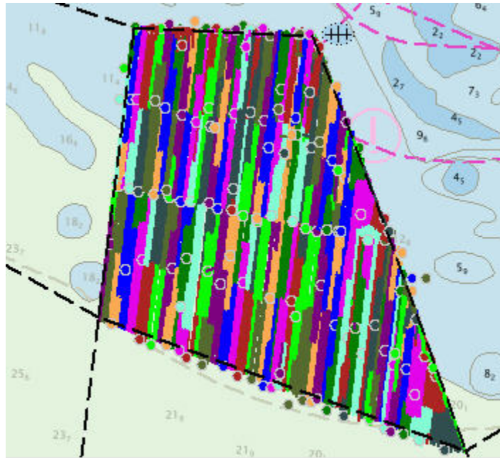
Figure 12: Temporal and geographic distribution of SVP casts within survey H13286
