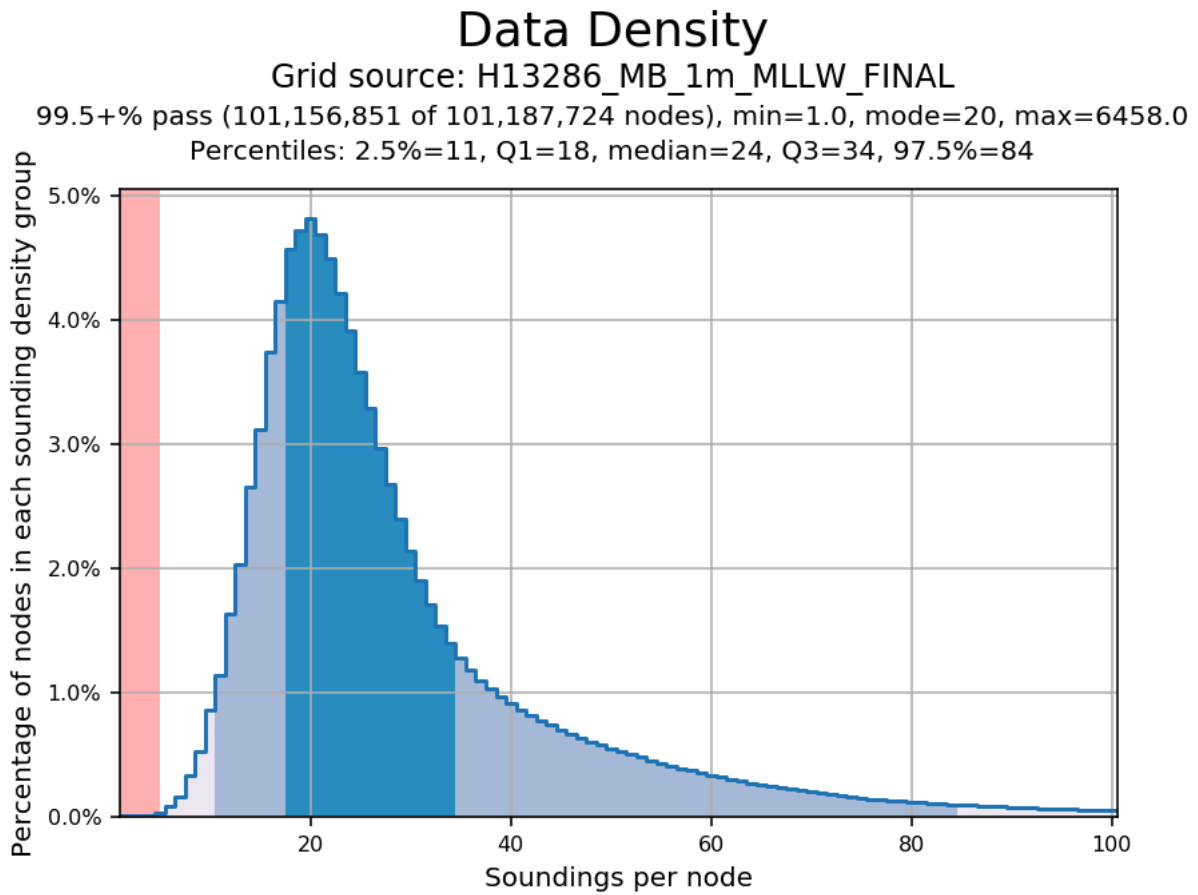
Figure 3: Survey H13286 1m complete coverage MBES density QC
