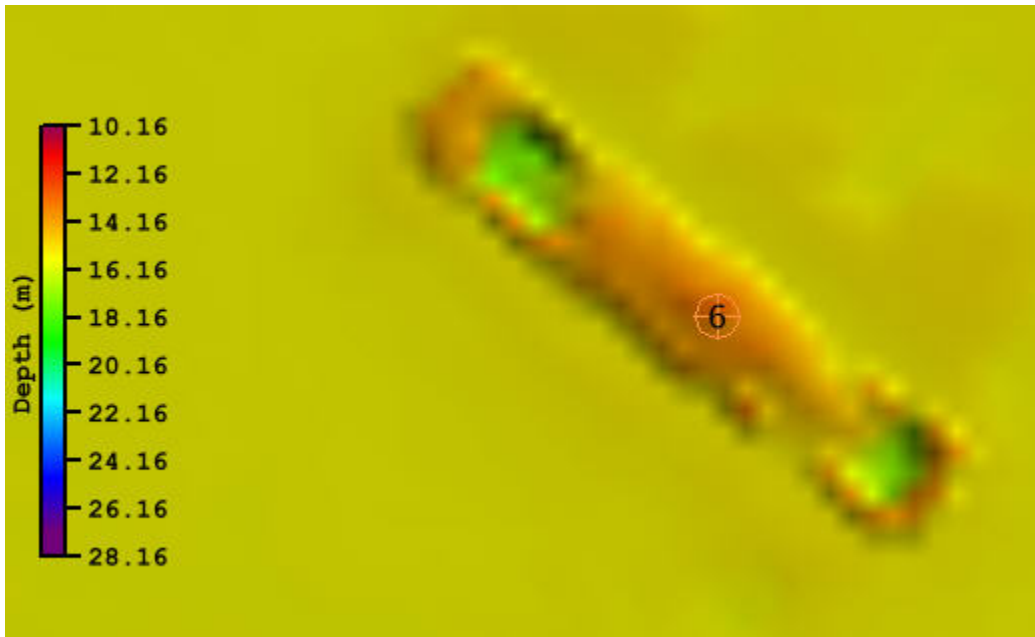
Figure 16: Survey H13286 sounding shoal to charted; uncharted wreck
