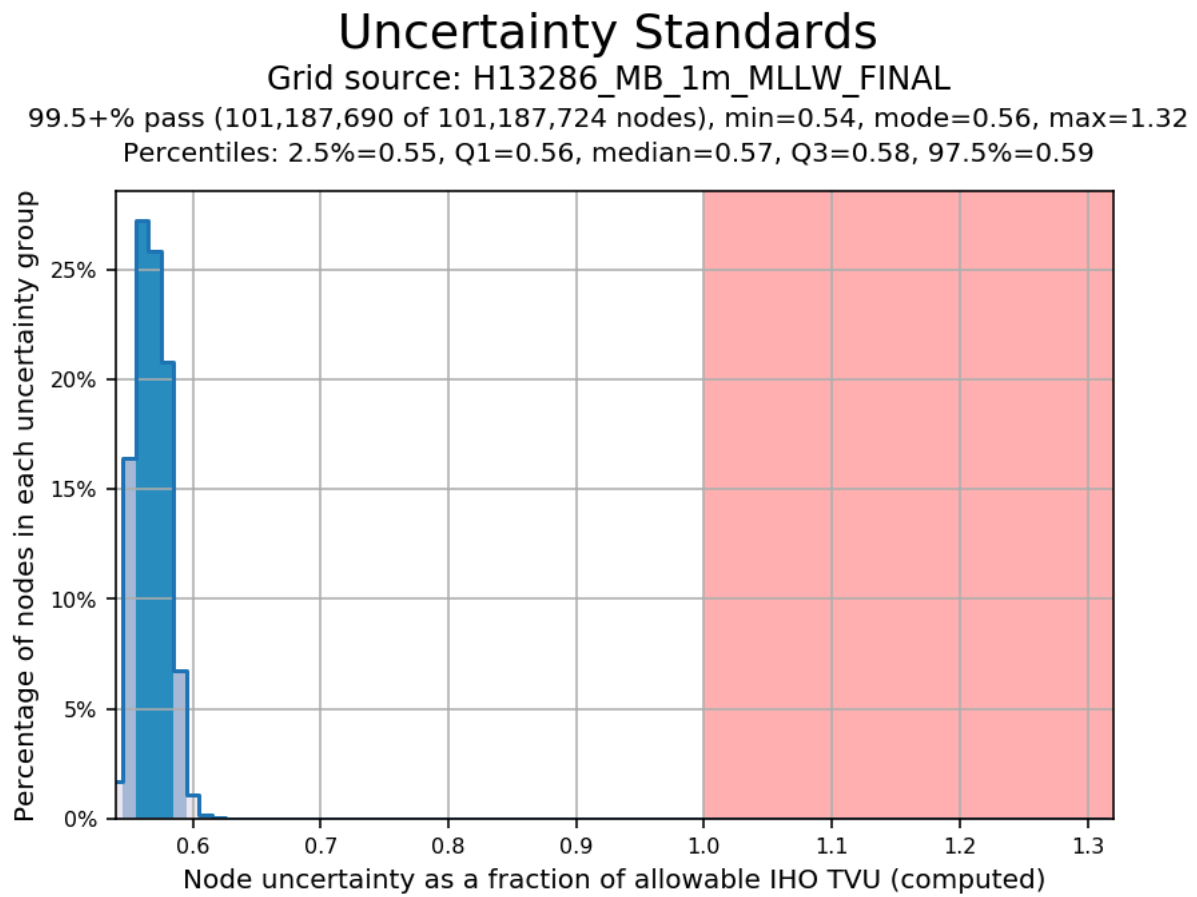
Figure 8: H13286 1m finalized grid TPU QC
