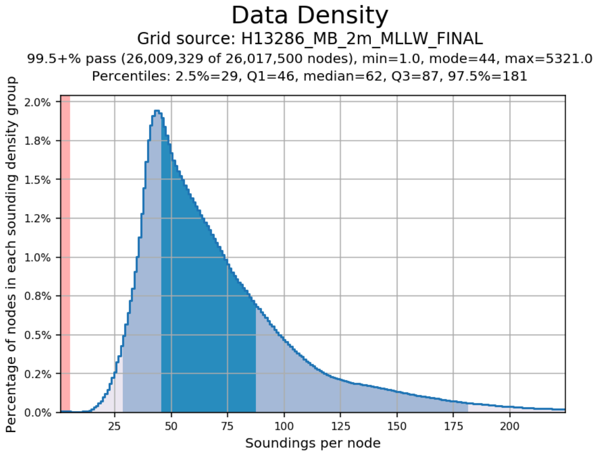
Figure 4: Survey H13286 2m complete coverage MBES density QC
