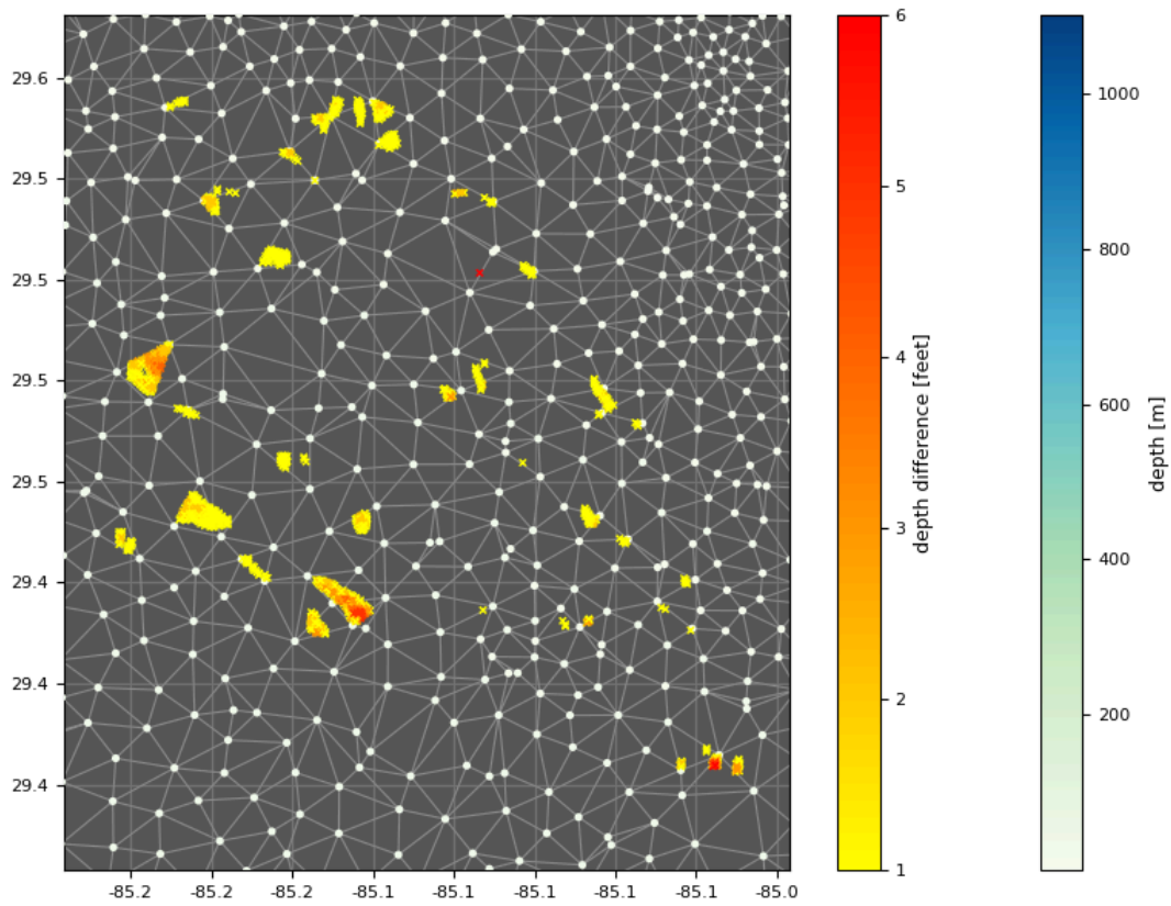
Figure 14: Pydro QC Tools chart review output of H13286 surveyed soundings shoal to charted soundings
