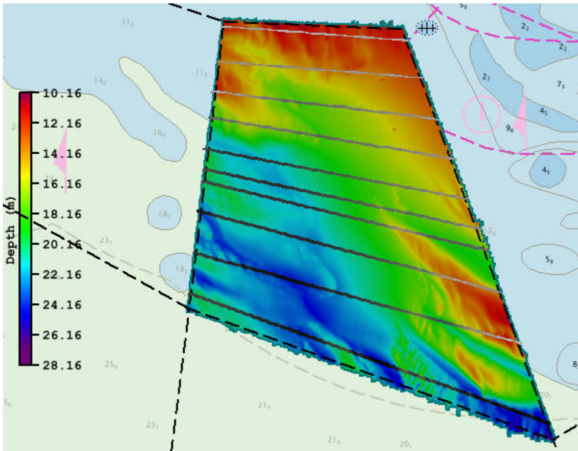
Figure 6: H13286 MBES mainscheme and MBES crossline distribution
