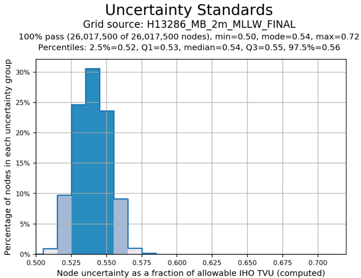
Figure 9: H13286 2m finalized grid TPU QC
