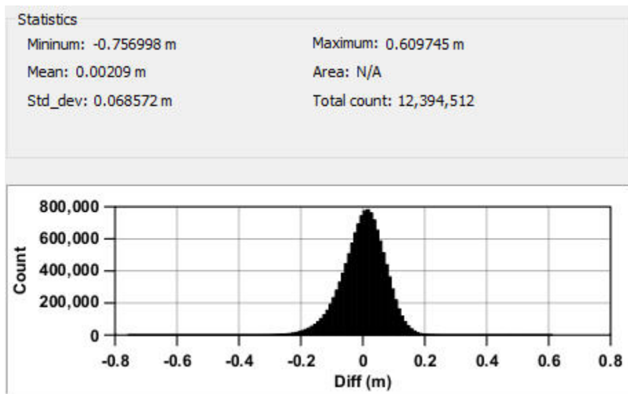
Figure 7: H13286 MBES mainscheme differenced from MBES crosslines statistical output
