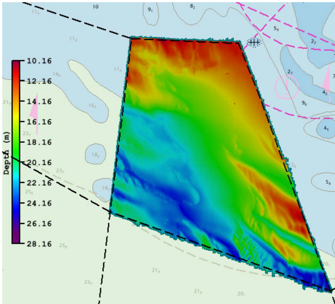
Figure 2: Survey H13286 complete coverage MBES
