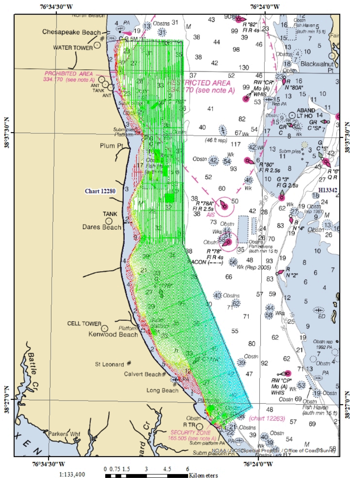
Figure 2: Final Bathymetry Coverage for H13343
