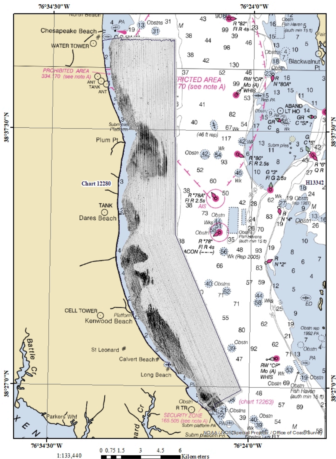
Figure 3: Final Side Scan Coverage for H13343 (First 100% coverage)
