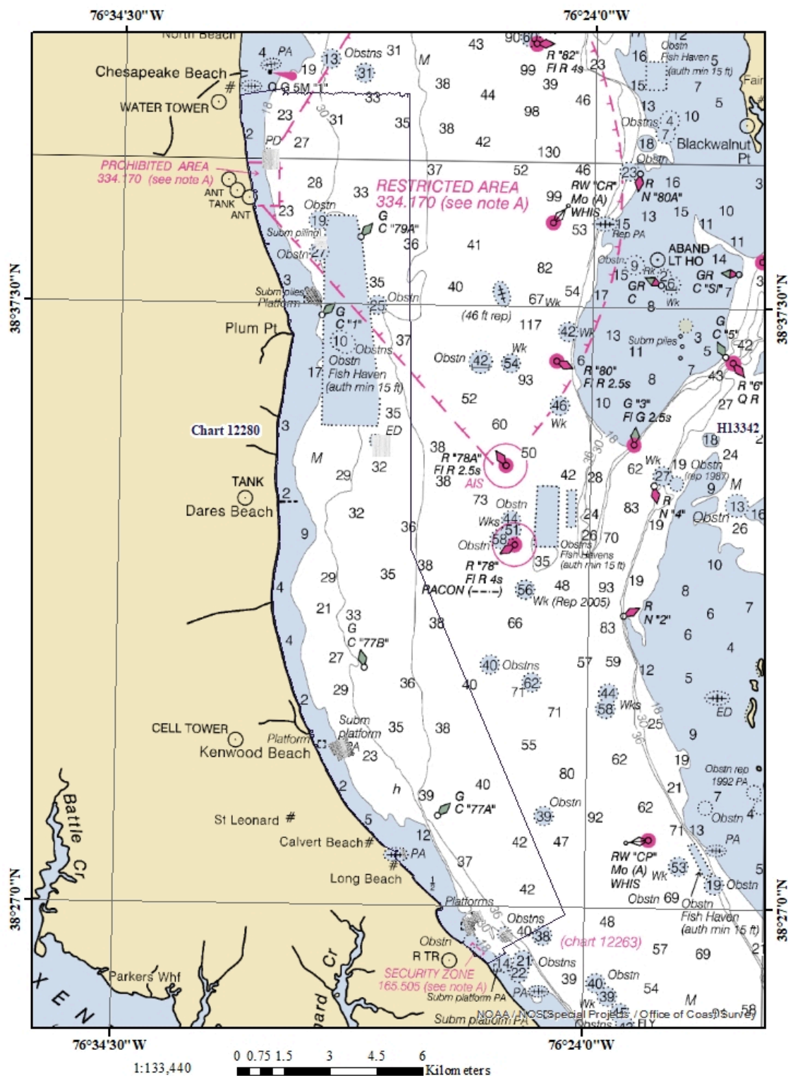
Figure 4: Final Side Scan Coverage for H13343 (Second 100% coverage)
