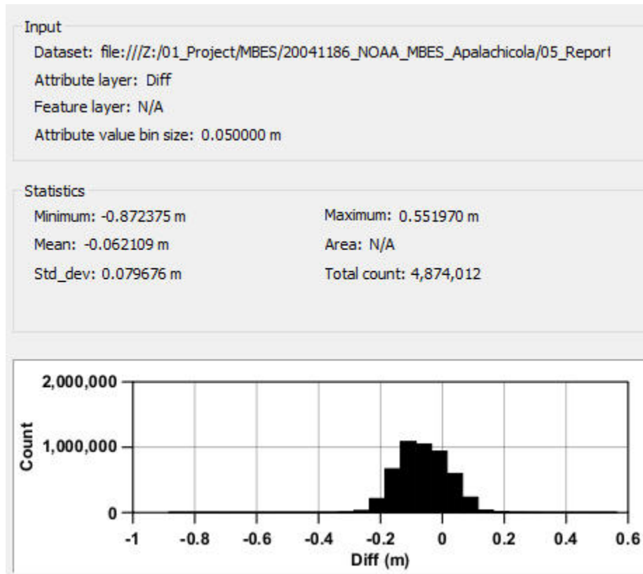
Figure 12: Survey H13358 junction with Survey H13357
