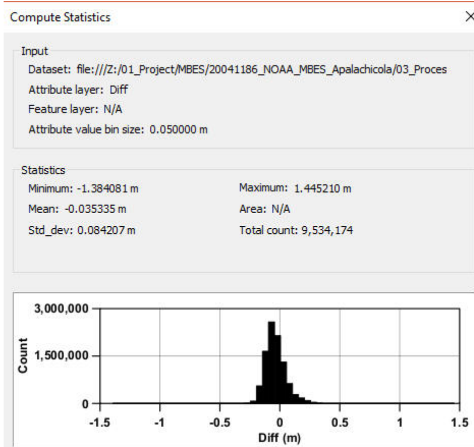
Figure 8: H13358 MBES mainscheme differenced from MBES crosslines statistical output
