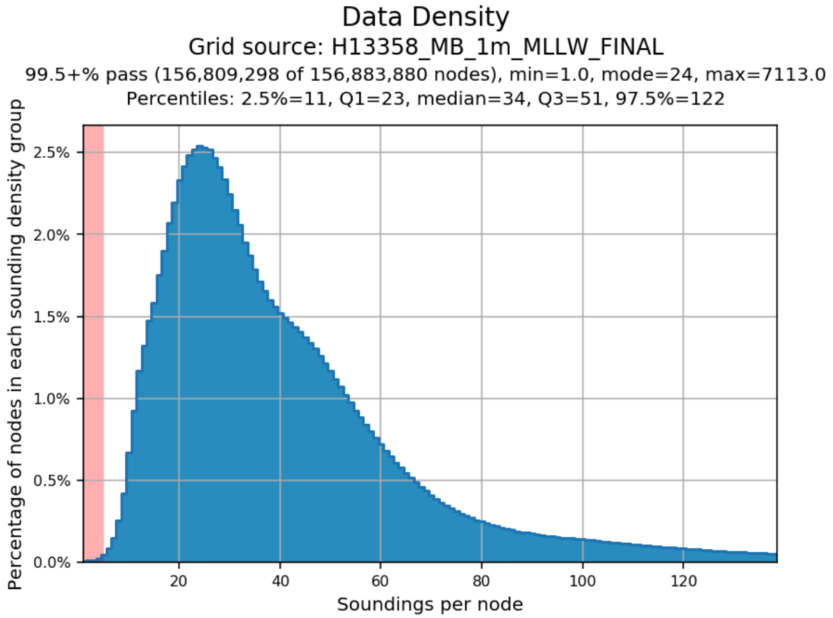
Figure 3: Survey H13358 1m complete coverage MBES density QC
