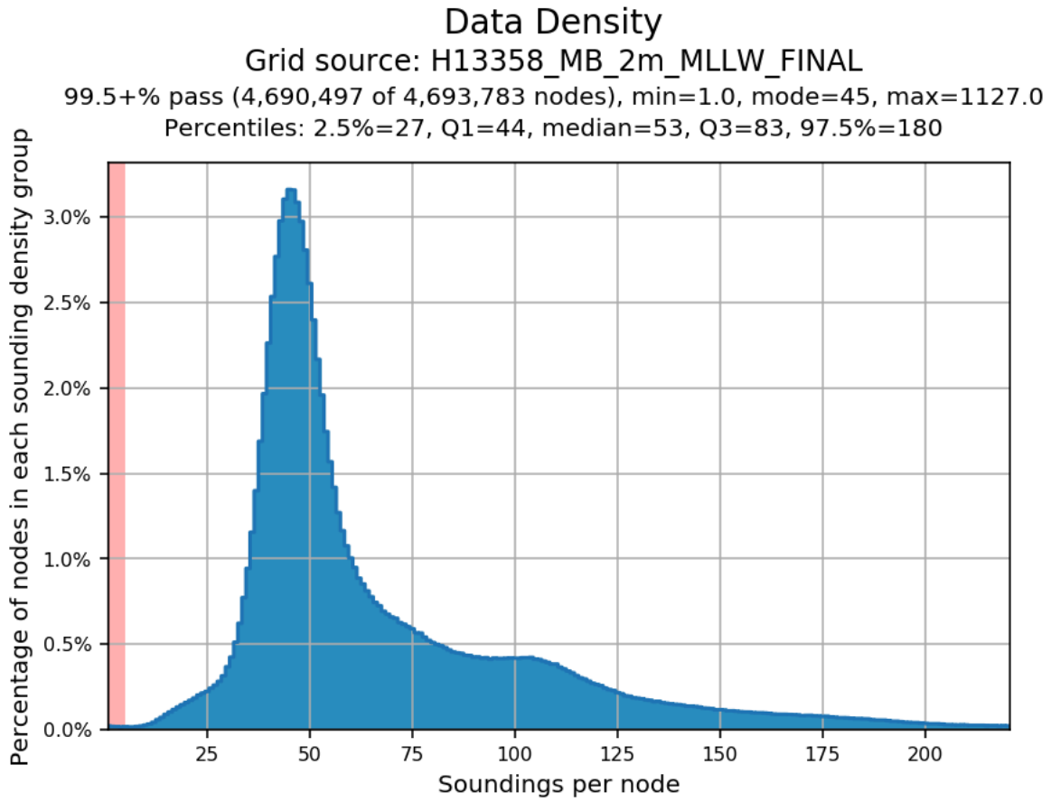
Figure 4: Survey H13358 2m complete coverage MBES density QC
