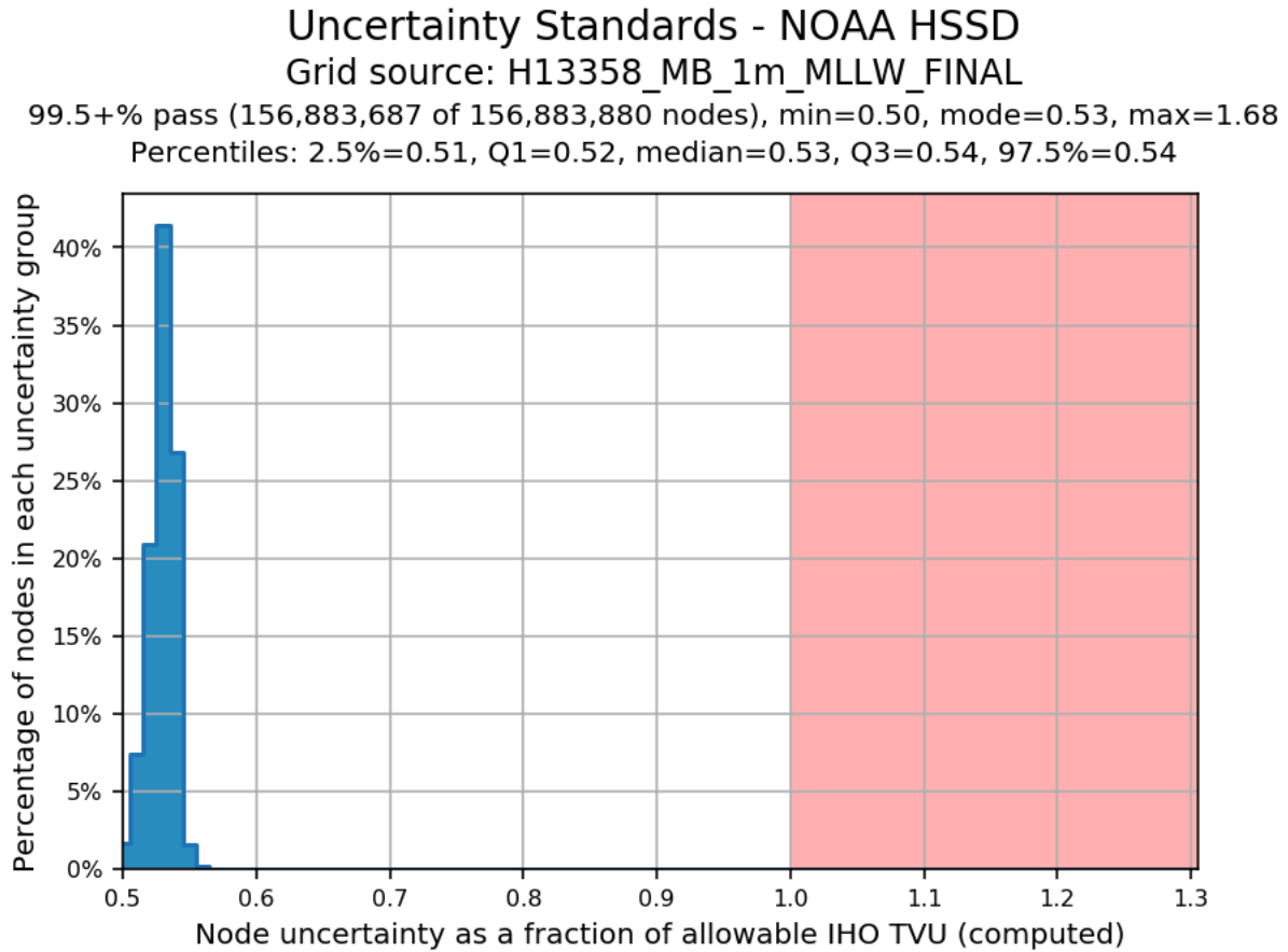
Figure 9: H13358 1m finalized grid TPU QC
