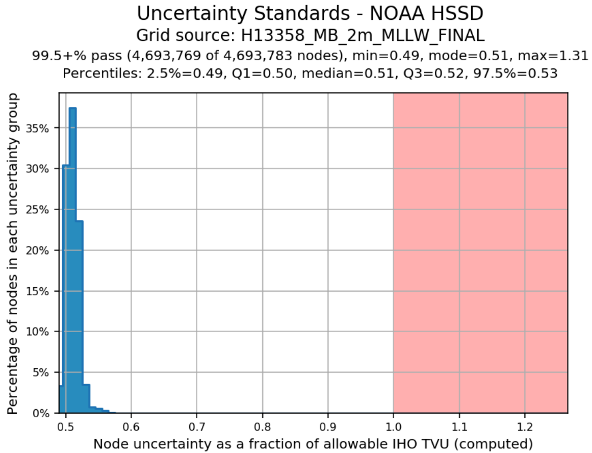
Figure 10: H13358 2m finalized grid TPU QC
