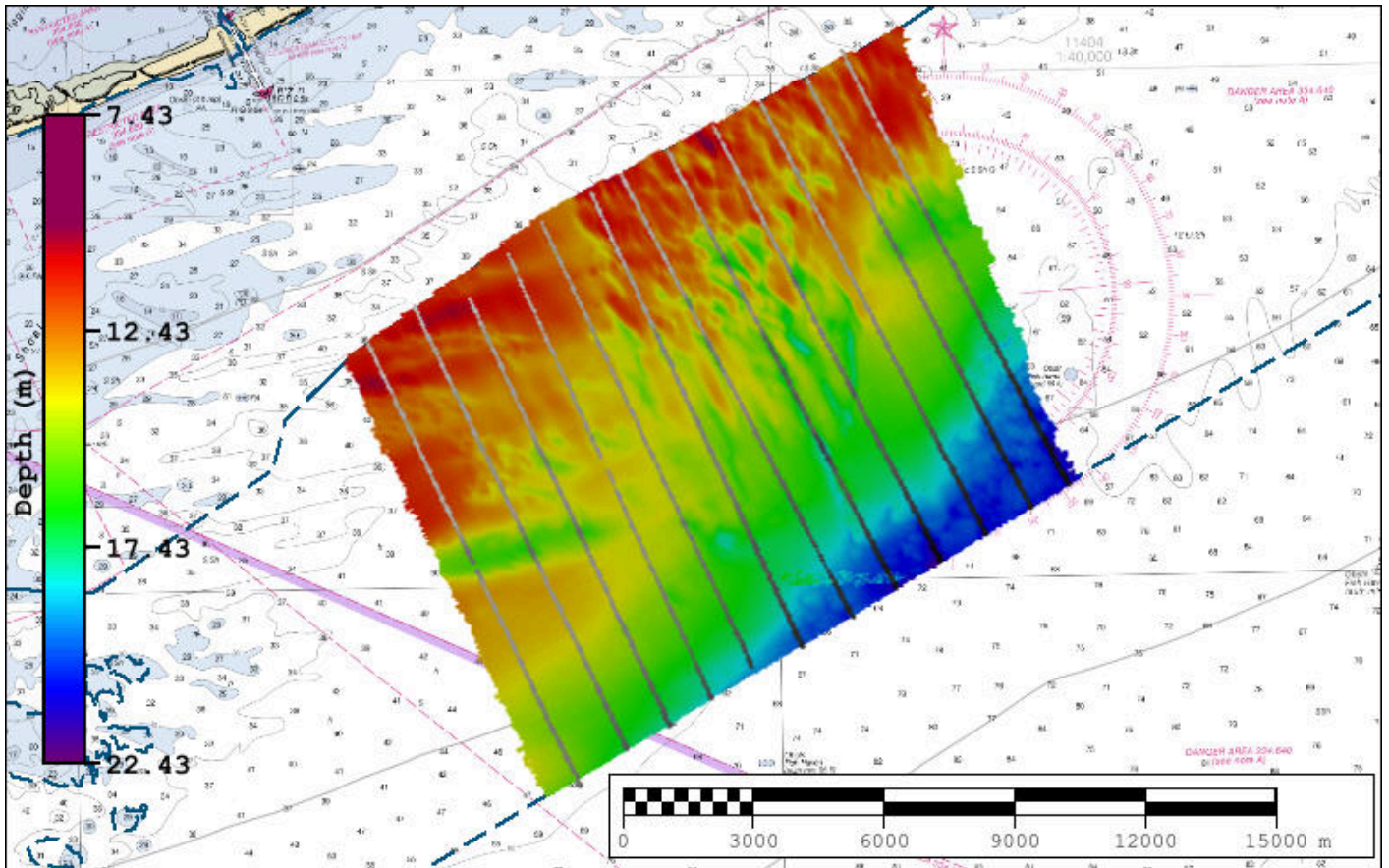
Figure 7: H13358 MBES mainscheme and MBES crossline distribution
