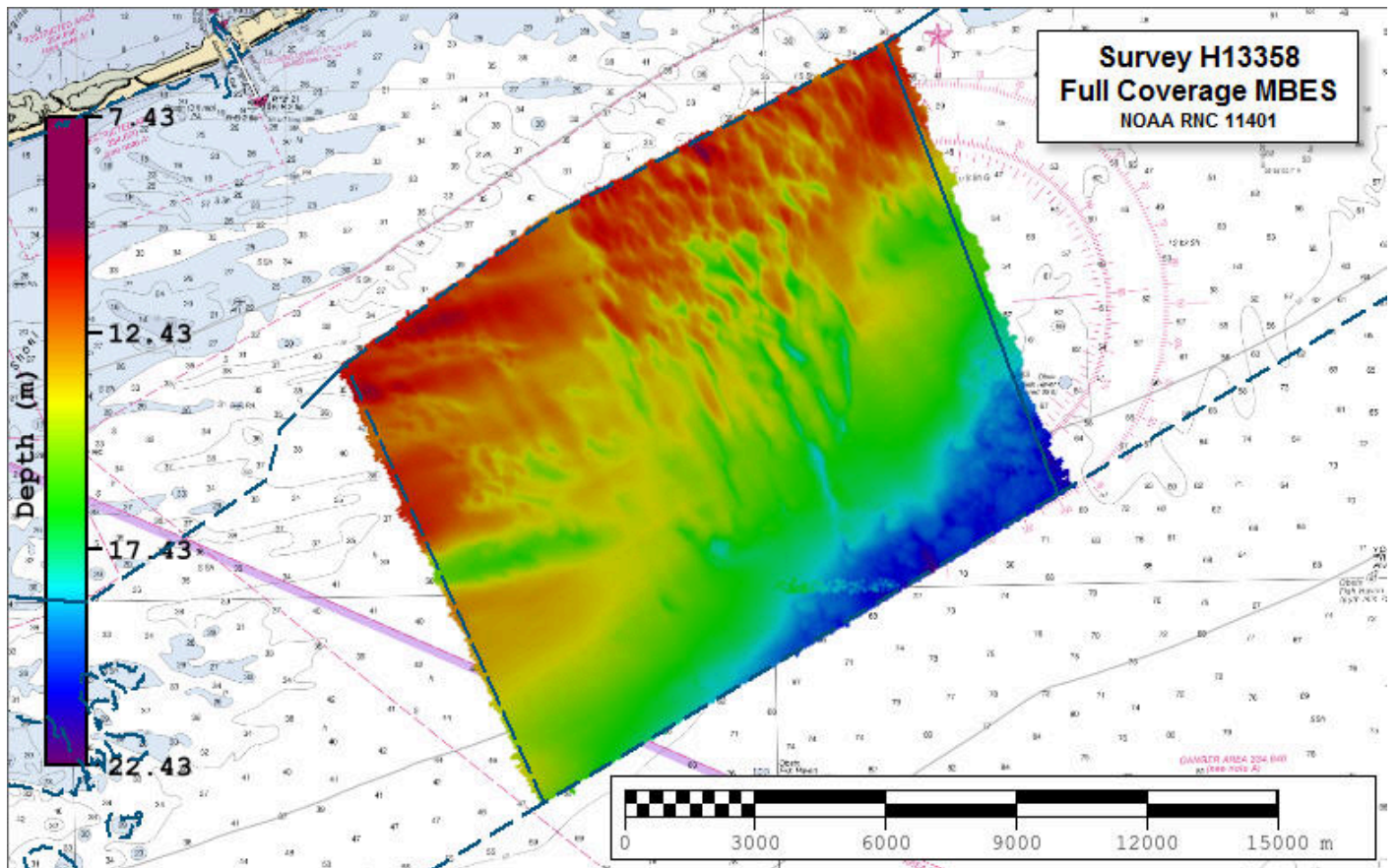
Figure 2: Survey H13358 complete coverage MBES
