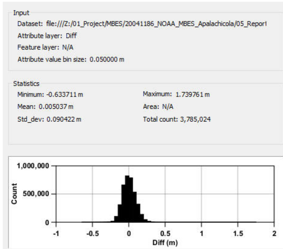
Figure 13: Survey H13358 junction with Survey H13359
