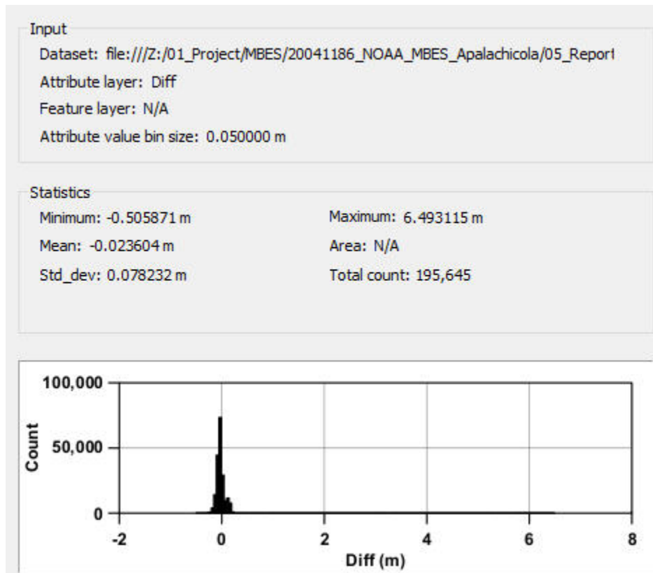
Figure 14: Survey H13358 junction with Survey H13361
