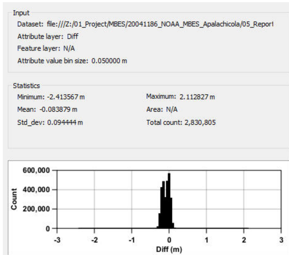
Figure 15: Survey H13358 junction with Survey H13287 (2019)
