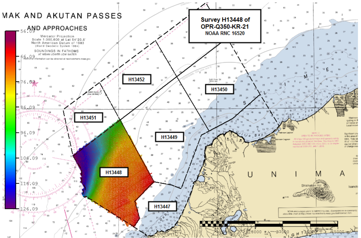
Figure 1: Survey H13448 relative to overall sheet limits of OPR-Q350-KR-21
