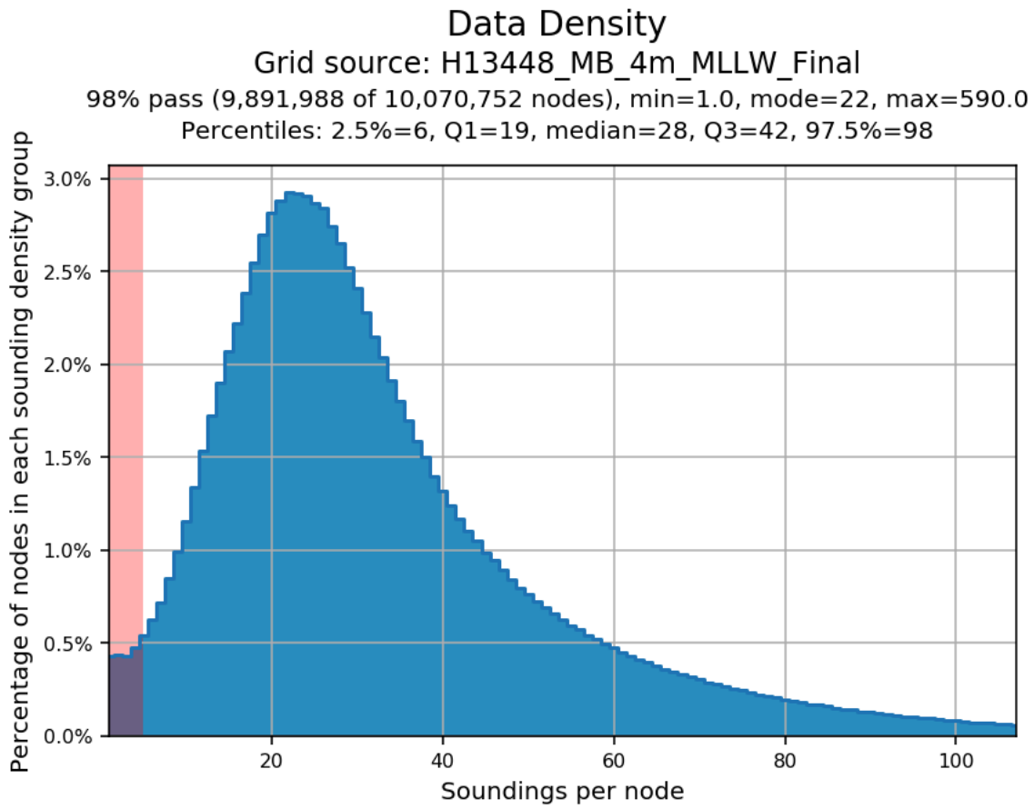
Figure 3: Survey H13448 4m finalized set line MBES density QC
