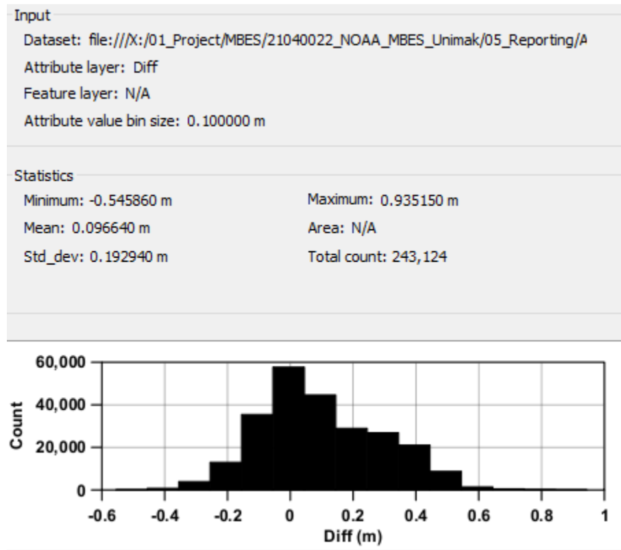
Figure 11: Survey H13448 junction with Survey H13447
