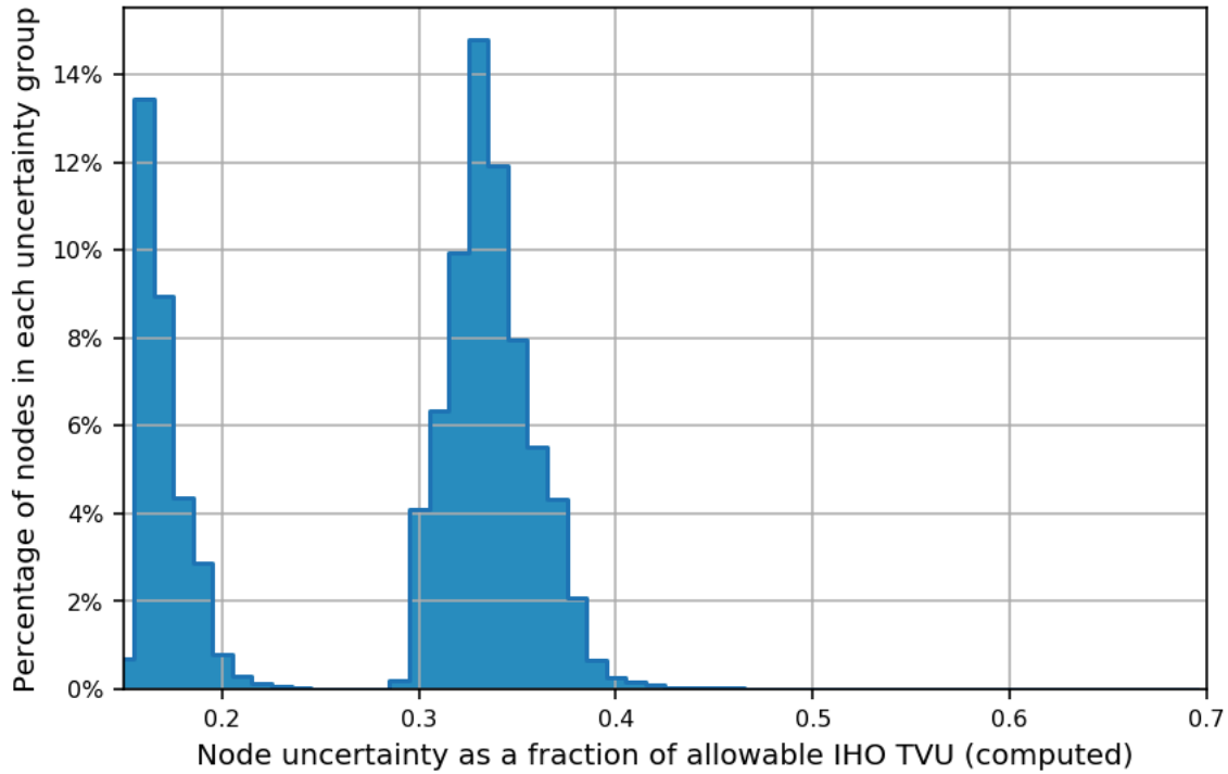
Figure 9: H13448 8m finalized grid TPU QC
