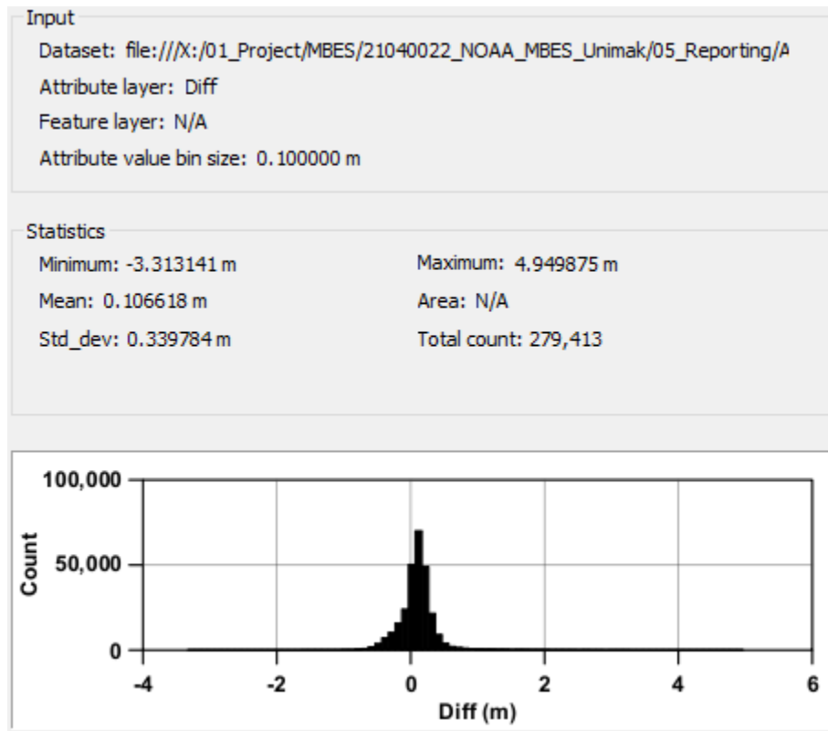
Figure 14: Survey H13448 junction with Survey H11644
