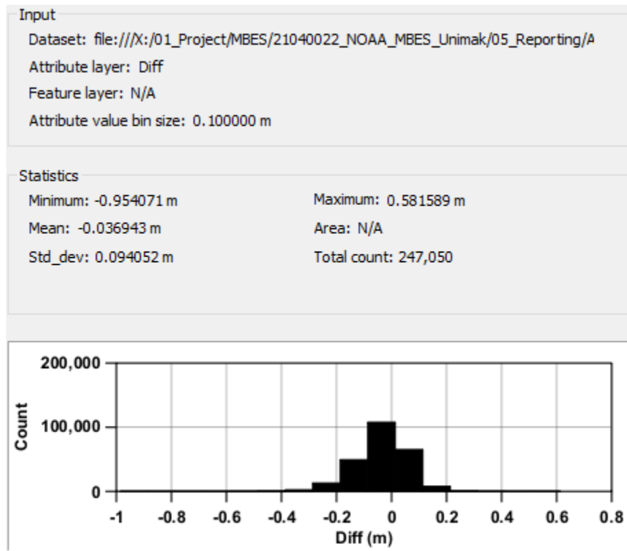
Figure 12: Survey H13448 junction with Survey H13449
