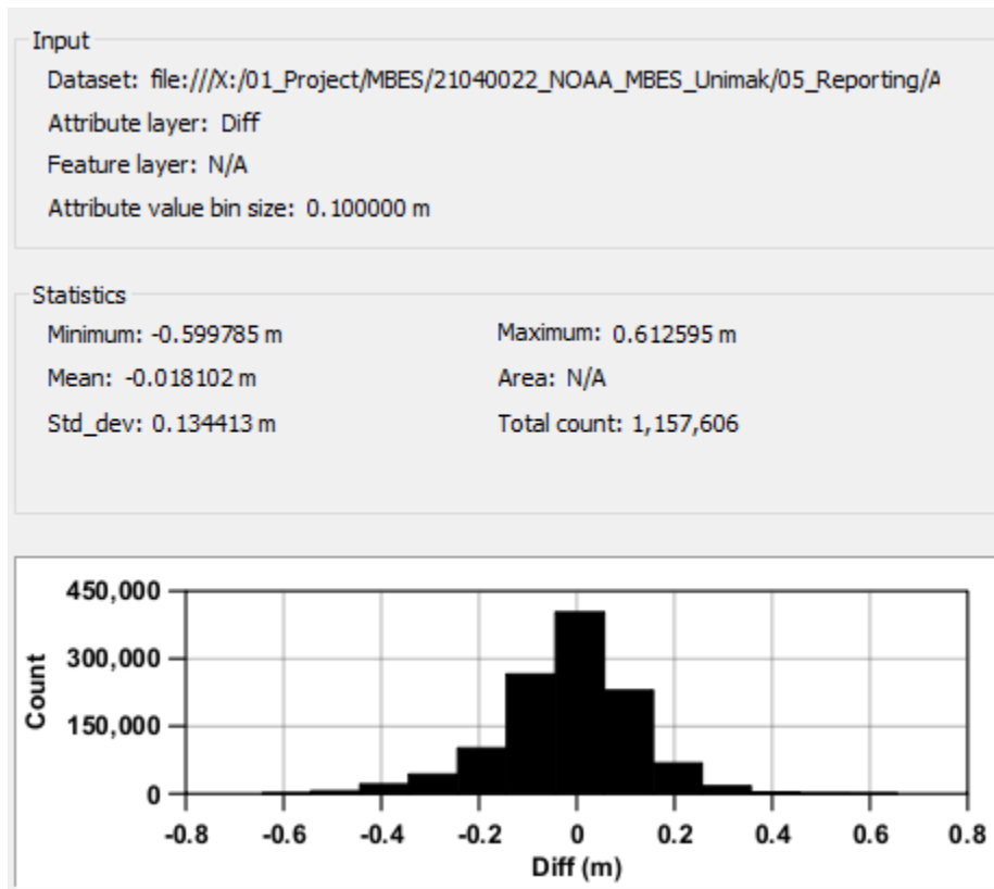
Figure 7: H13448 MBES mainscheme differenced from MBES crosslines statistical output
