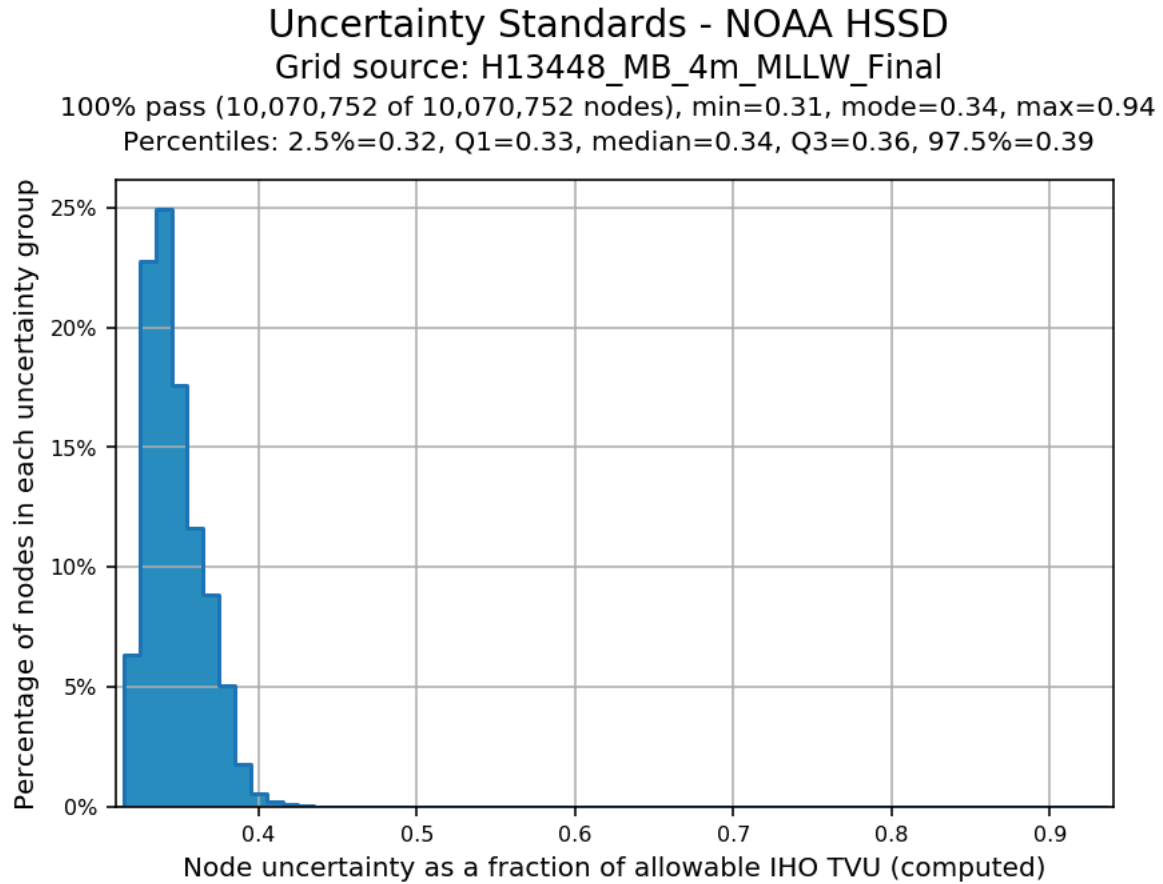
Figure 8: H13448 4m finalized grid TPU QC
