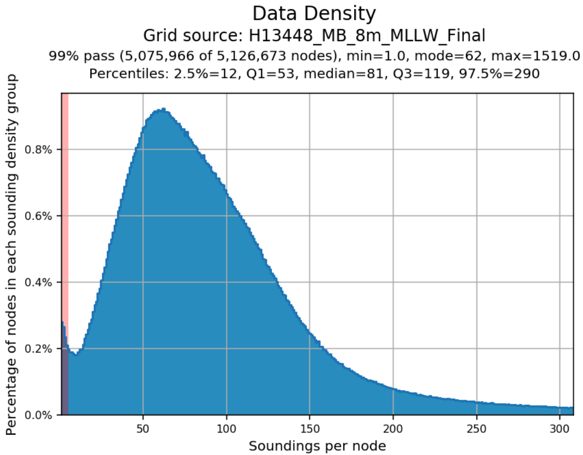
Figure 4: Survey H13448 8m finalized set line MBES density QC
