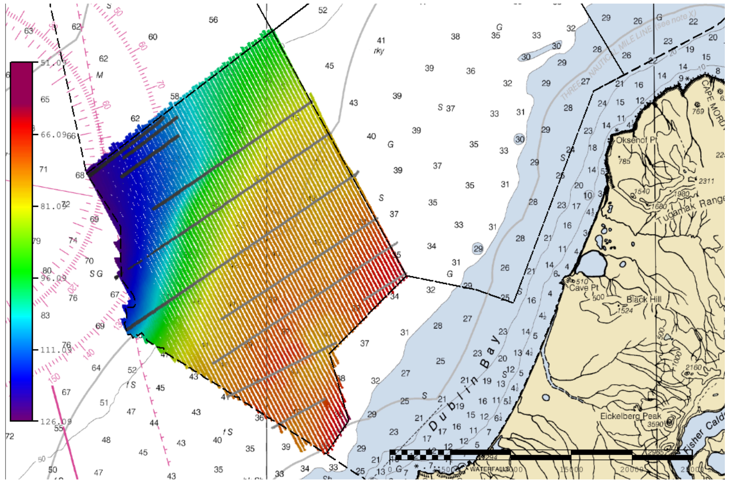
Figure 6: H13448 MBES mainscheme and MBES crossline distribution
