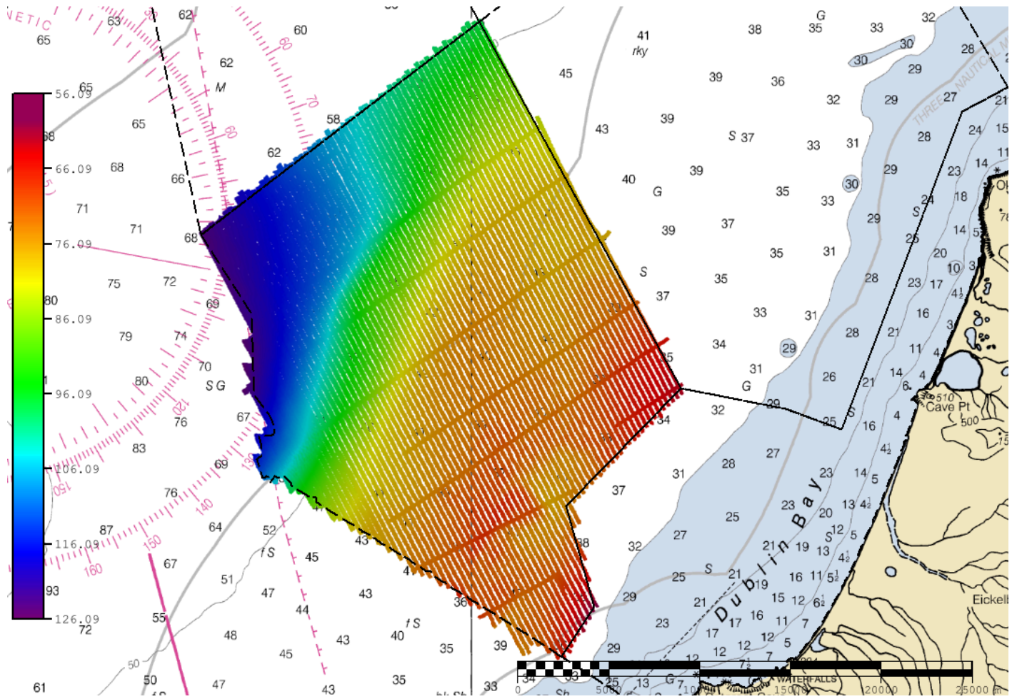
Figure 2: Survey H13448 MBES coverage
