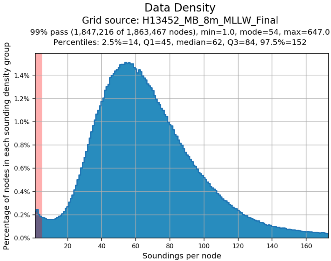
Figure 3: Survey H13452 8m finalized set line MBES density QC
