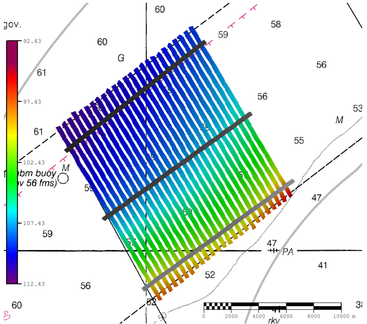
Figure 5: H13452 MBES mainscheme and MBES crossline distribution
