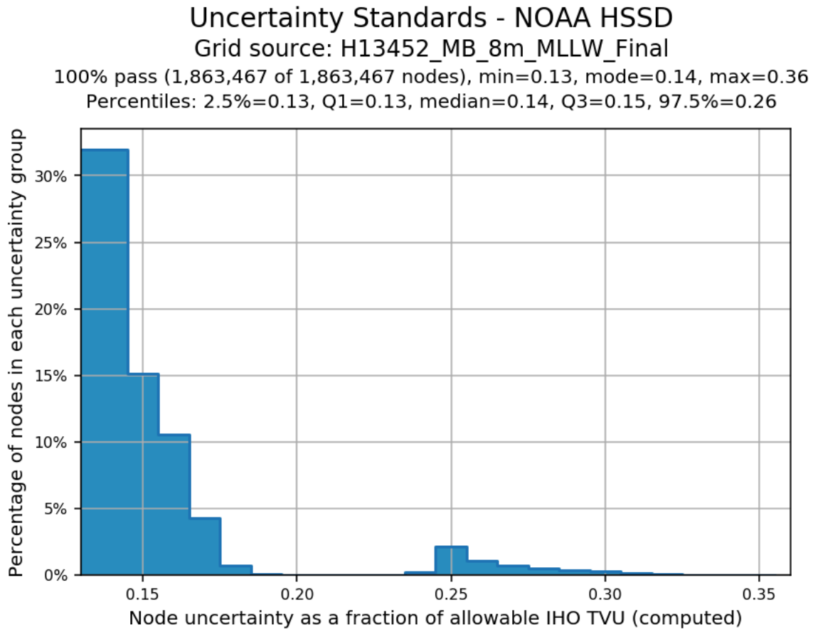
Figure 7: H13452 8m.finalized grid TPU QC
