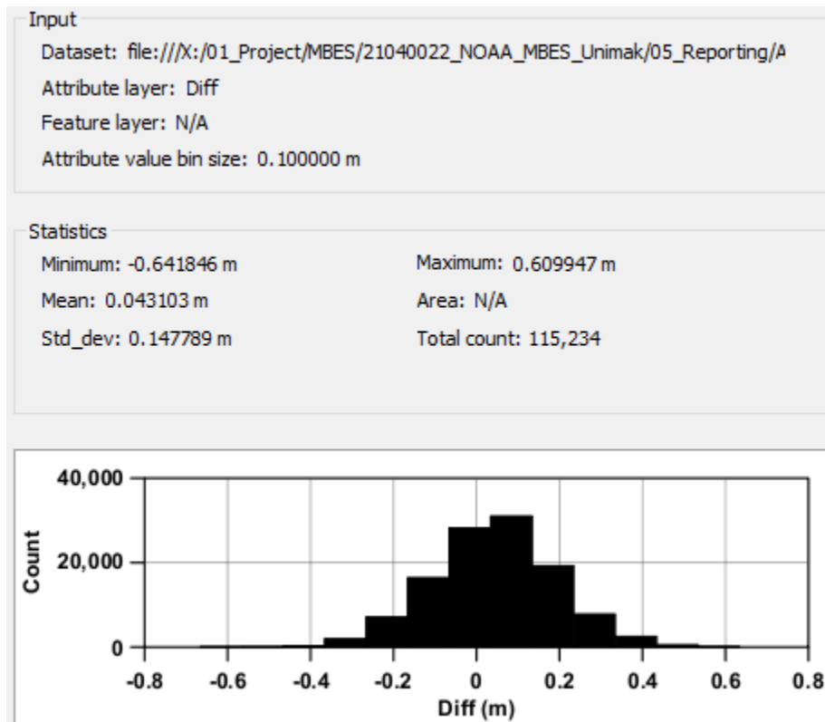
Figure 6: H13452 MBES mainscheme differenced from MBES crosslines statistical output
