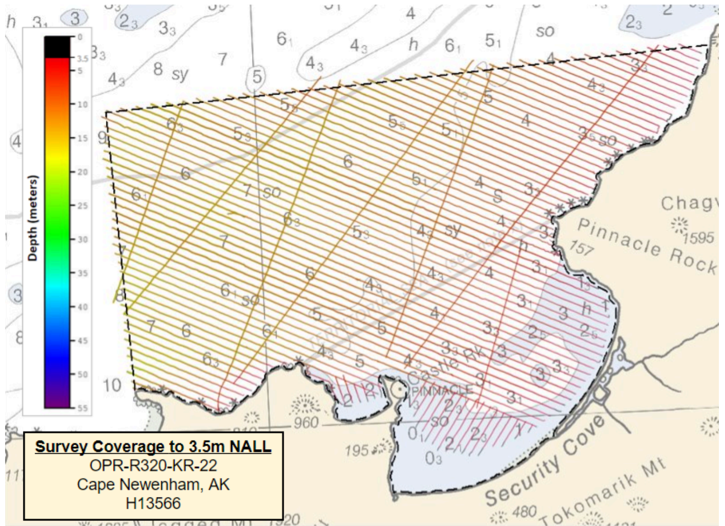
Figure 4: Survey Coverage with 3.5 NALL Displayed
