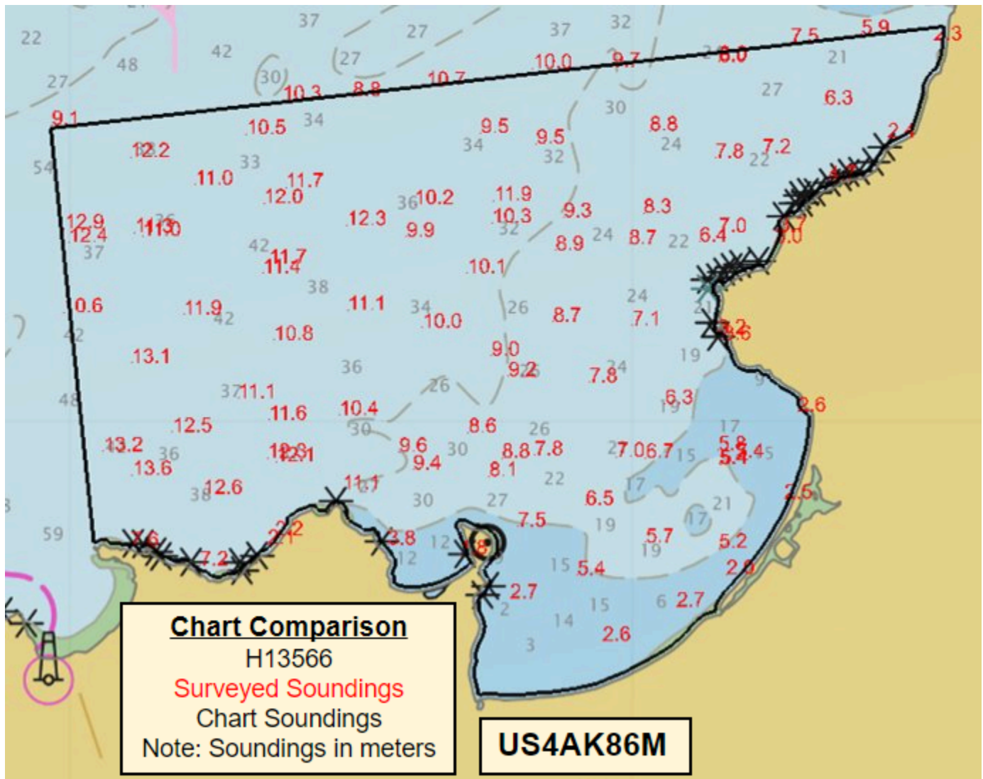
Figure 15: Generated Soundings used for Chart Comparison (US4AK86M)
