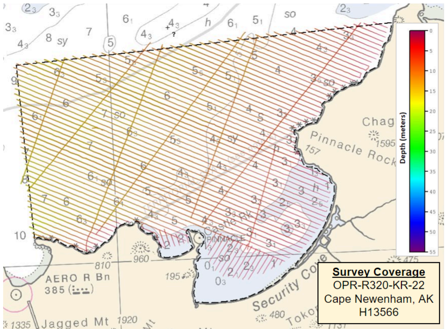
Figure 14: H13566 Finalized 4m CUBE Weighted Dynamic Surface Coverage
