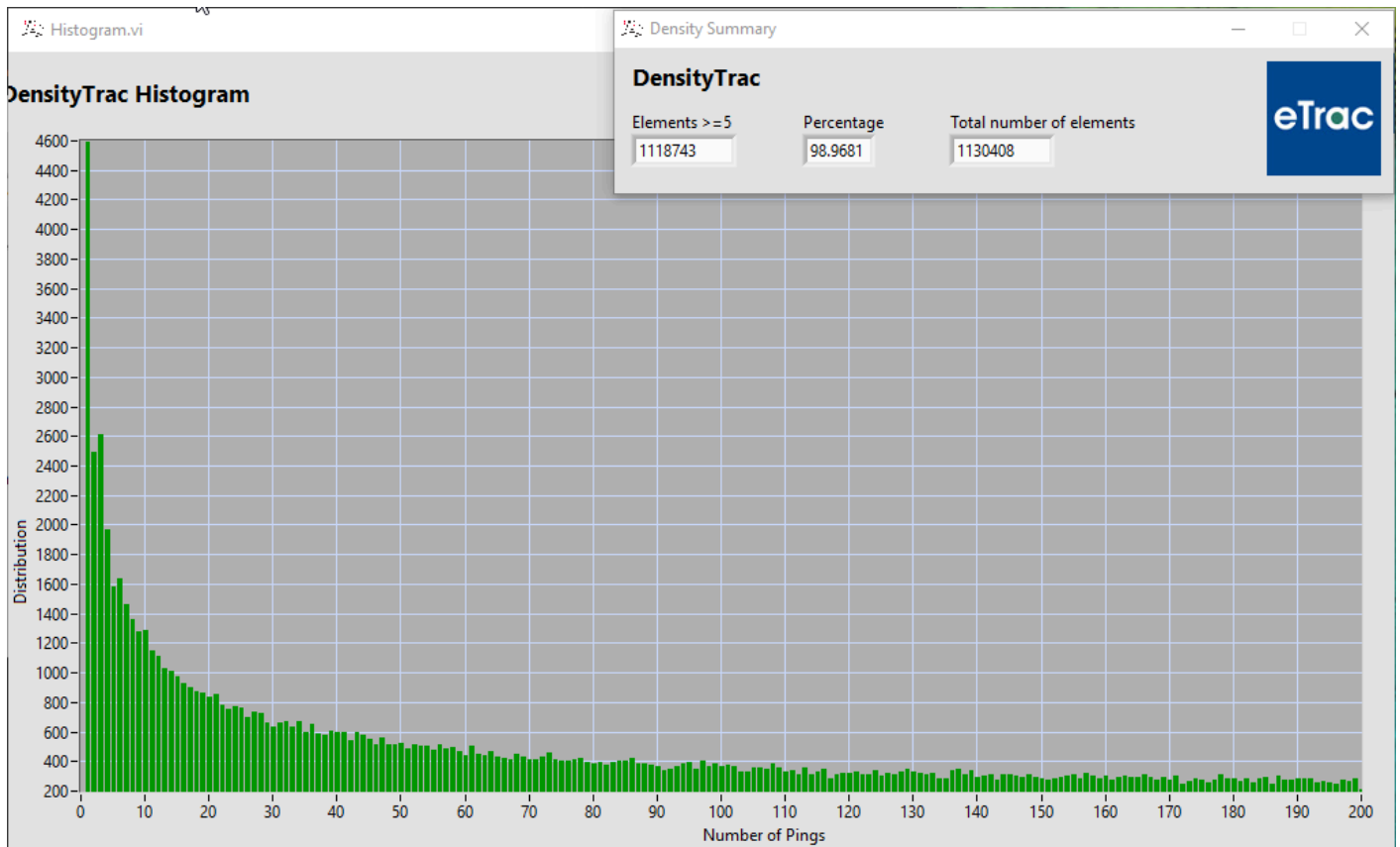
Figure 12: H13566 Finalized 4m Set Line Spacing MBES Density Distribution
