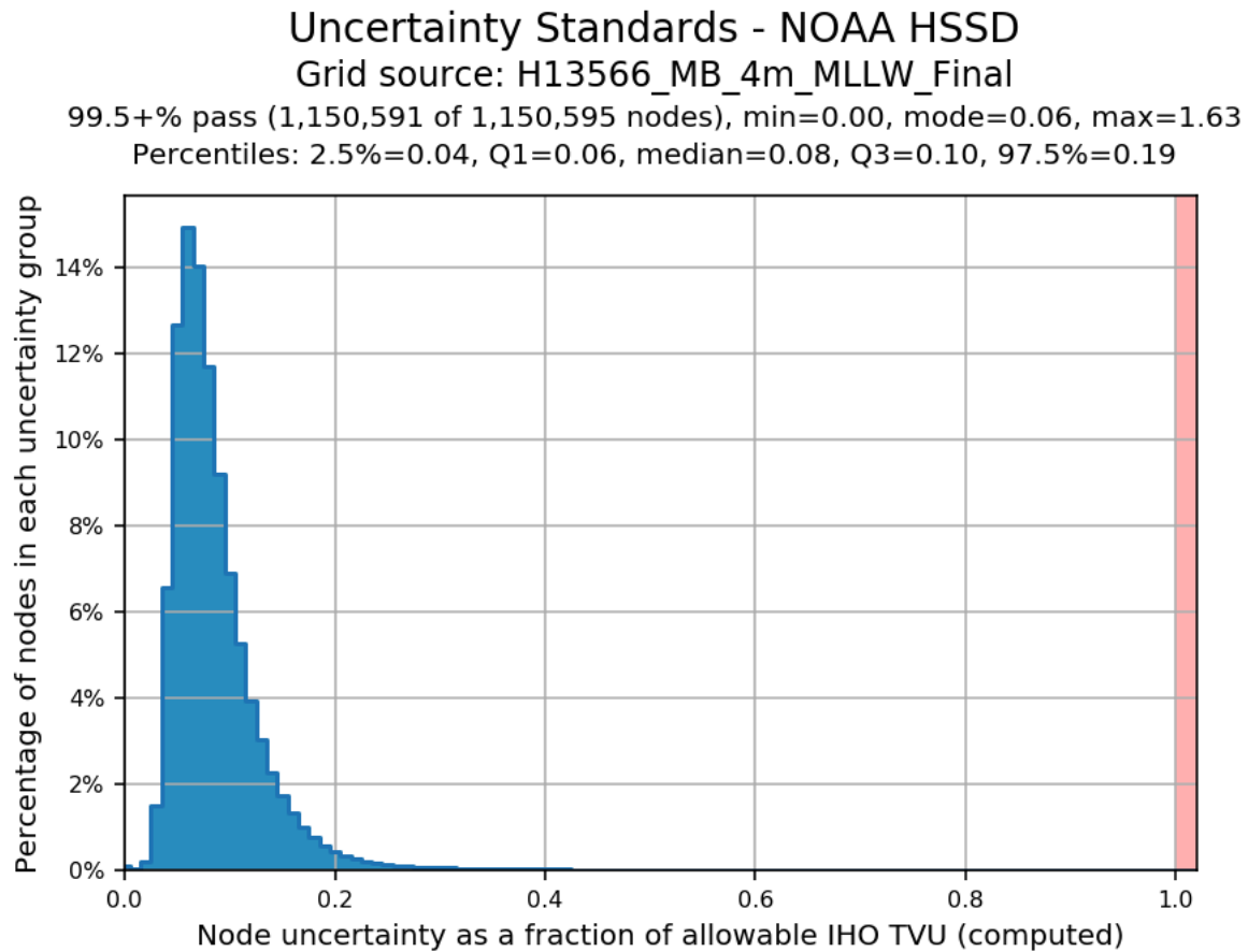
Figure 9: H13566 Finalized 4m Set Line Spacing MBES TVU Statistics
