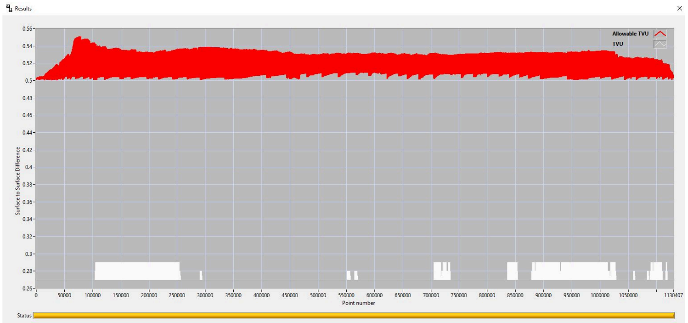
Figure 7: H13566 Finalized 4m Set Line Spacing MBES TVUTrac Results
