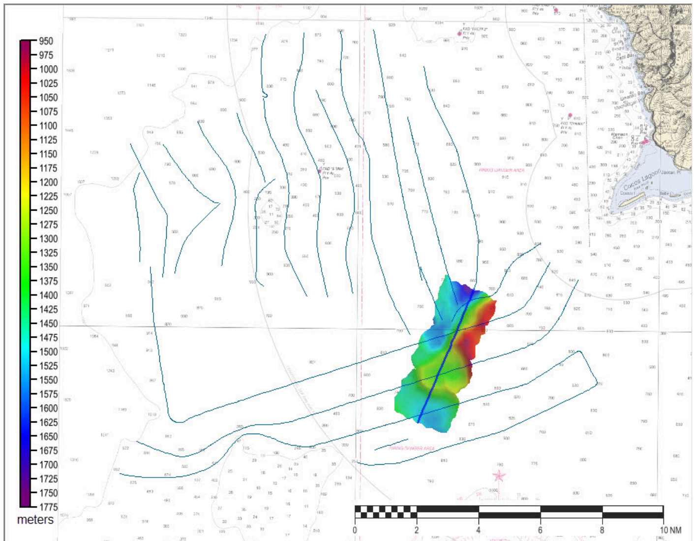
Figure 7: H13577 crossline surface overlaid on mainscheme tracklines.
