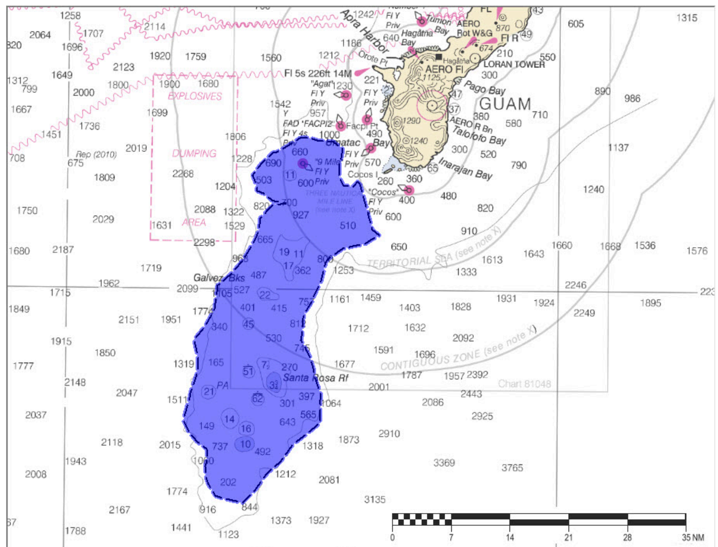
Figure 1: H13577 assigned survey area.
