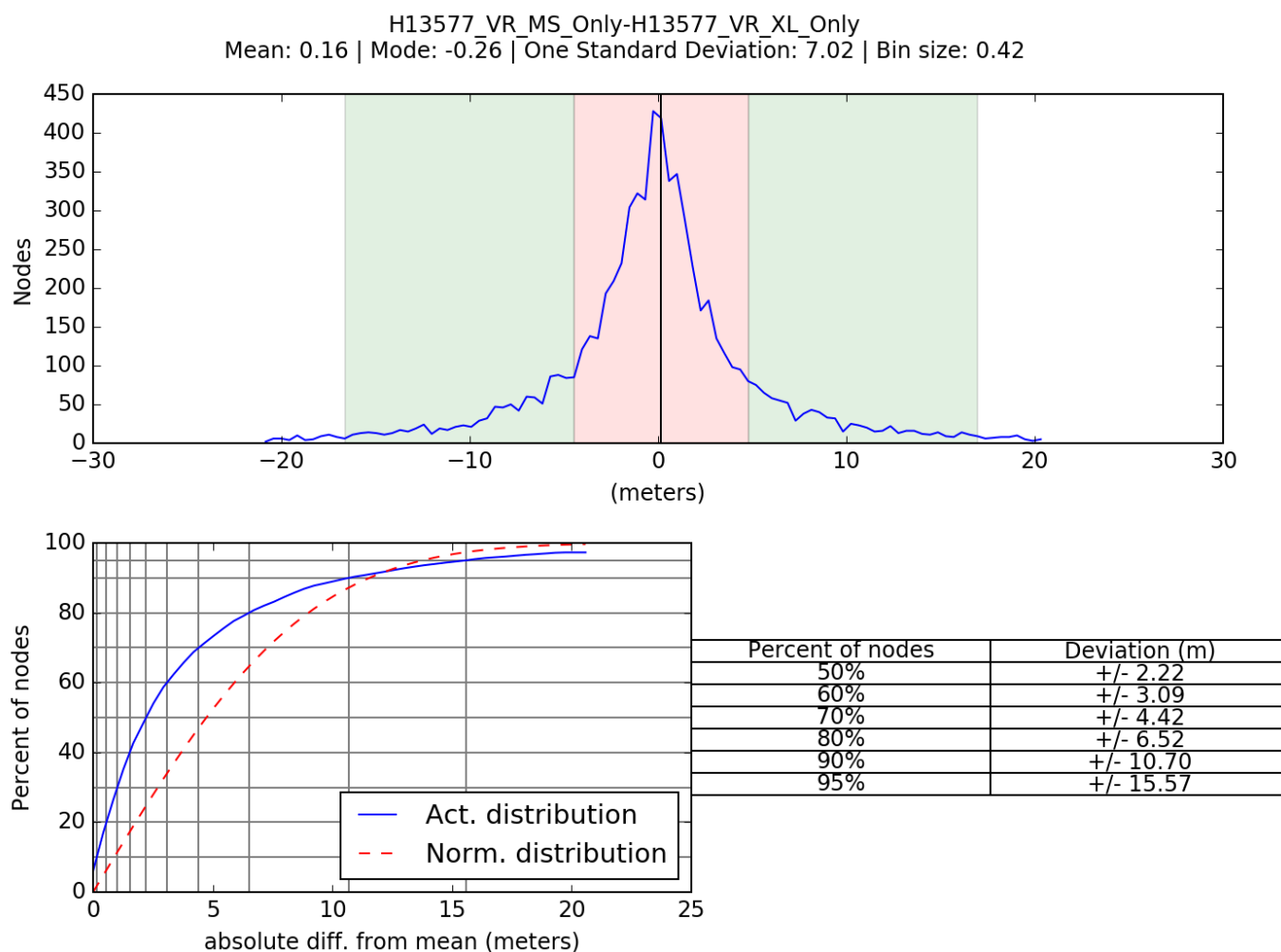
Figure 9: Pydro derived plot showing absolute difference statistics of H13577 mainscheme to crossline data.
