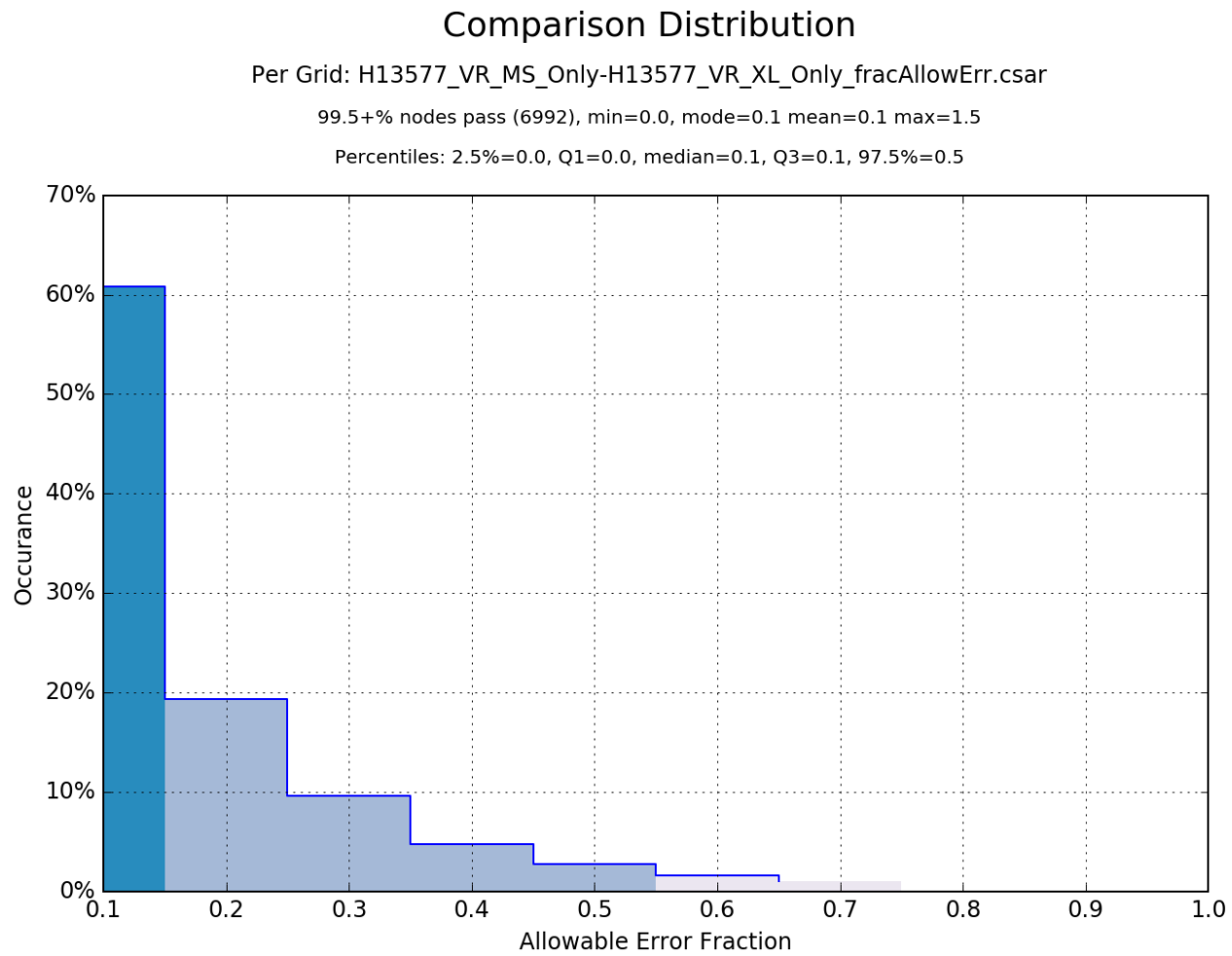
Figure 8: Pydro derived plot showing node percentage pass value of H13577 mainscheme to crossline data.
