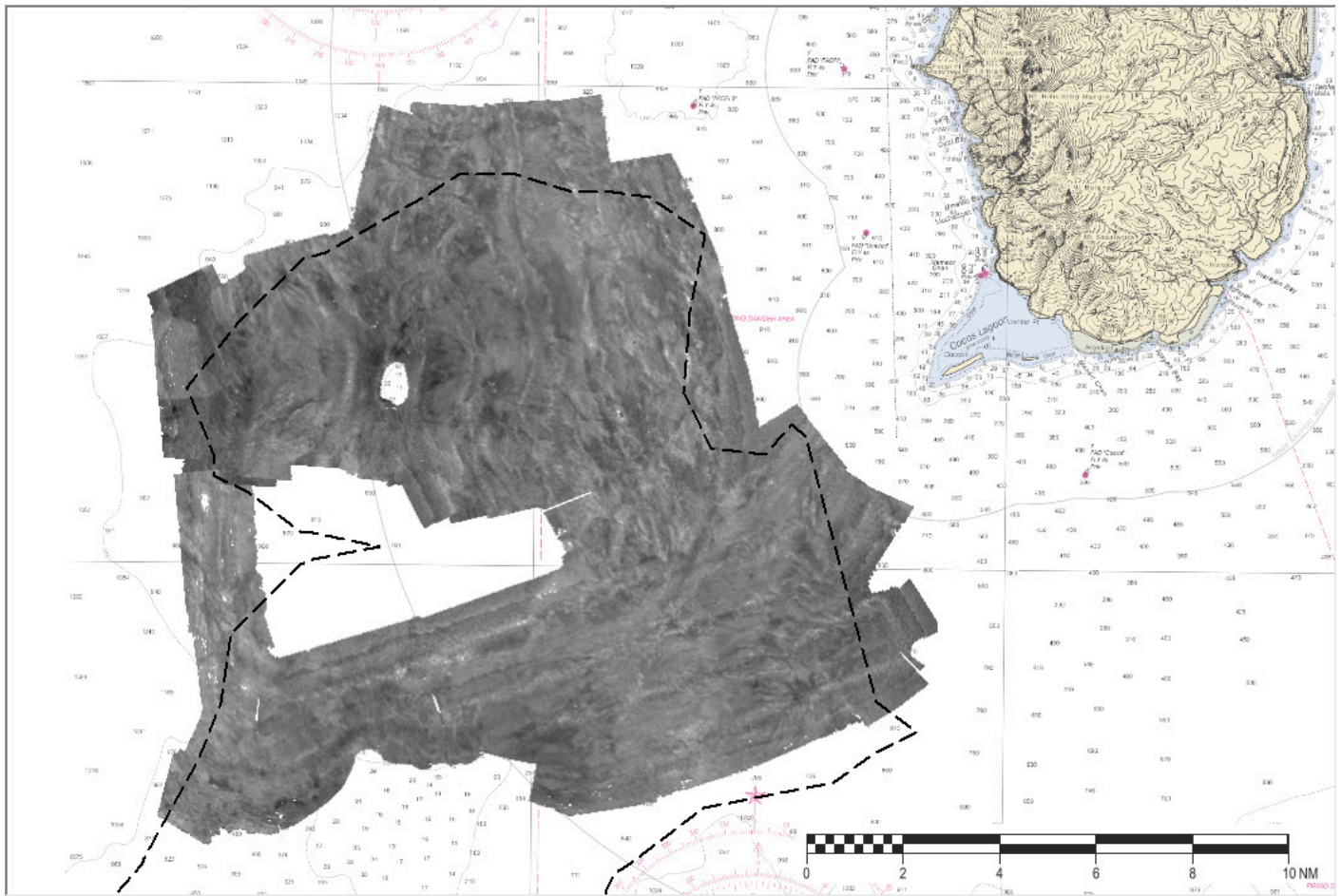
Figure 15: H13577 multibeam acoustic backscatter overview.
