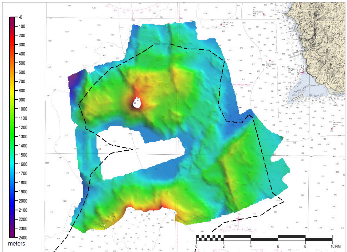
Figure 5: Acquired H13577 MBES coverage.
