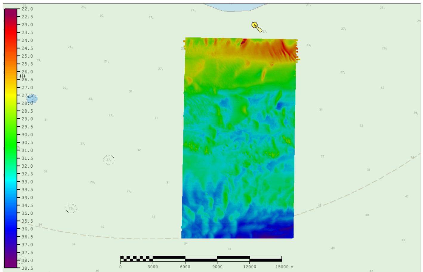
Figure 2: Survey coverage for H13600 (ENC US3SC10M).
