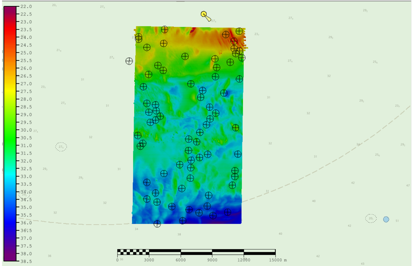
Figure 12: H13600 sound speed profile locations.
