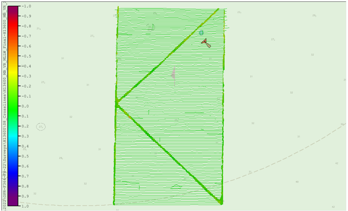
Figure 4: H13600 crossline surface overlaid on mainscheme tracklines.
