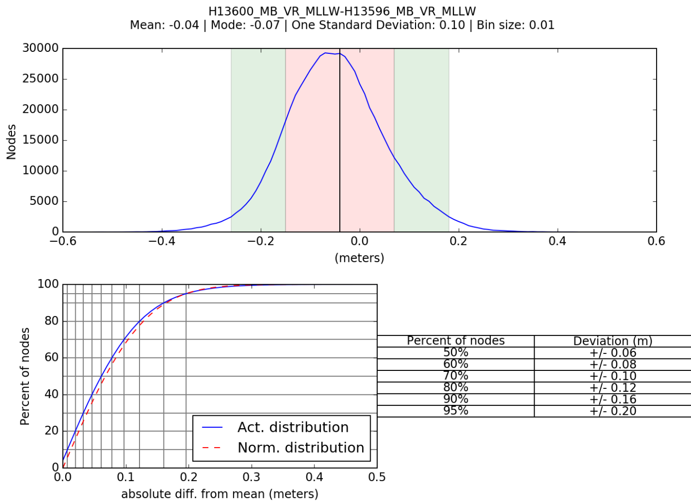
Figure 11: Pydro derived plot showing absolute difference statistics of H13600 and H13596
