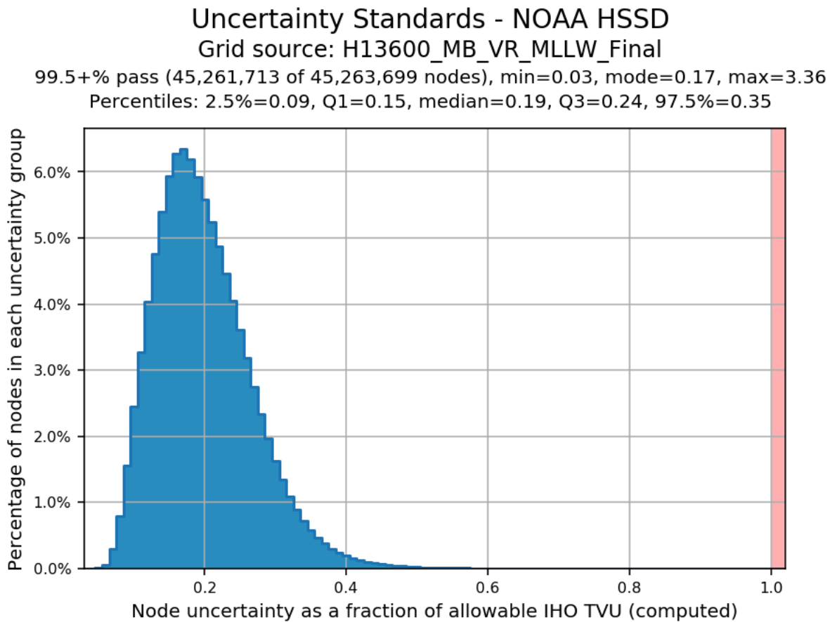
Figure 7: Pydro derived plot showing Total Vertical Uncertainty (TVU) compliance of H13600's finalized VR (Variable Resolution) surface.
