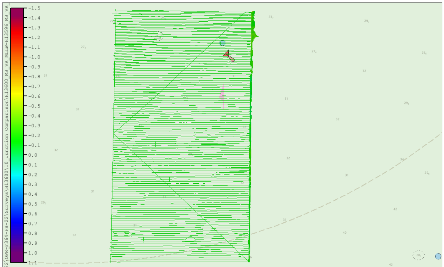
Figure 9: H13596 difference surface overlaid on H13600 tracklines.
