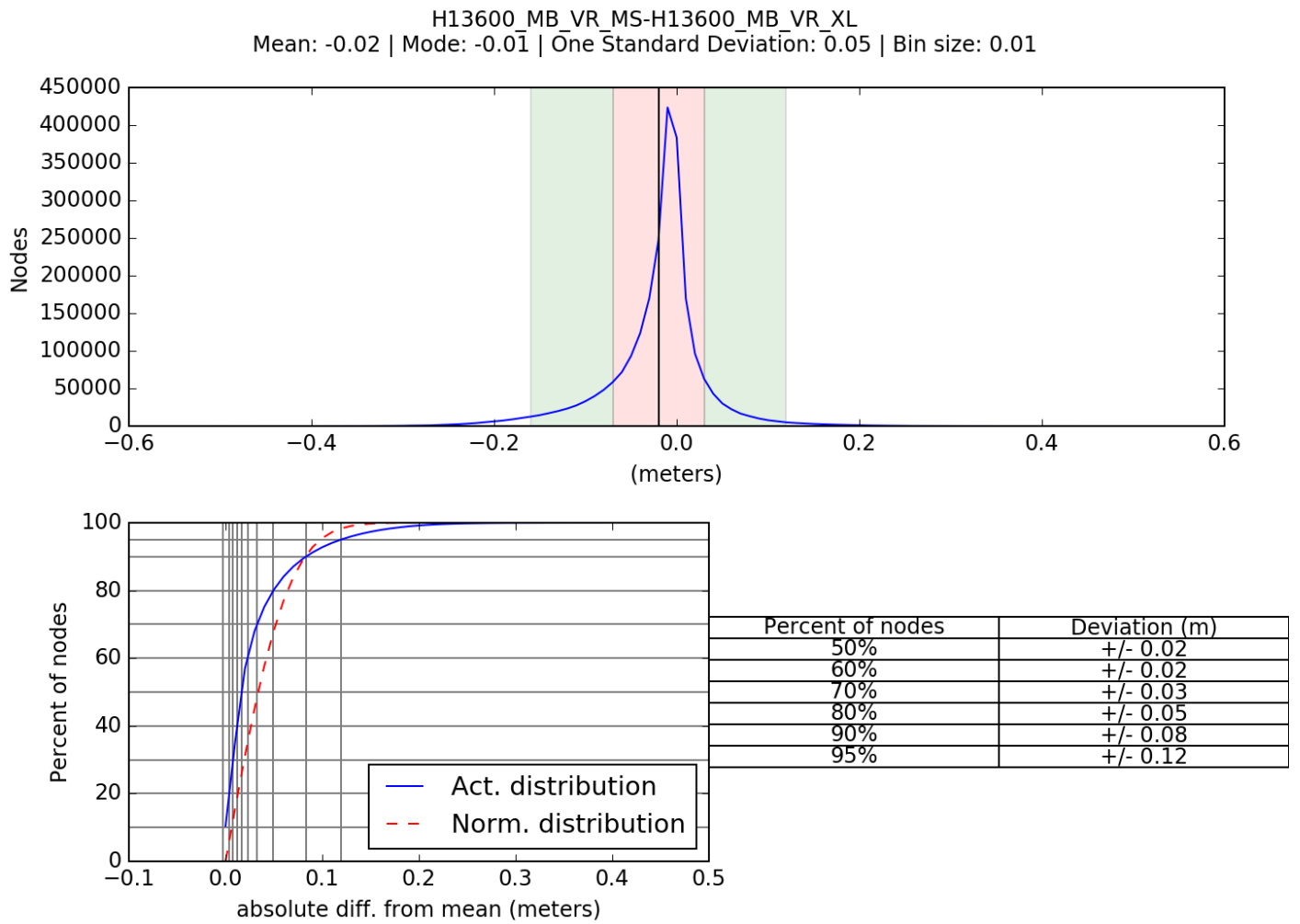
Figure 6: Pydro derived plot showing absolute difference statistics of H13600 mainscheme and crossline data.
