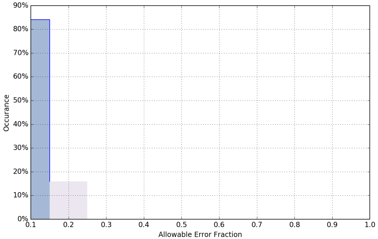
Figure 5: Pydro derived plot showing percentage-pass value of nodes in H13600 mainscheme and crossline data.
