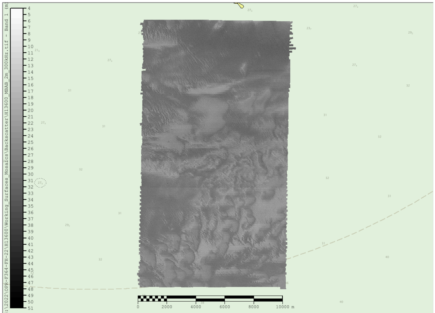
Figure 13: Overview of H13600 backscatter mosaic.
