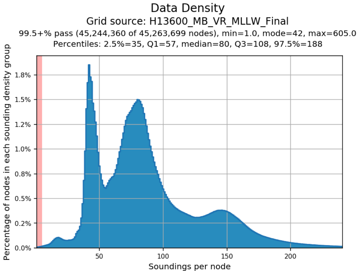
Figure 14: Pydro derived plot showing HSSD density compliance of H13600 finalized variable-resolution surface.
