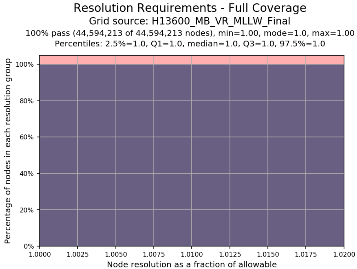
Figure 15: Pydro derived plot showing HSSD resolution compliance of H13600 finalized variable-resolution surface.
