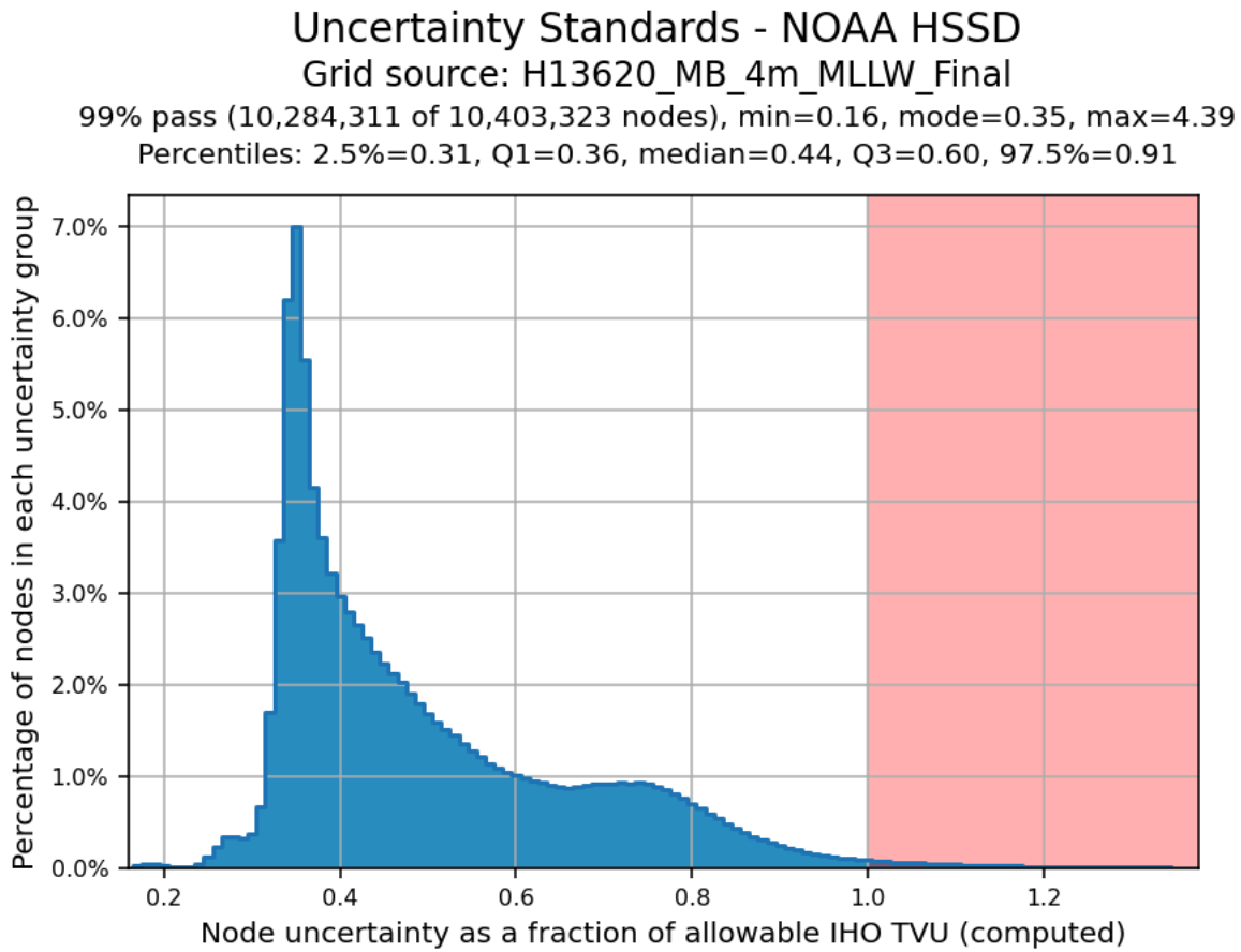
Figure 2: H13620 4m grid allowable uncertainty statistics.
