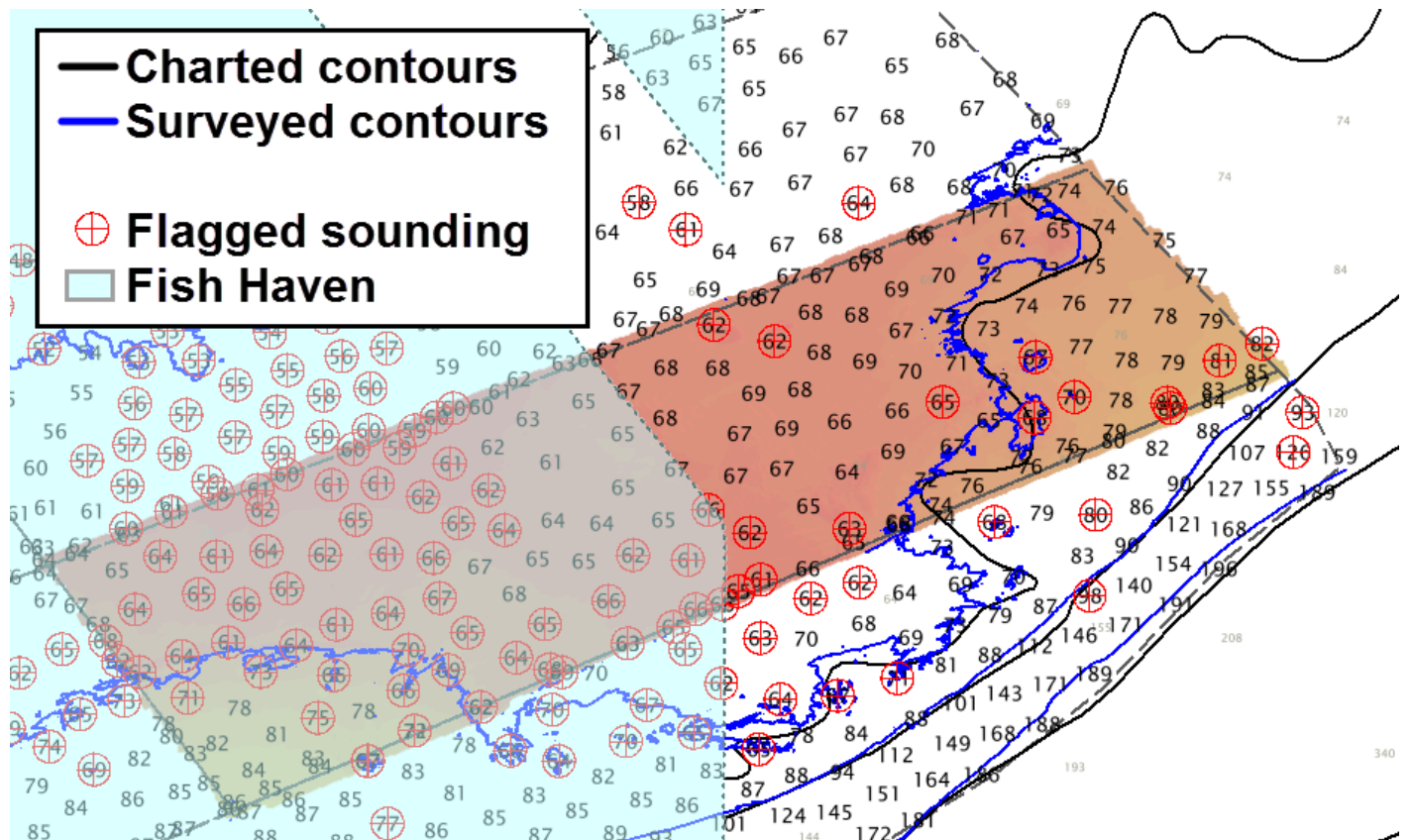
Figure 10: Comparison of charted vs. surveyed depths. Soundings in meters.
