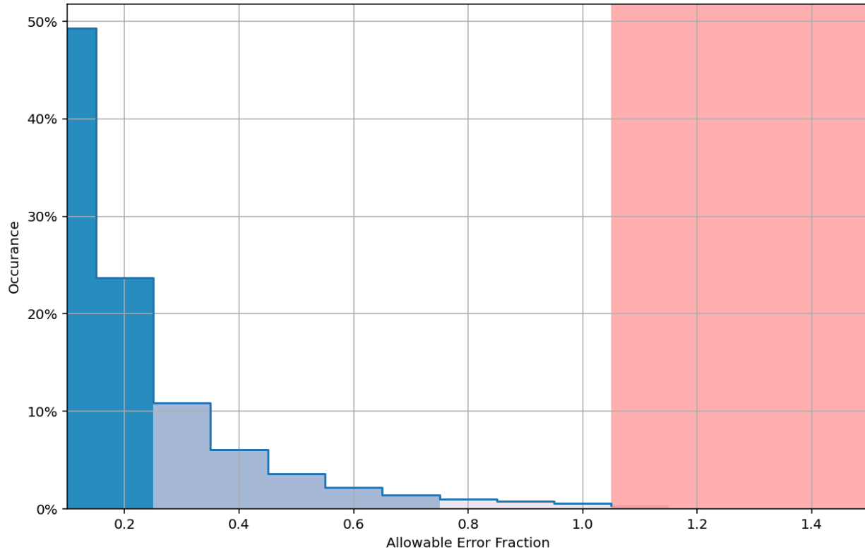
Figure 9: H13620 Crossline comparison distribution of nodes with an allowable error fraction.
