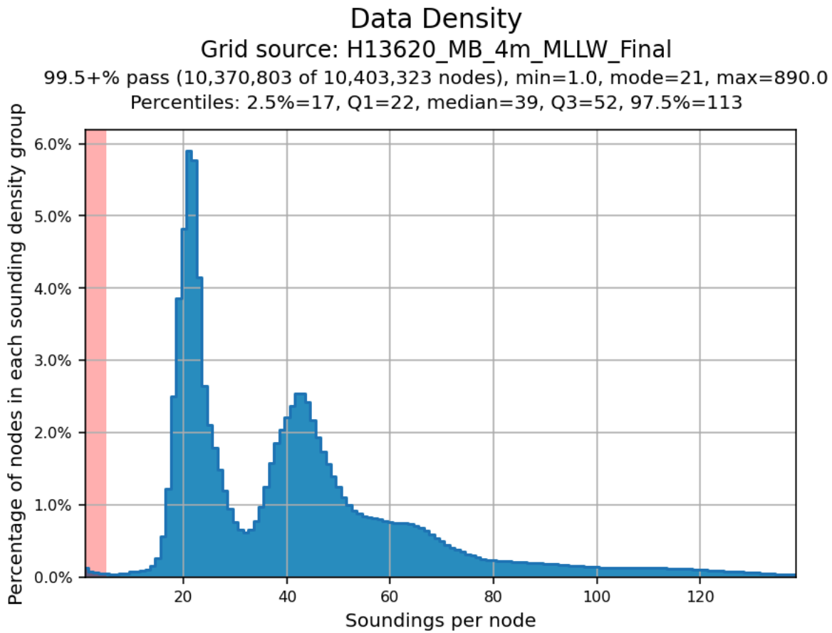
Figure 3: H13620 4m grid data density statistics.
