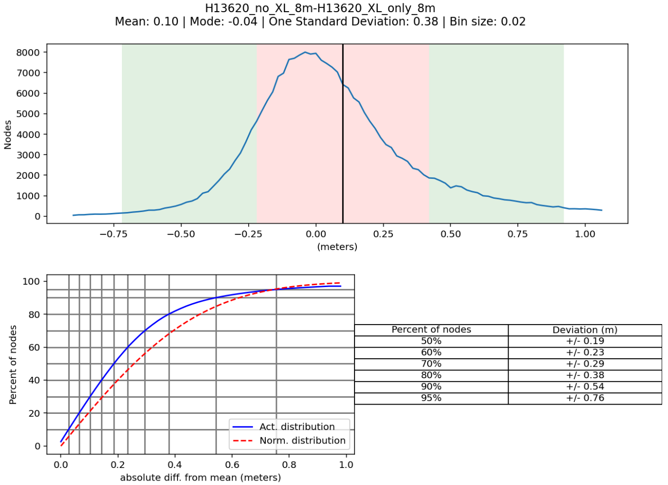
Figure 8: H13620 Distribution of depth difference values (m) calculated between crossline and mainscheme grids.
