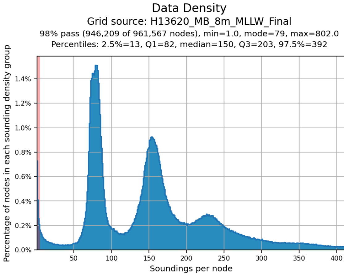
Figure 5: H13620 8m grid data density statistics.
