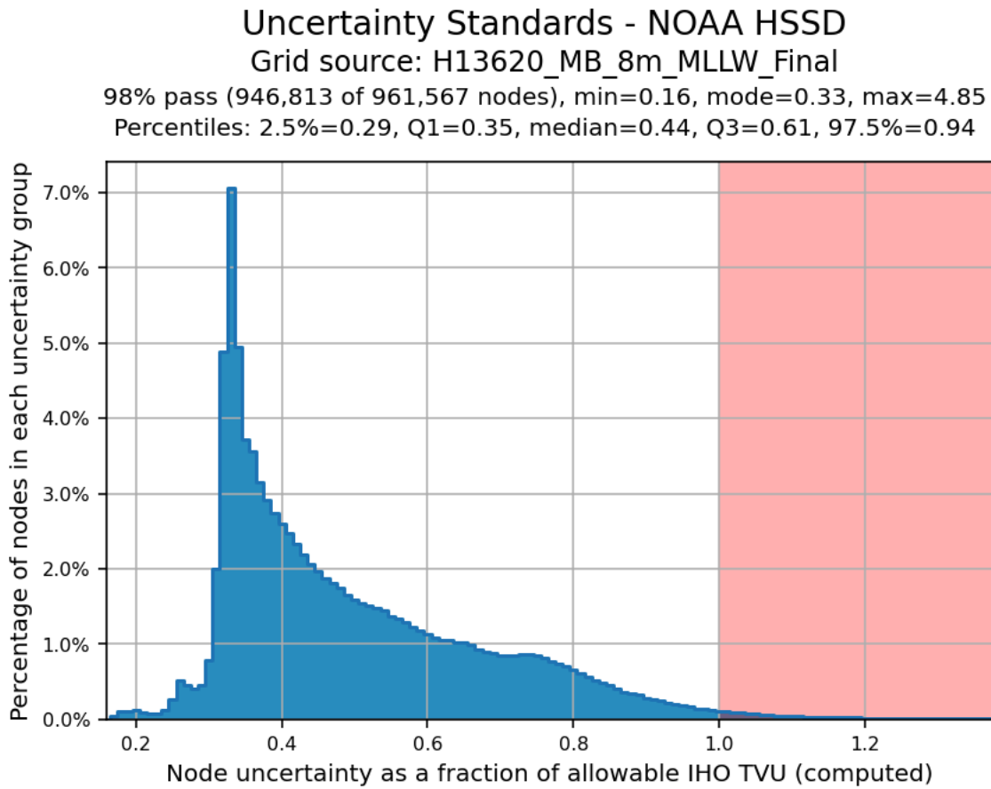
Figure 4: H13620 8m grid allowable uncertainty statistics.
