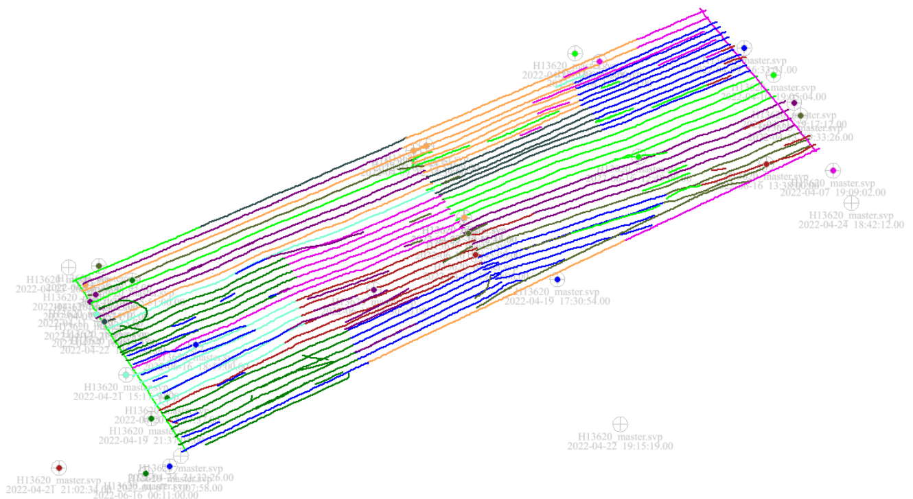
Figure 11: Distribution of SVP casts and application to survey lines.
