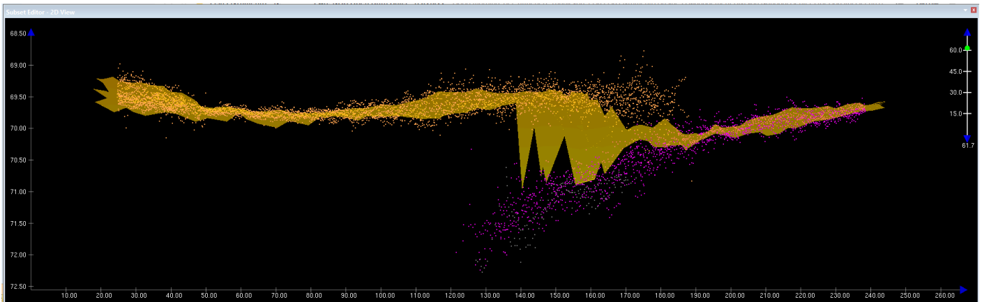
Figure 13: Downward curvature of swath outer edge, with CUBE reference surface overlaid.
