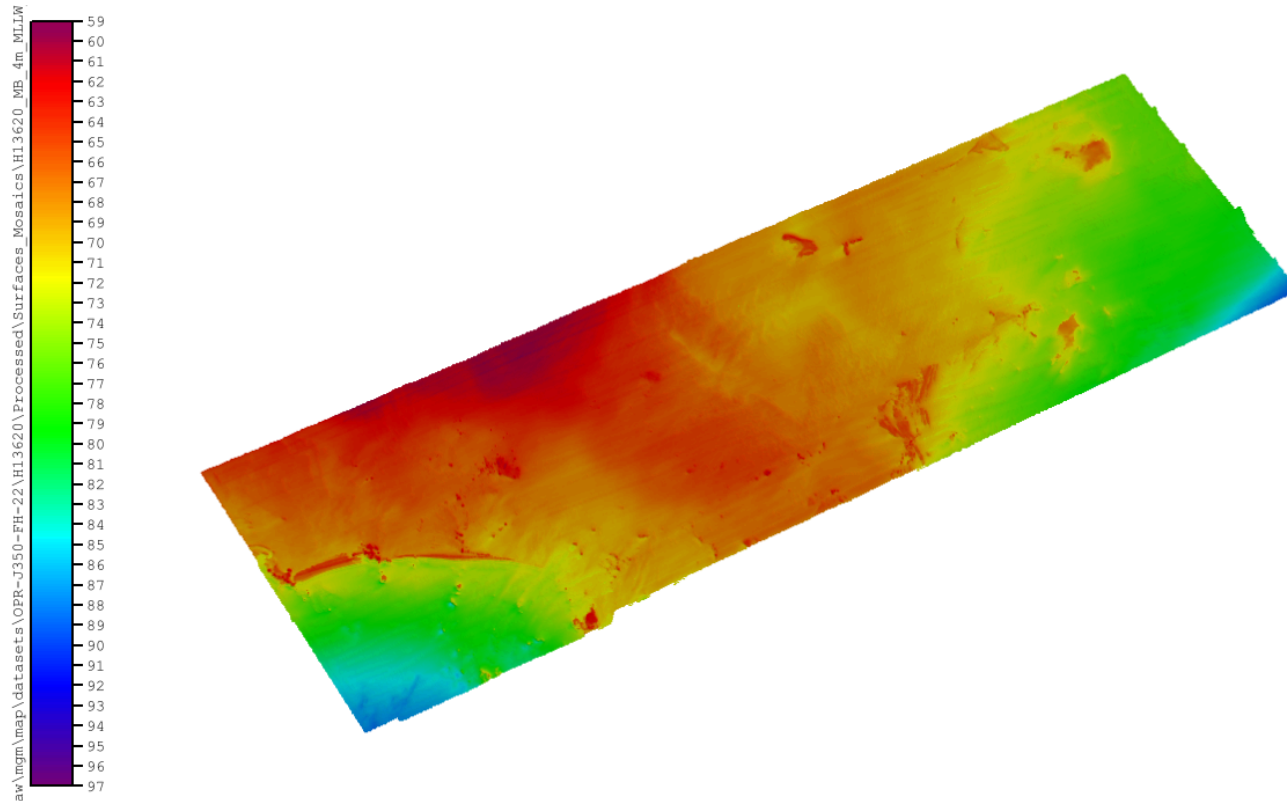
Figure 6: H13620 Coverage overview of combined 4m and 8m resolution CUBE grids.
