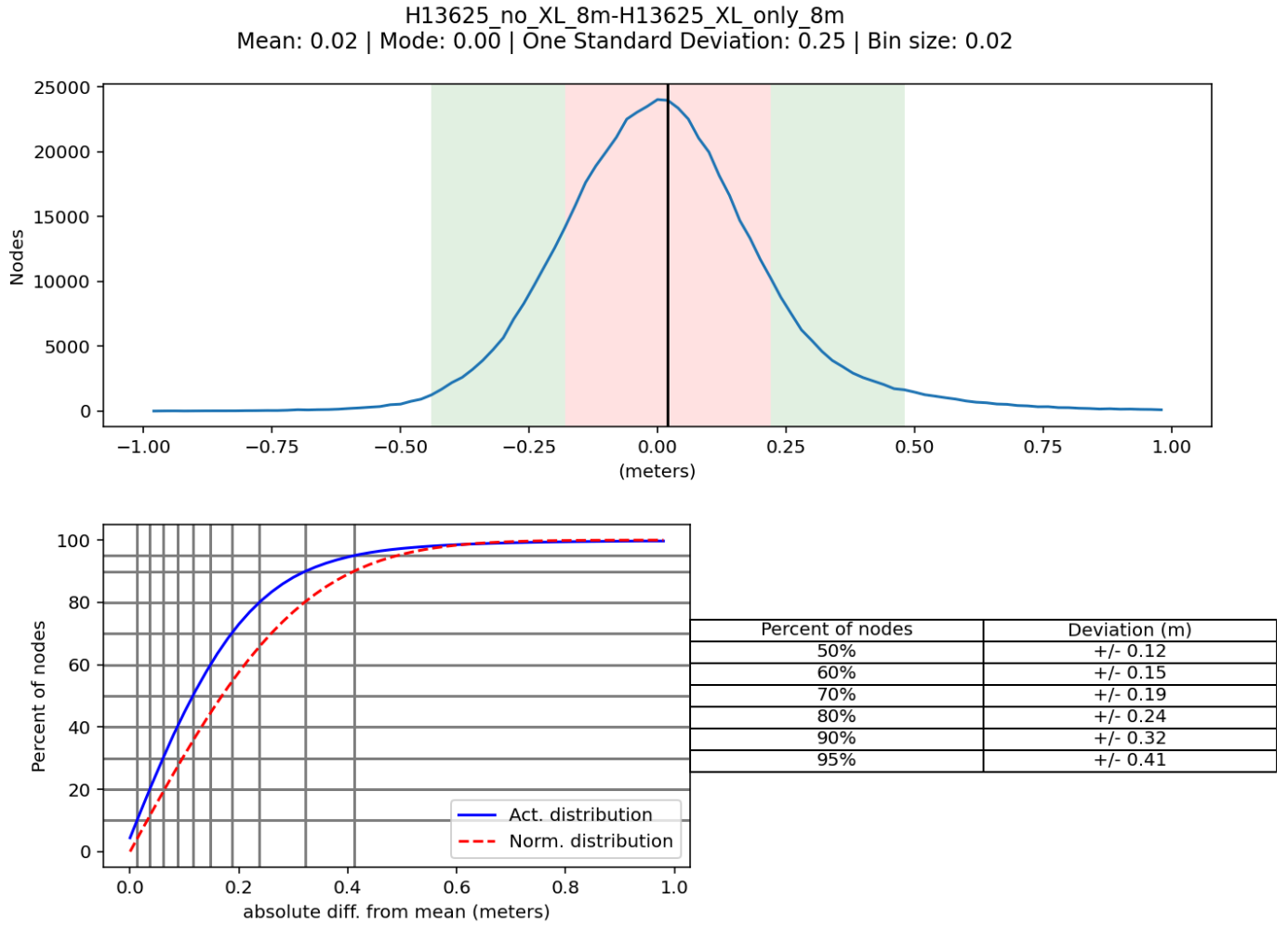
Figure 9: H13625 Distribution of depth difference values (m) calculated between crossline and mainscheme grids.
