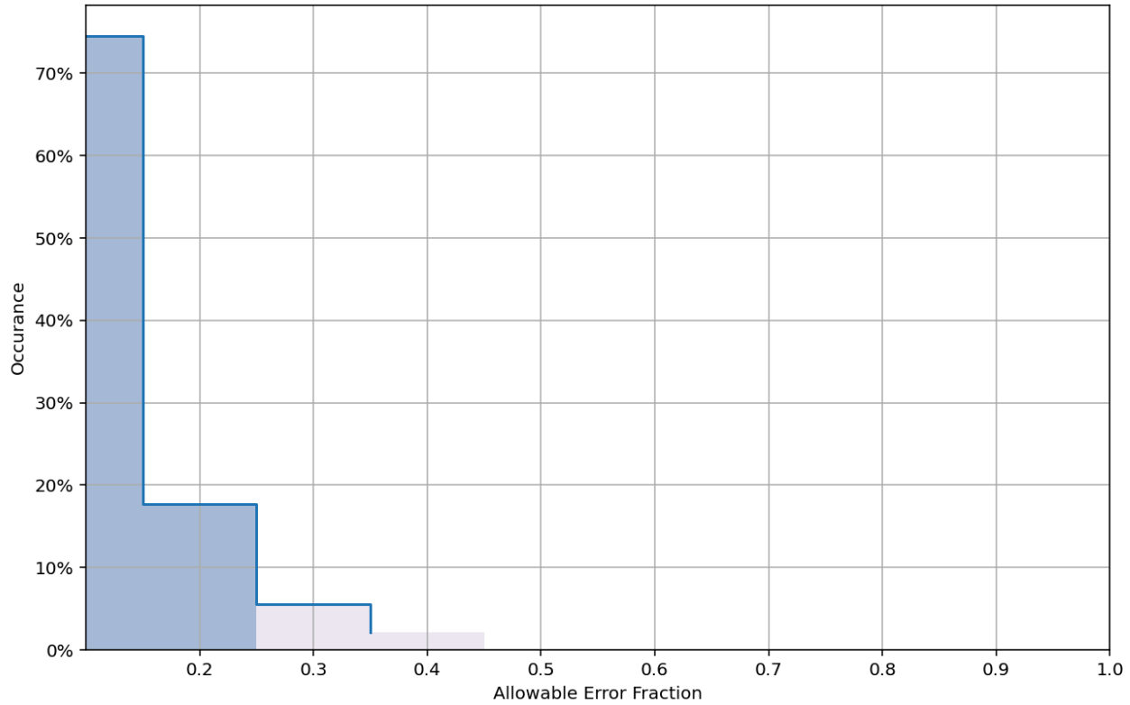
Figure 10: H13625 Crossline comparison distribution of nodes with an allowable error fraction.
