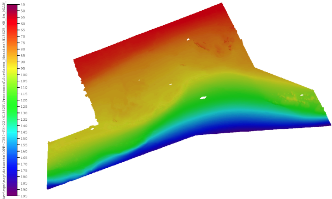
Figure 6: H13625 Coverage overview of combined 4m and 8m resolution CUBE grids.
