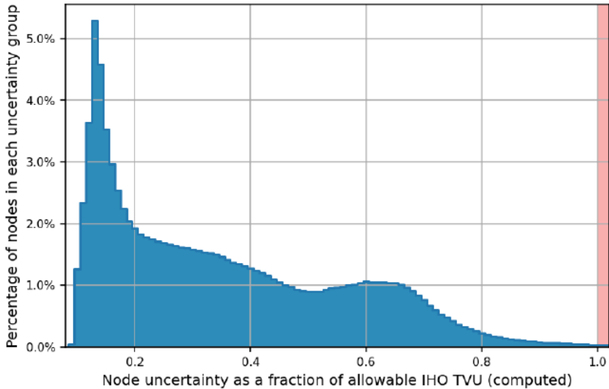
Figure 2: H13625 4m grid allowable uncertainty statistics.
