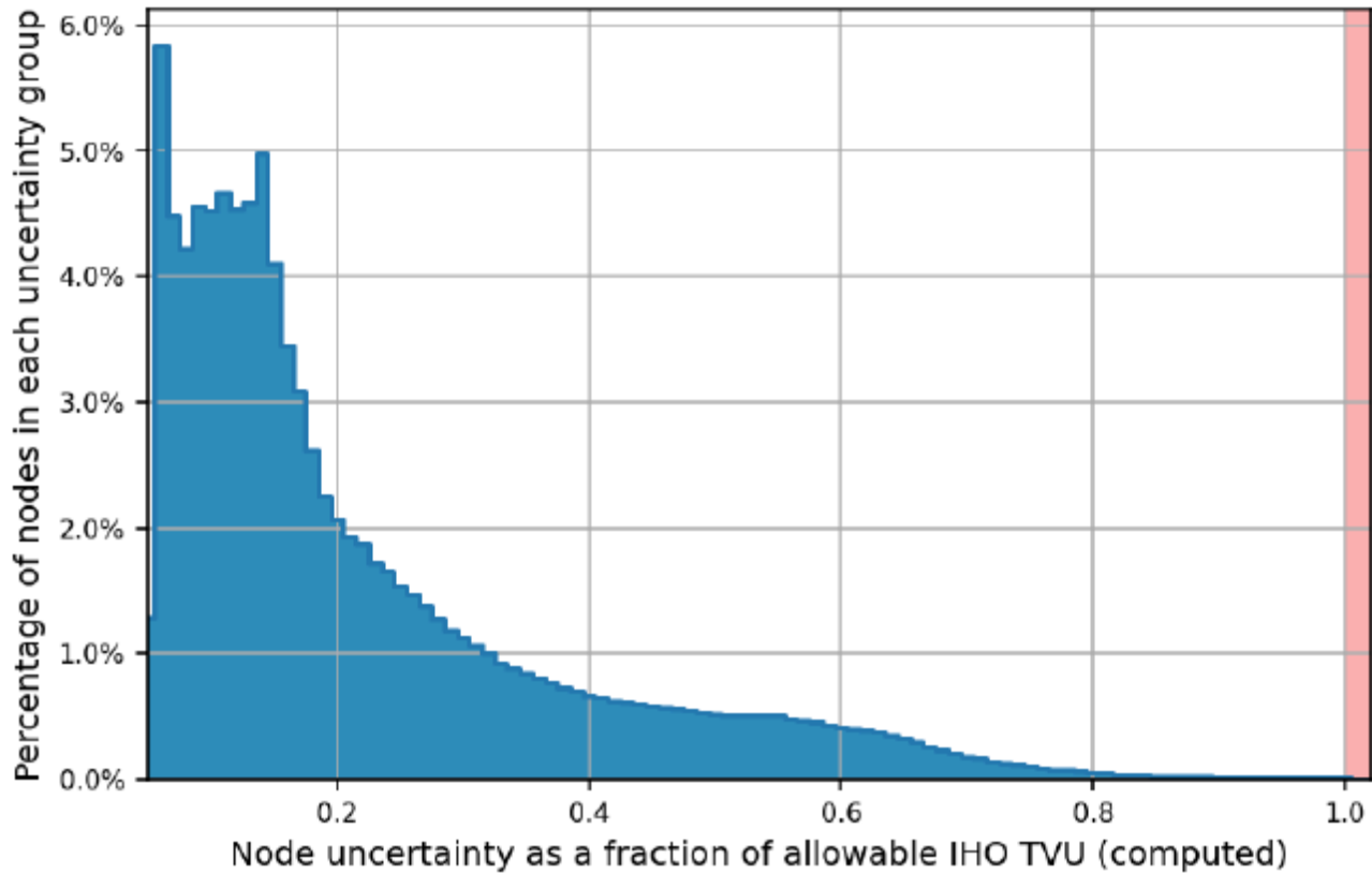
Figure 4: H13625 8m grid allowable uncertainty statistics.
