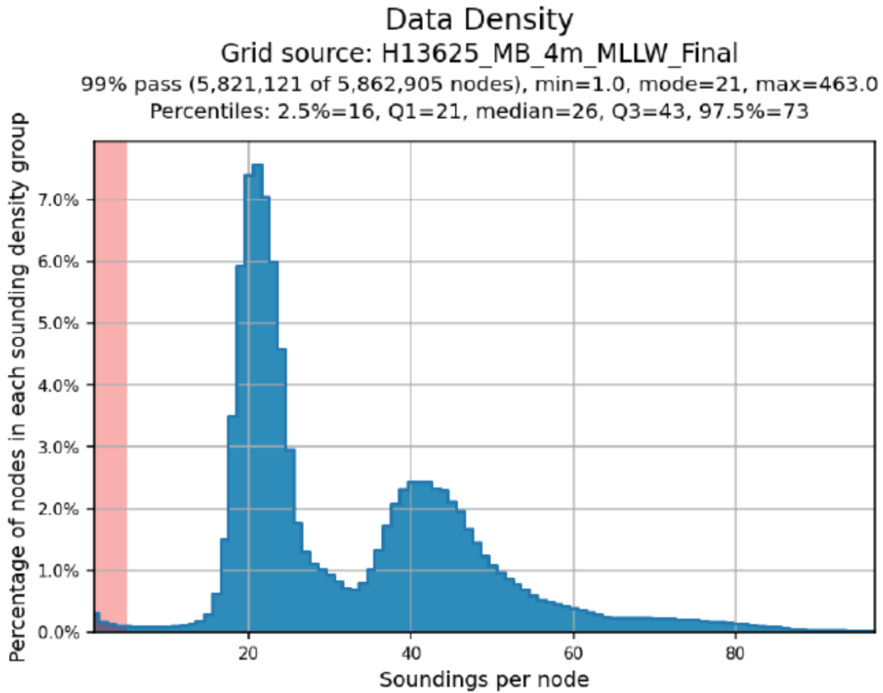
Figure 3: H13625 4m grid data density statistics.
