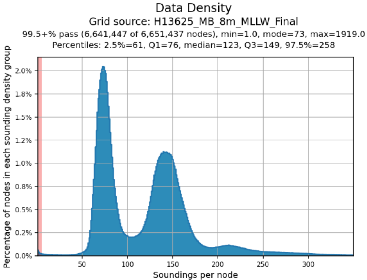
Figure 5: H13625 8m grid data density statistics.
