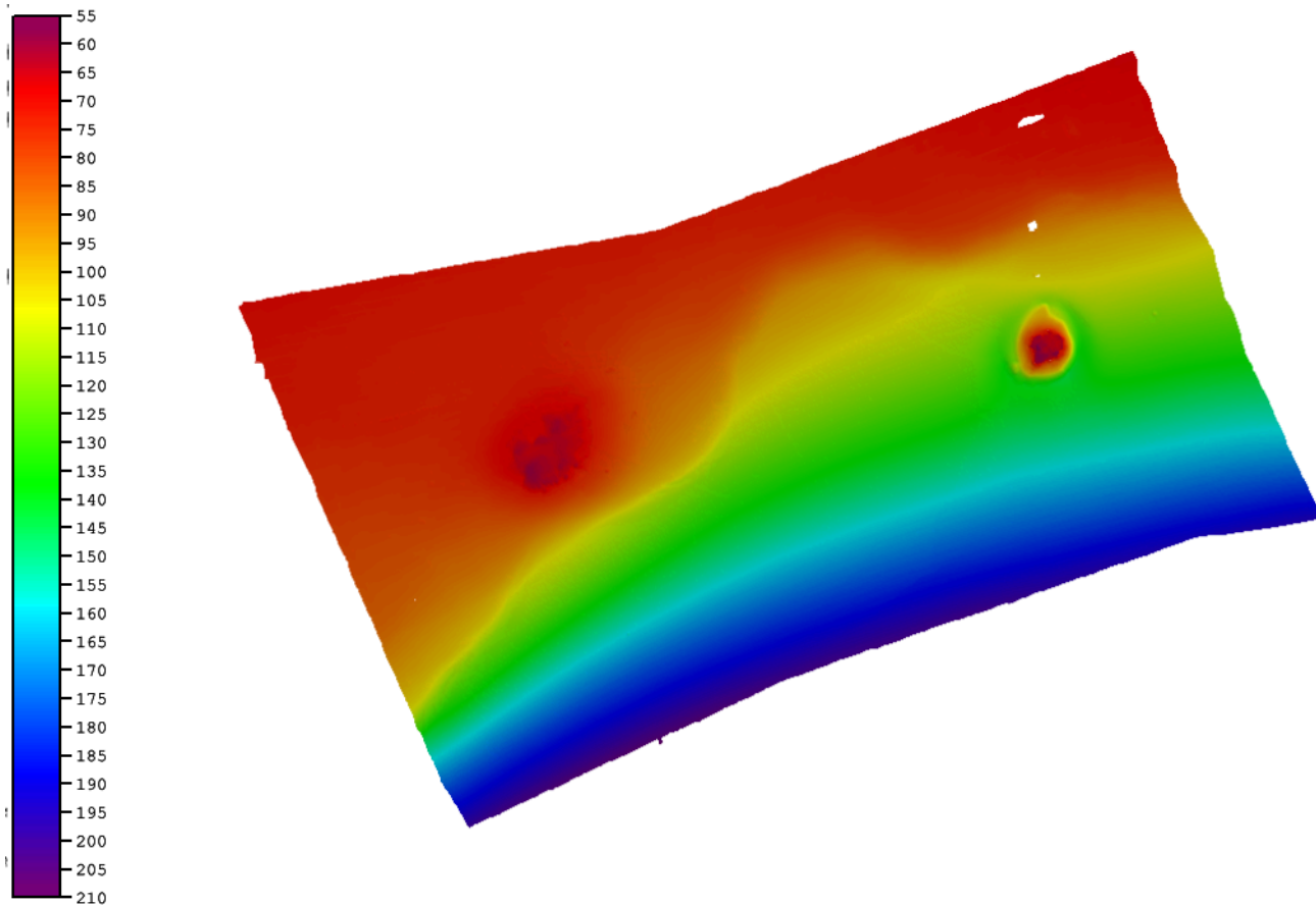
Figure 8: H13627 Coverage overview of combined 4m, 8m, and 16m resolution CUBE grids.
