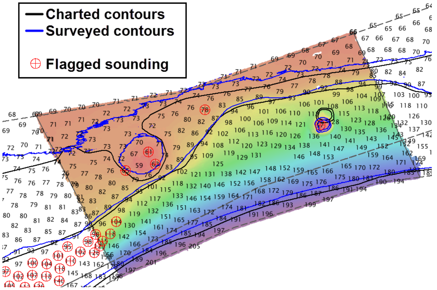
Figure 13: Comparison of charted vs. surveyed depths. Soundings in meters.
