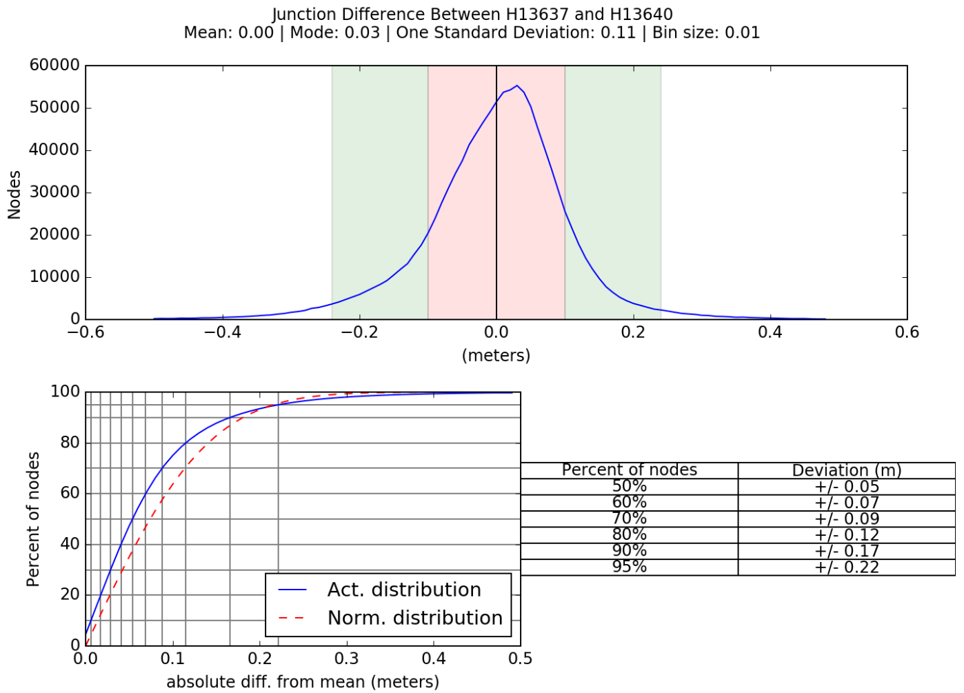
Figure 14: Junction analysis between H13637 and H13640
