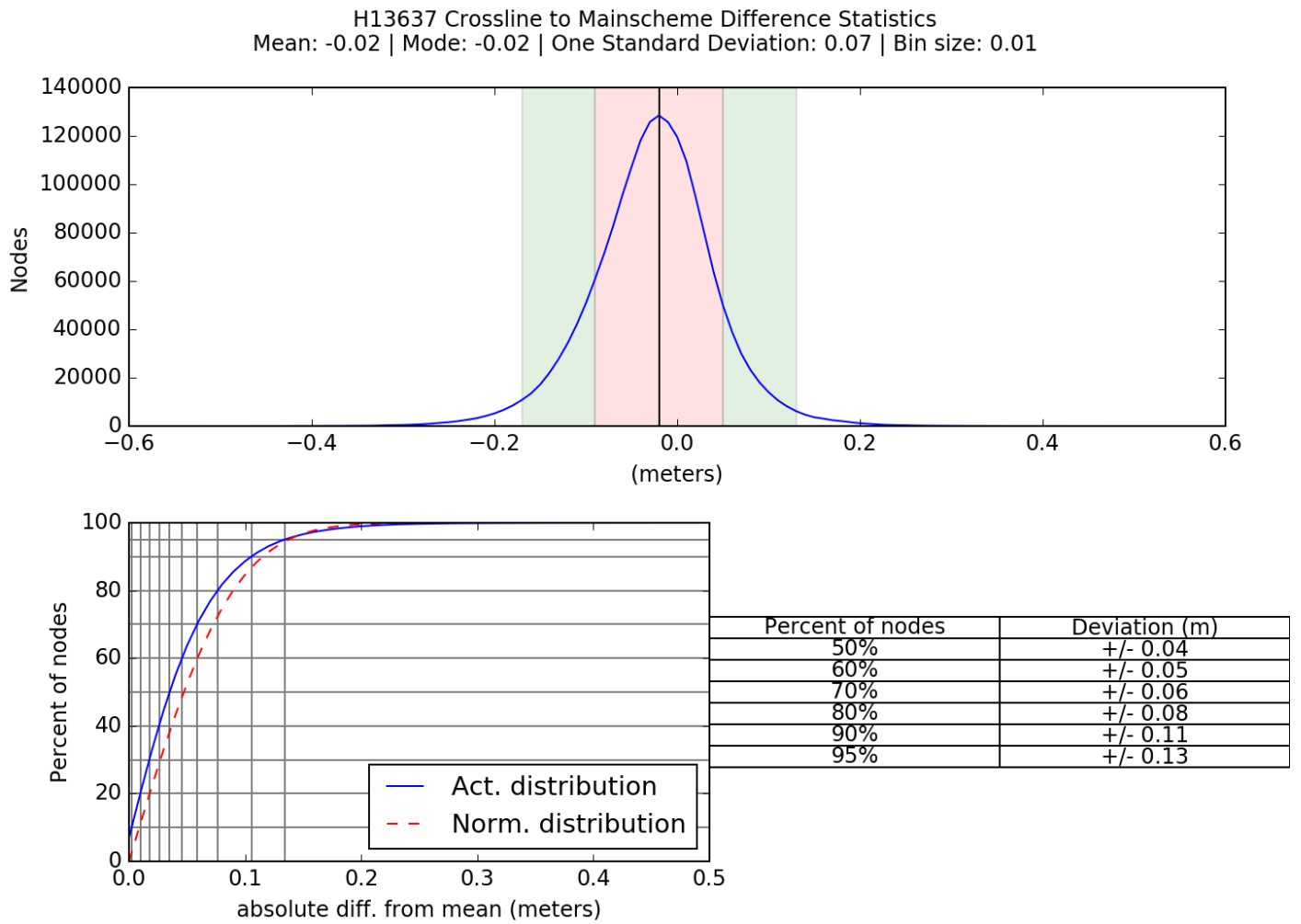
Figure 5: H13637 crossline to mainscheme difference statistics
