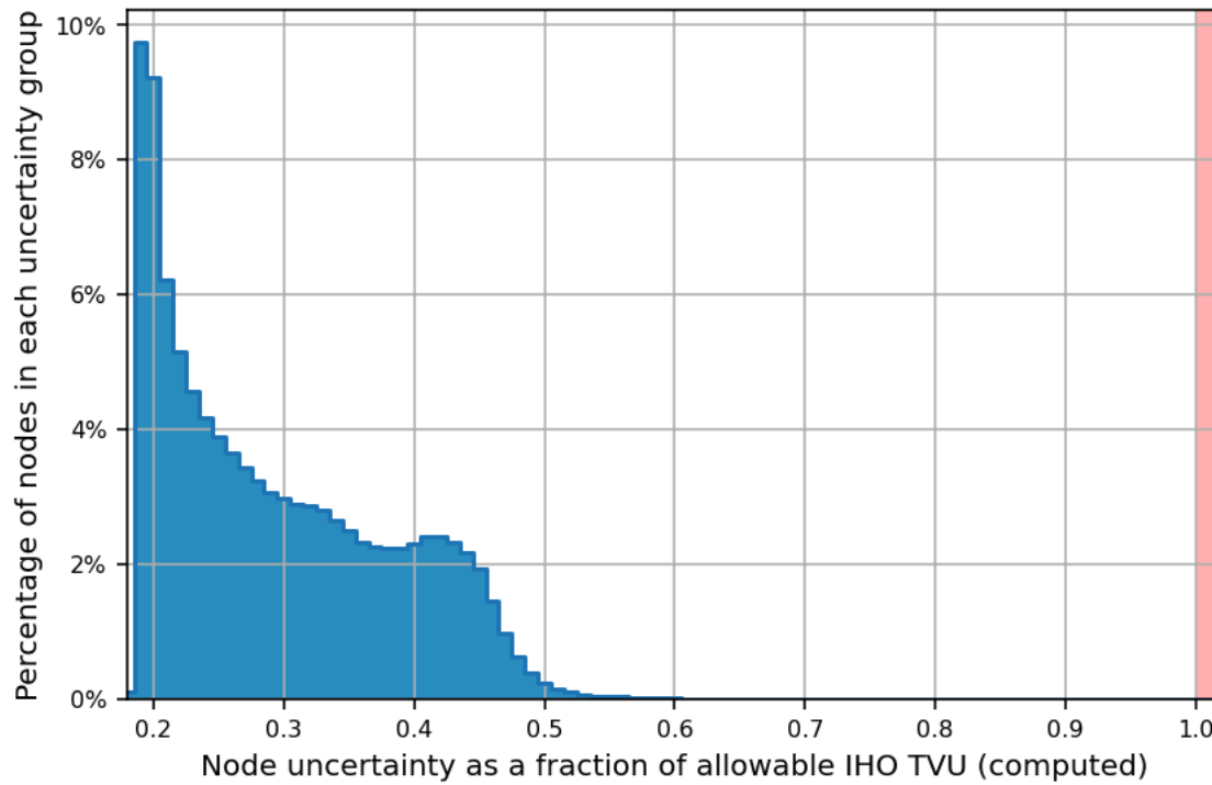
Figure 7: Finalized 2 m CUBE surface TVU statistics for H13637
