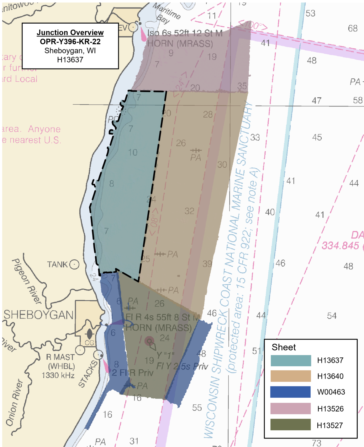
Figure 9: Overview of H13637 junction surveys
