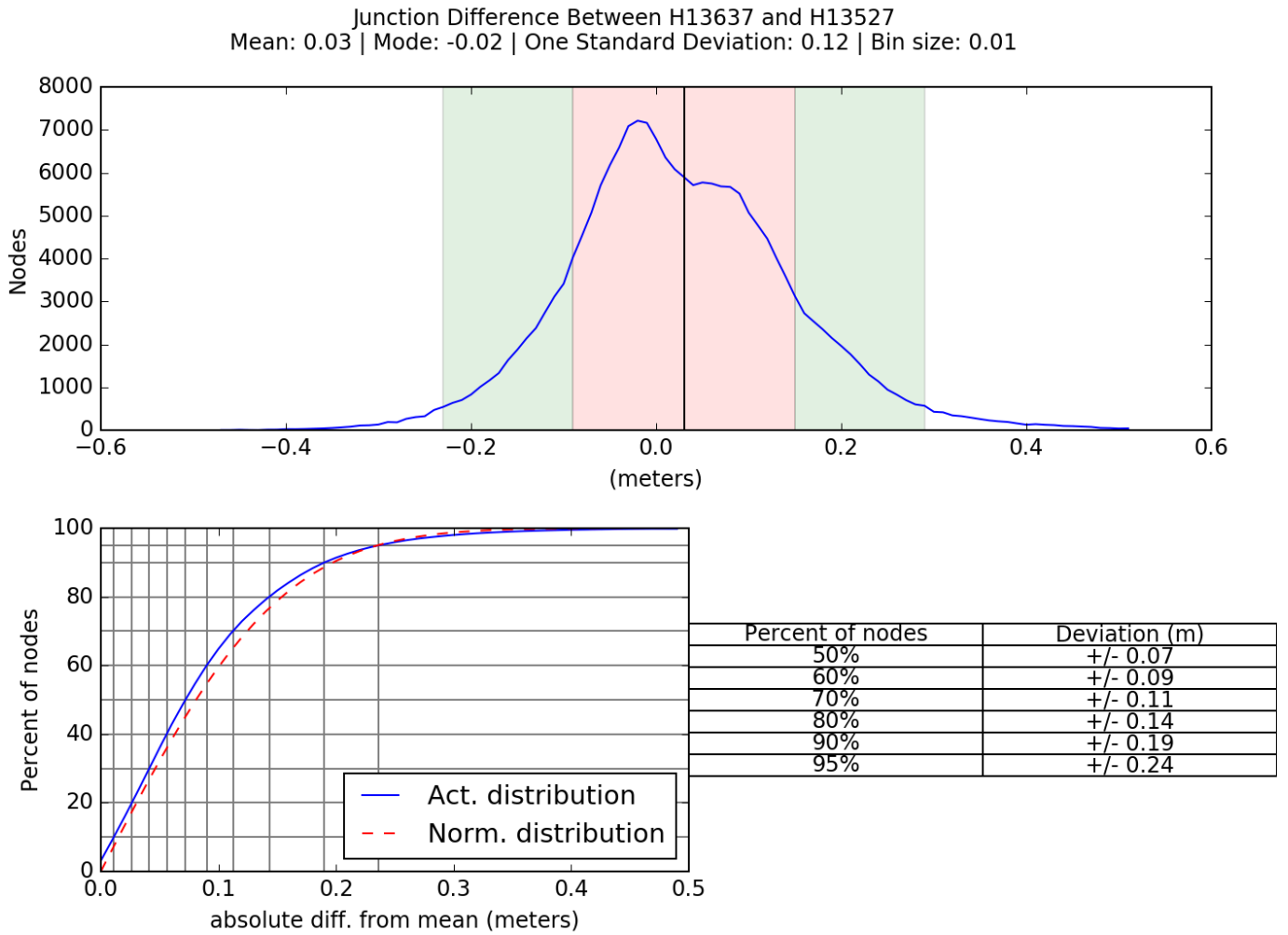
Figure 11: Junction analysis between H13637 and H13527
