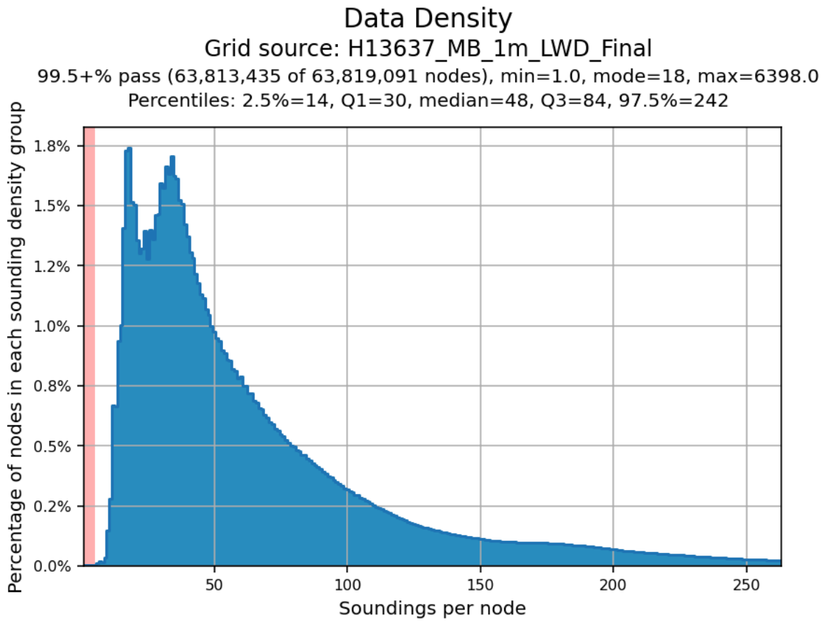
Figure 17: Finalized 1 m CUBE surface density statistics for H13637
