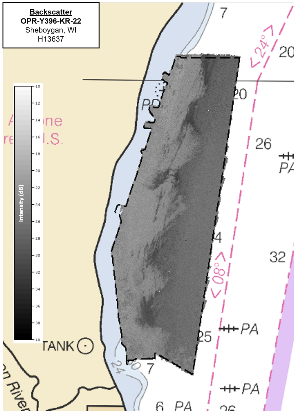
Figure 20: H13637 backscatter
