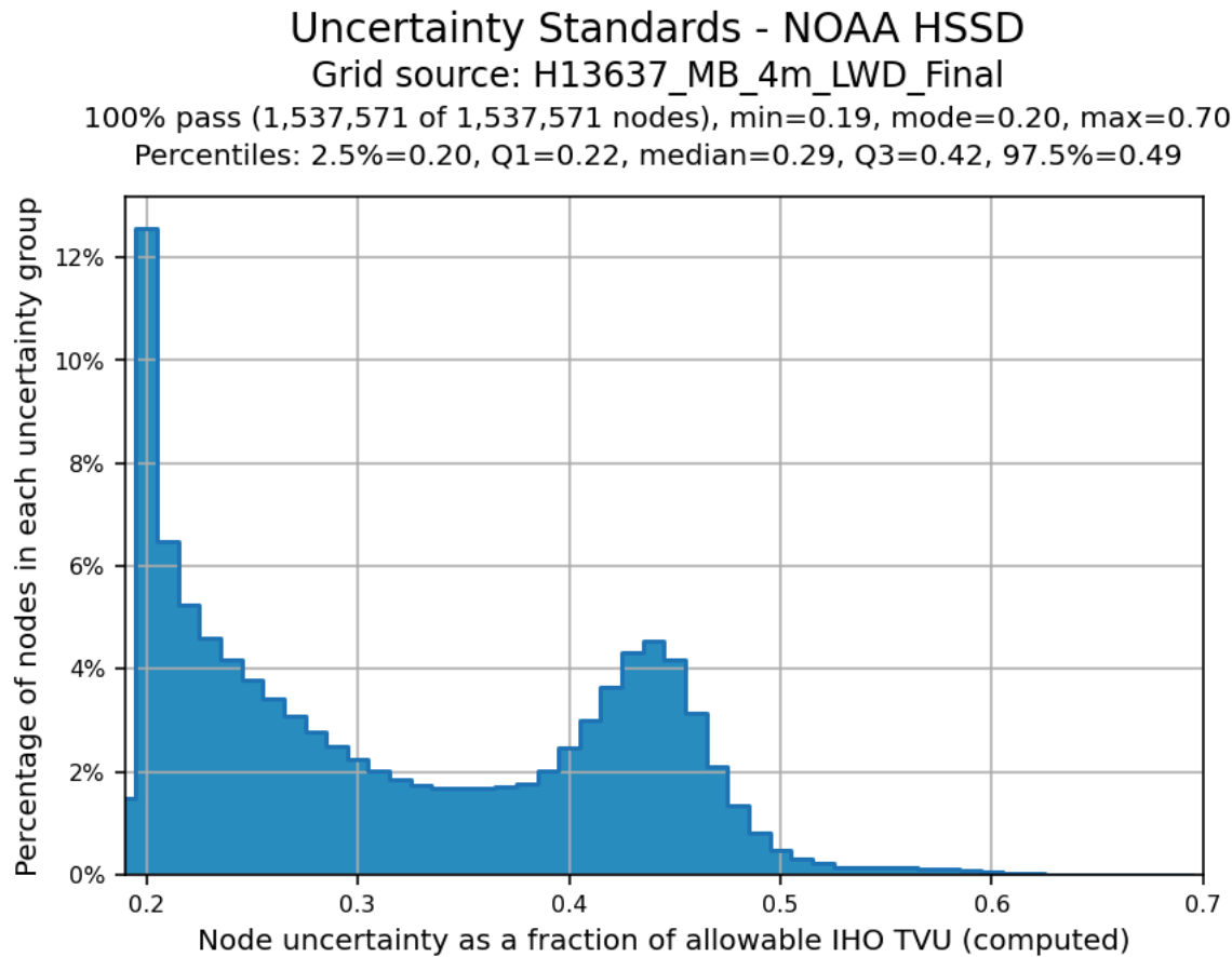
Figure 8: Finalized 4 m CUBE surface TVU statistics for H13637
