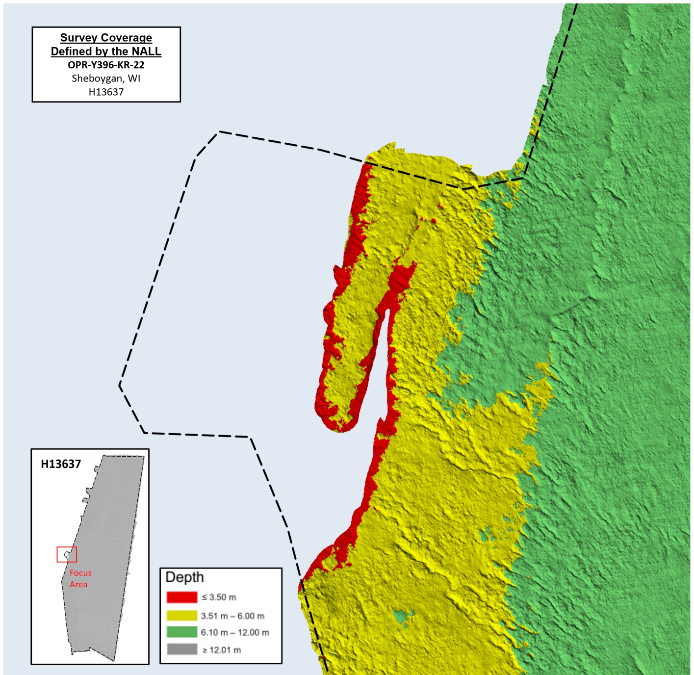
Figure 4: H13637 example of area where survey coverage was defined by the NALL overlaid on Chart 14901
