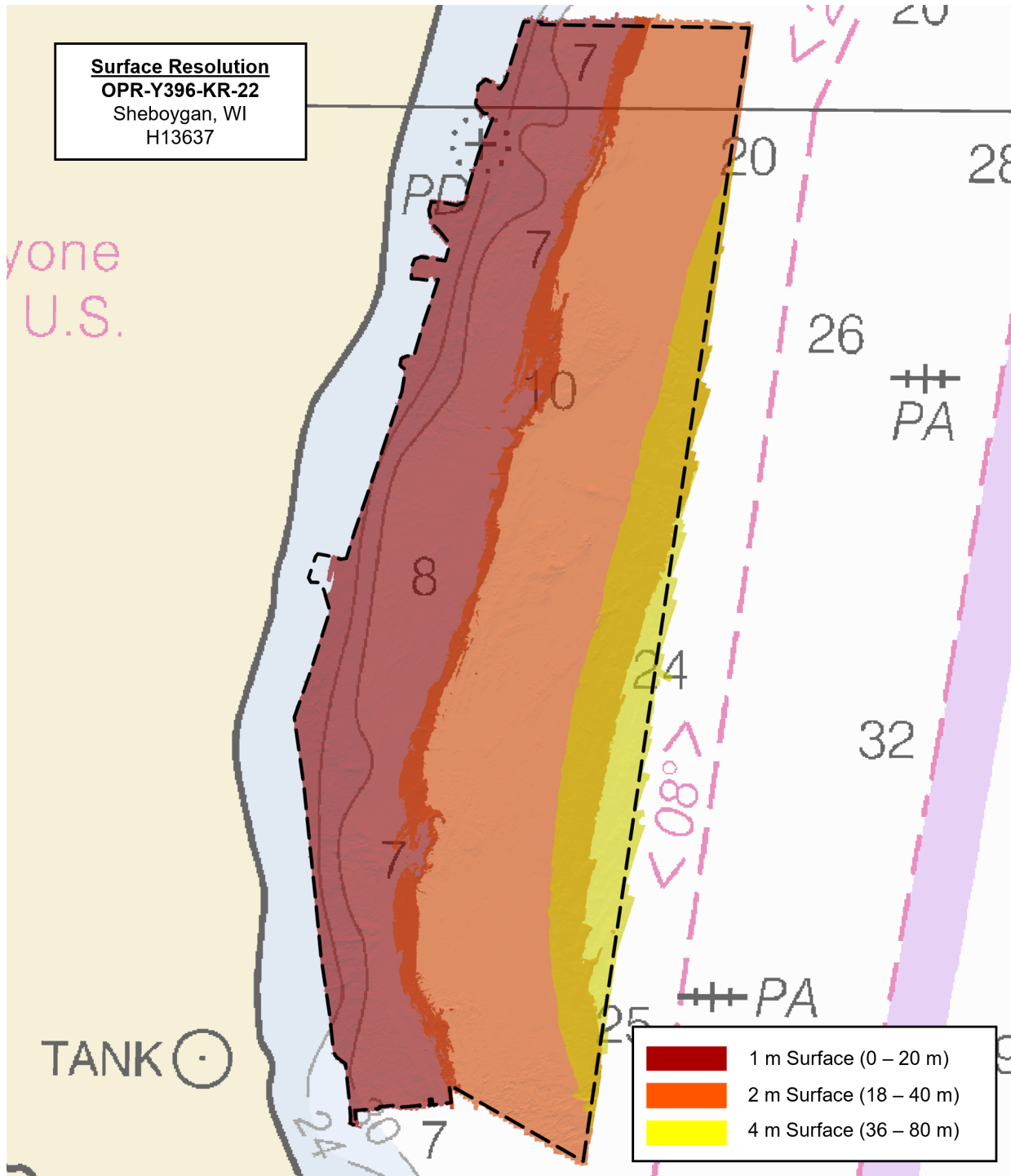
Figure 21: Image representing the finalized CUBE surface resolutions in H13637
