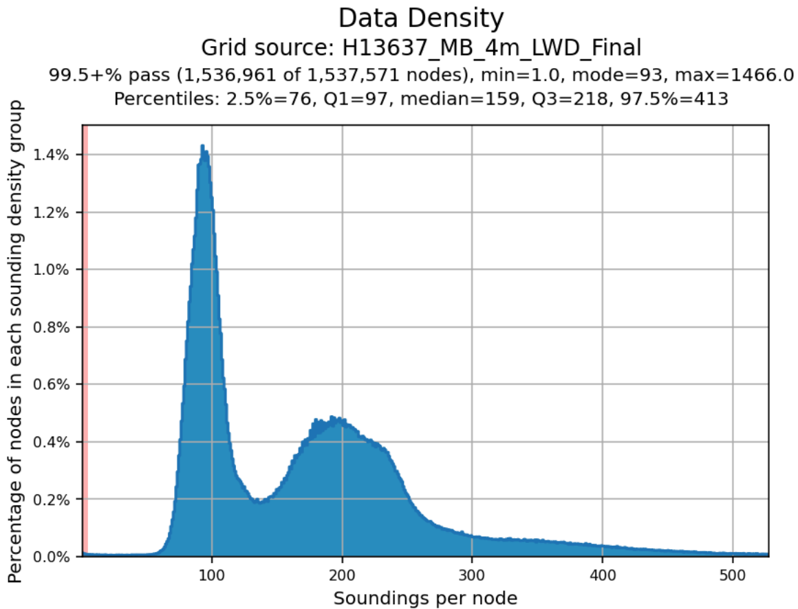
Figure 19: Finalized 4 m CUBE surface density statistics for H13637
