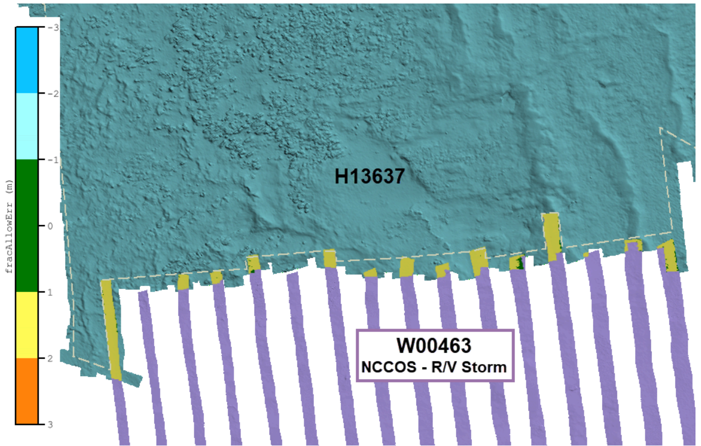
Figure 13: Fraction Allowable Difference surface between H13637 and W00463
