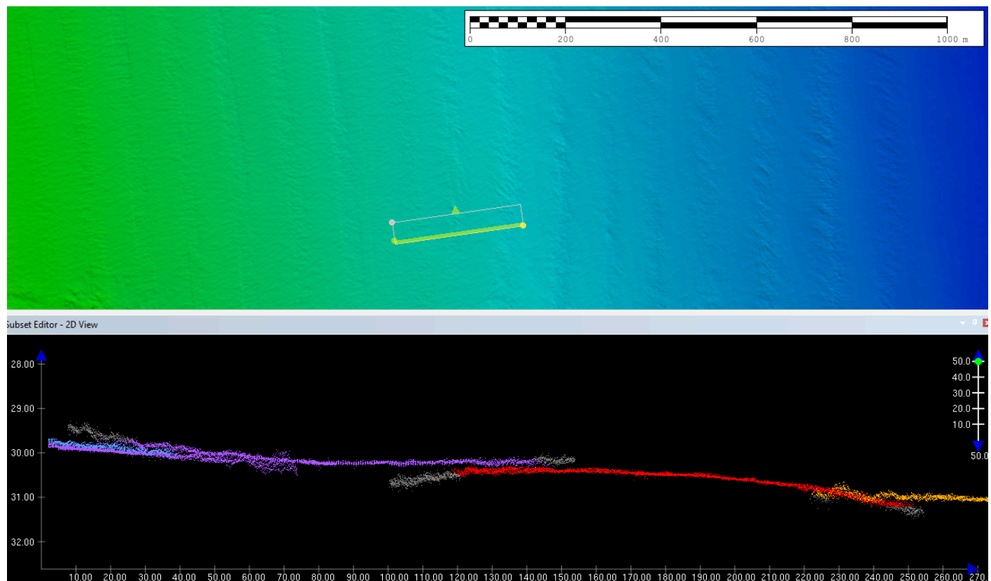
Figure 15: H13637 surface artifacts as a result of refraction causing the soundings to trend concave/convex
