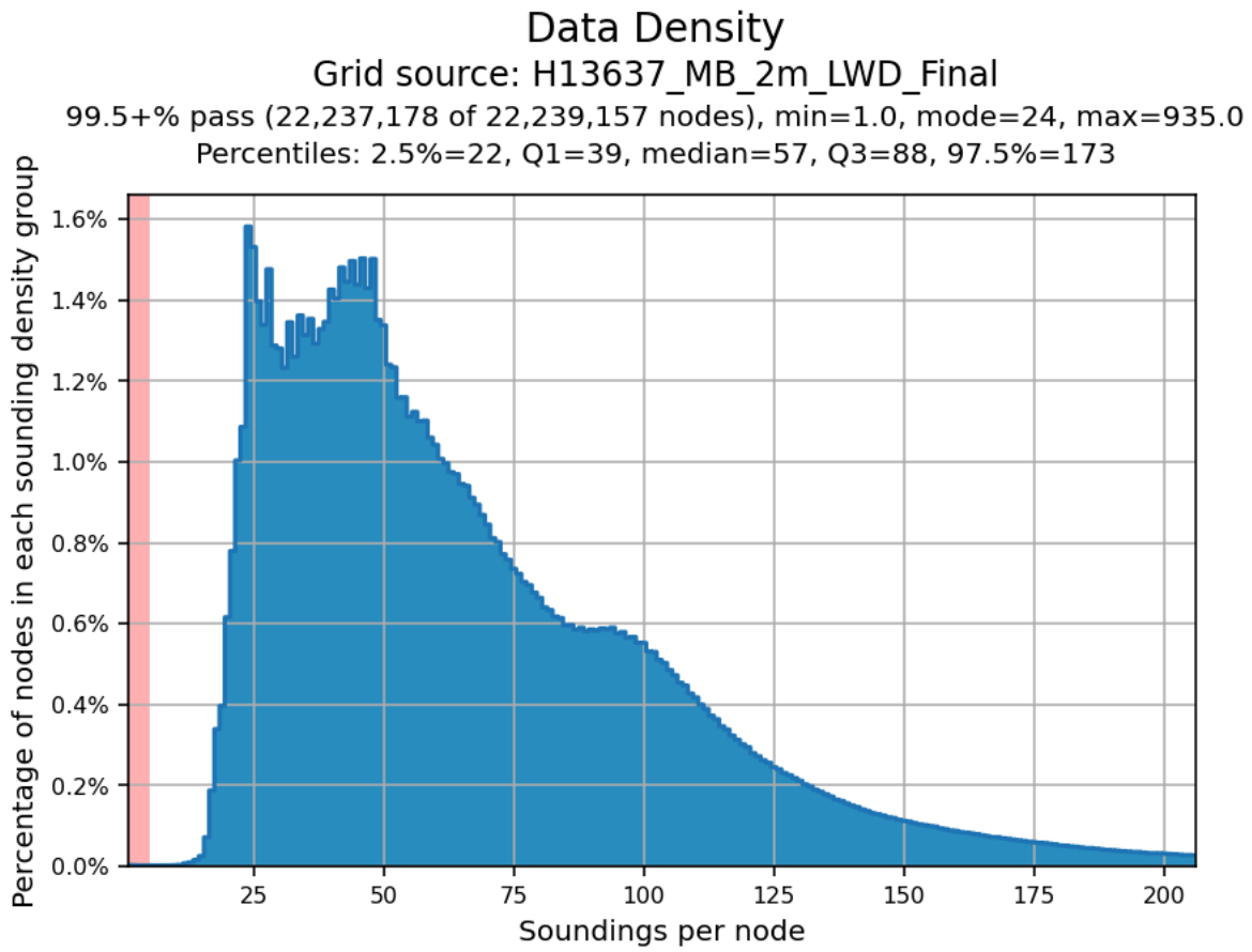
Figure 18: Finalized 2 m CUBE surface density statistics for H13637
