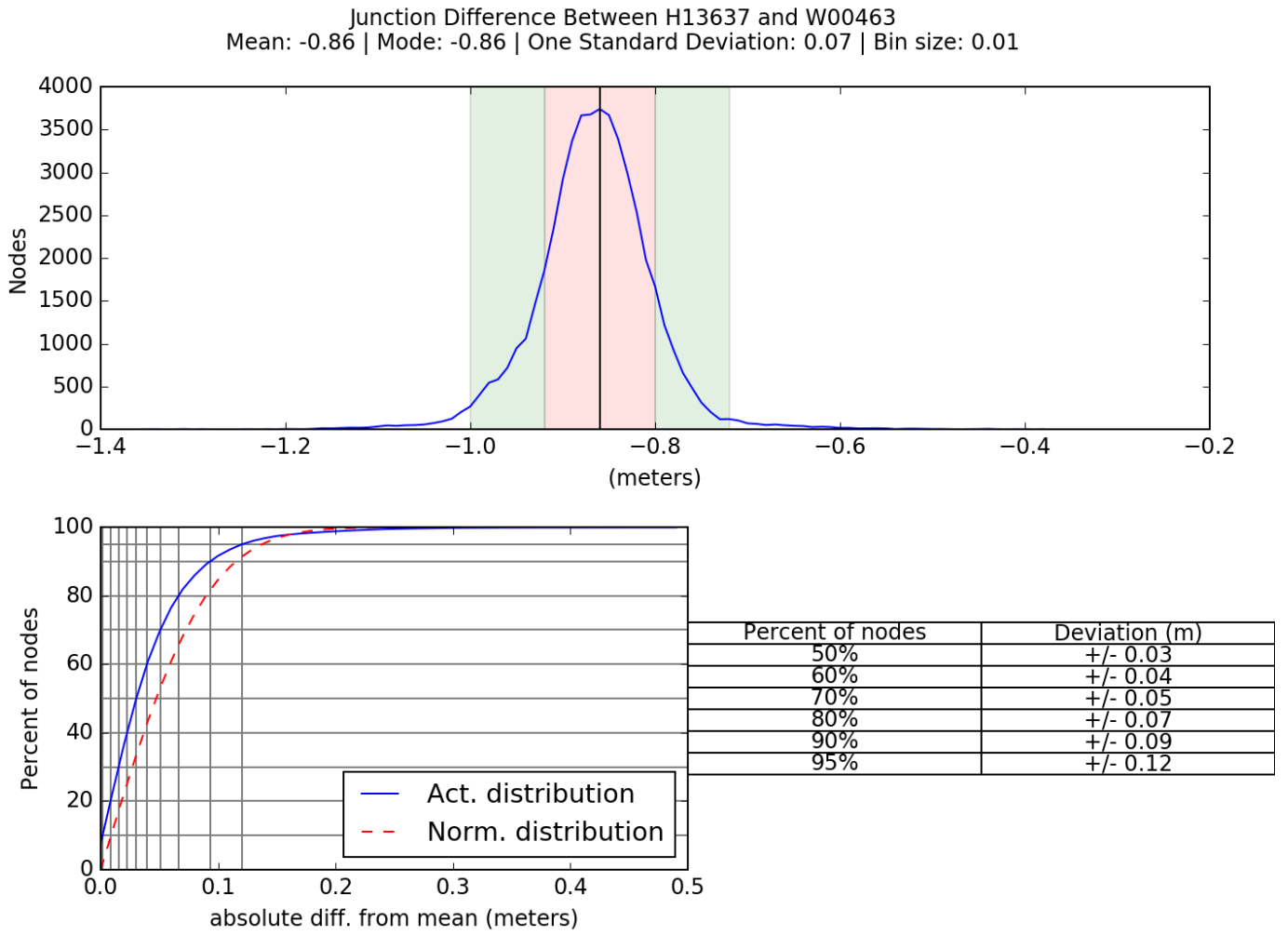
Figure 12: Junction analysis between H13637 and W00463
