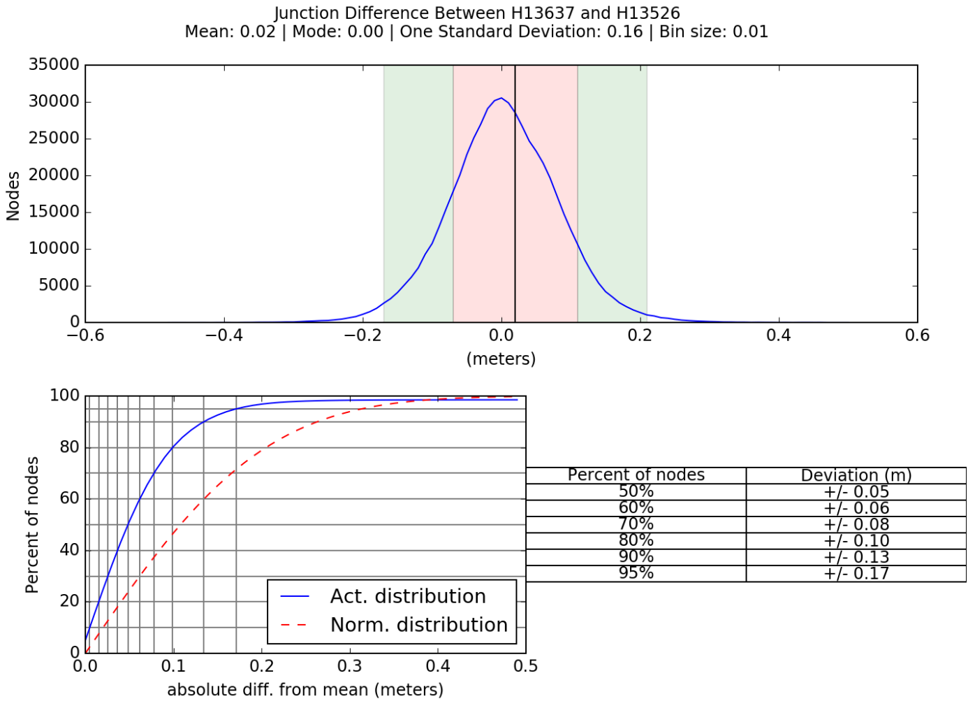
Figure 10: Junction analysis between H13637 and H13526
