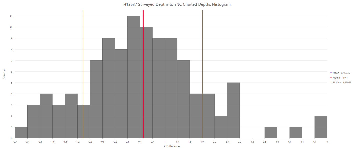
Figure 22: H13637 statistical analysis of surveyed depths to charted depths
