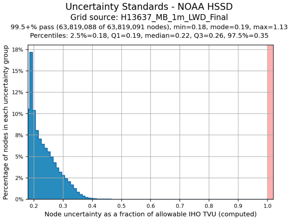
Figure 6: Finalized 1 m CUBE surface TVU statistics for H13637
