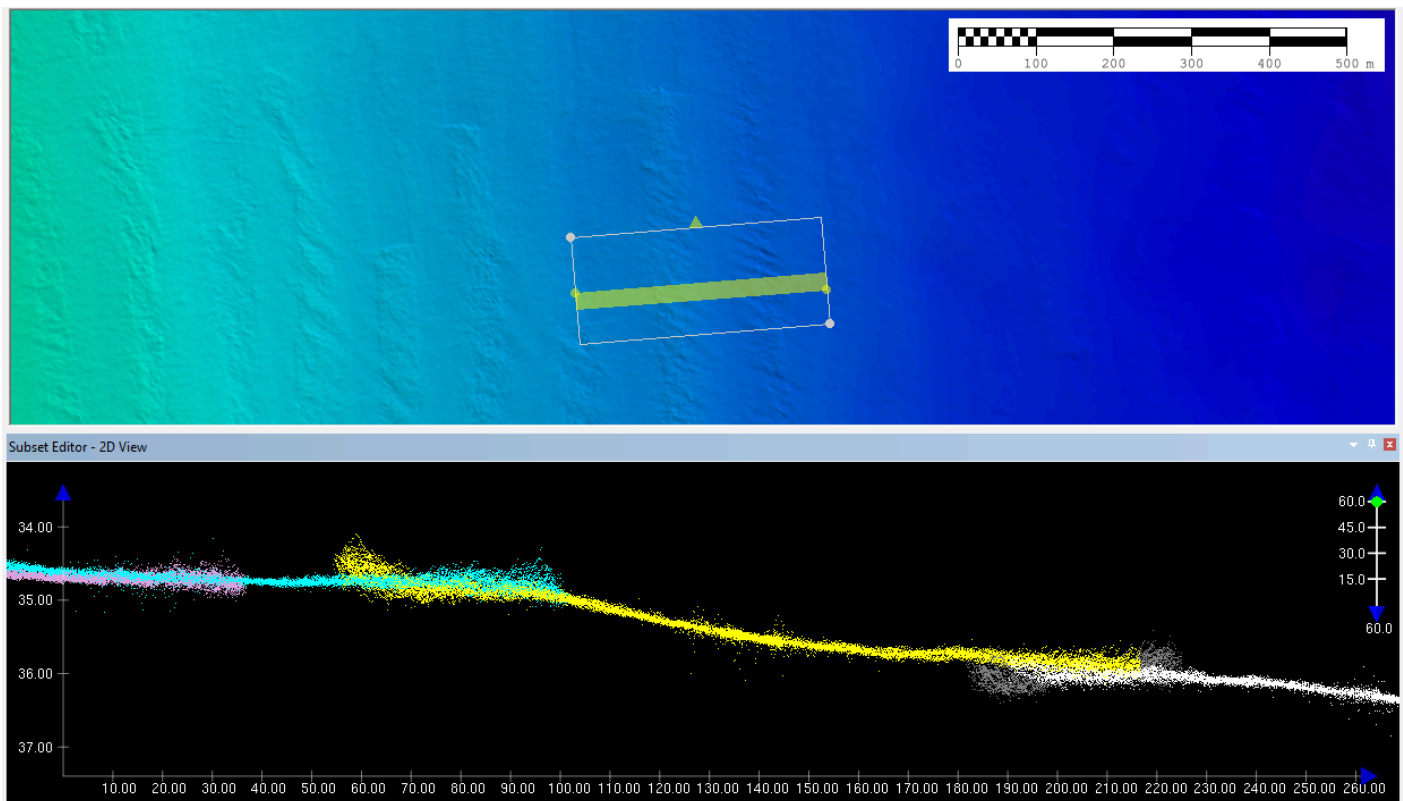
Figure 16: H13637 surface artifacts as a result of refraction causing outer beam noise
