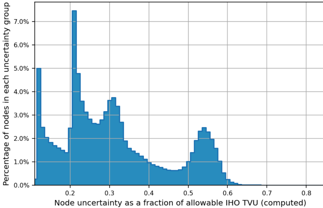
Figure 6: Finalized 8 m CUBE surface TVU statistics for H13641
