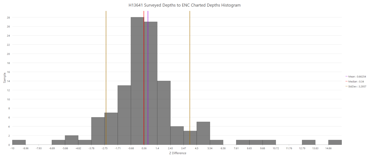
Figure 20: H13641 statistical analysis of surveyed depths to charted depths
