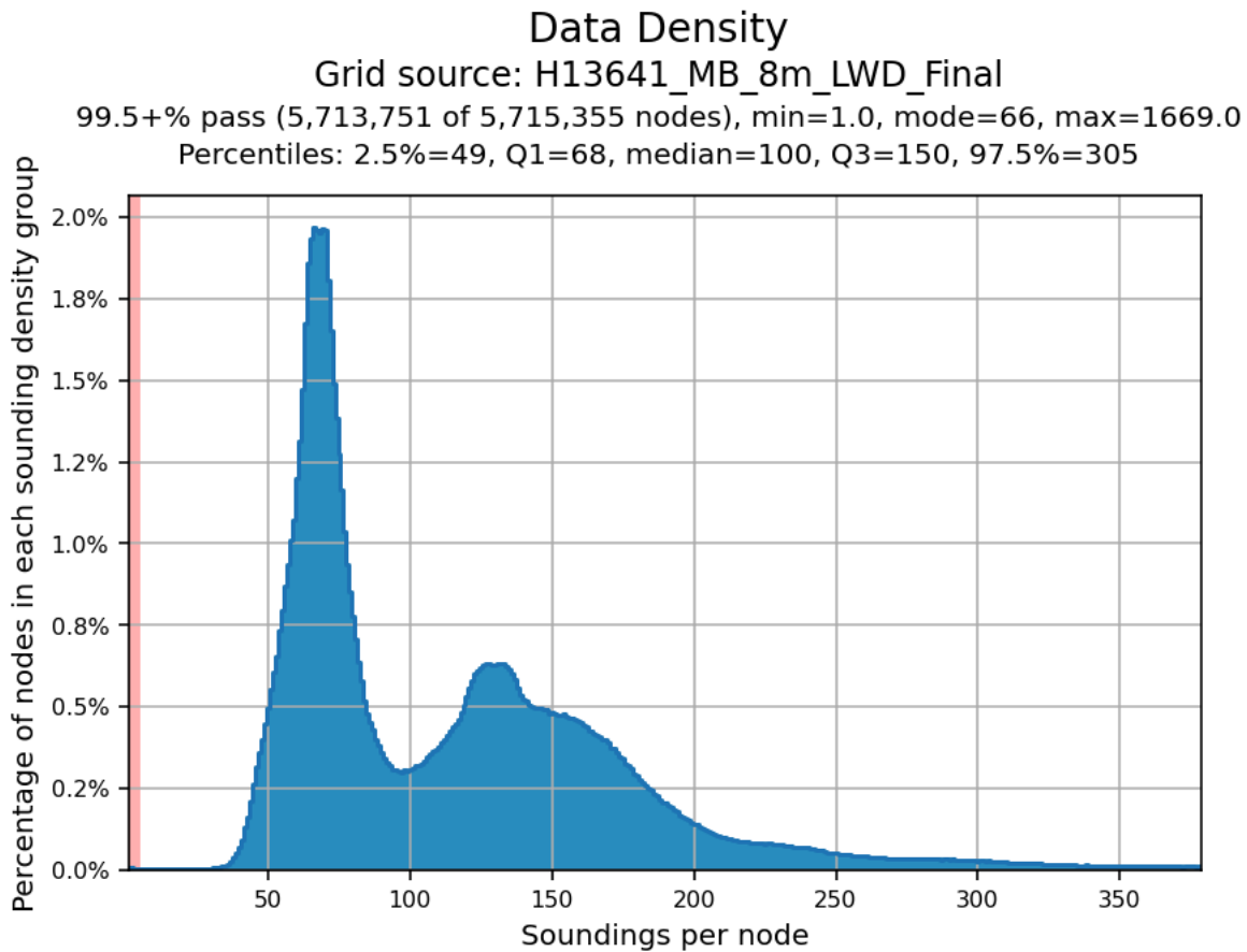
Figure 17: Finalized 8 m CUBE surface density statistics for H13641
