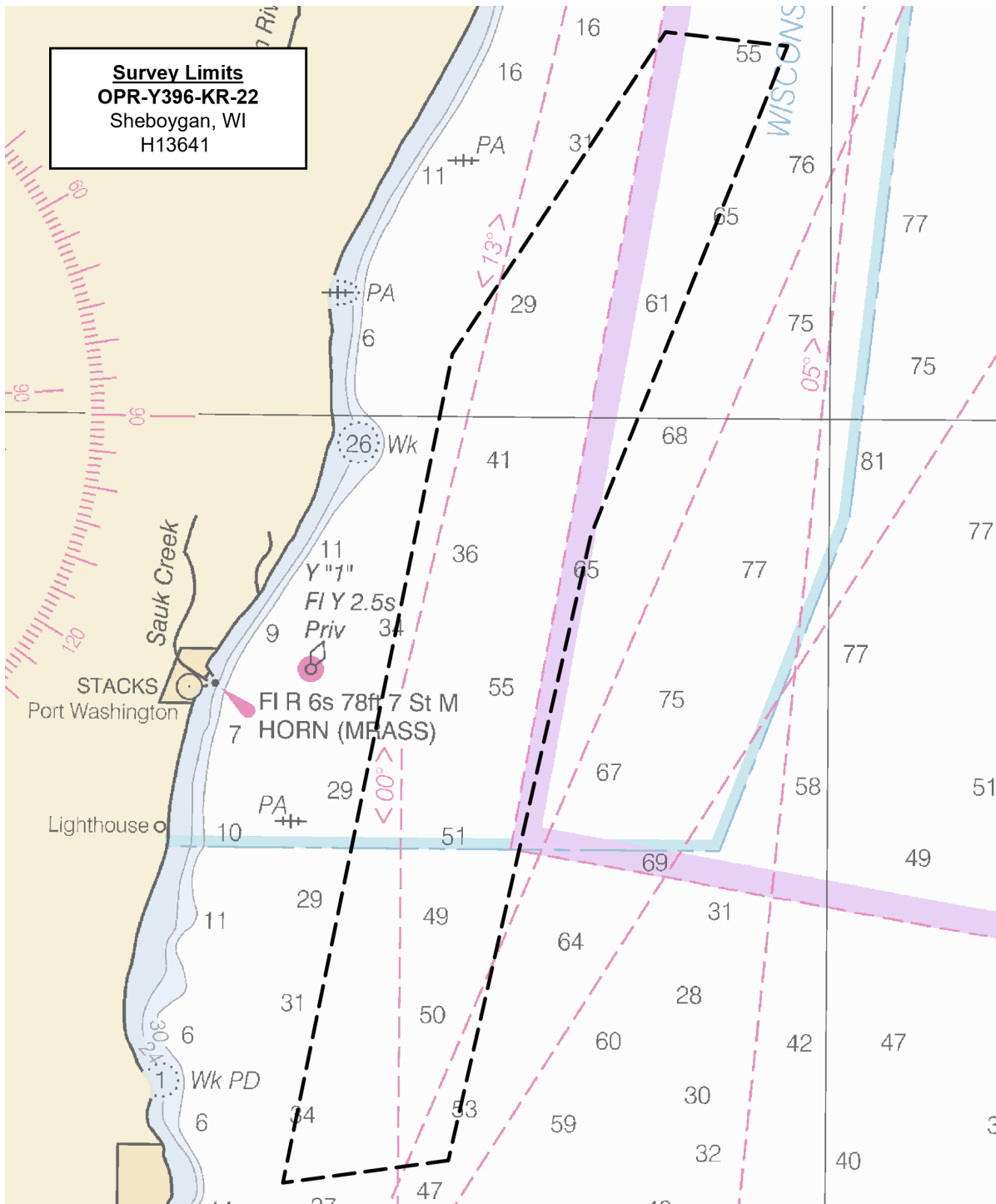
Figure 2: H13641 survey limits overlaid onto Chart 14901
