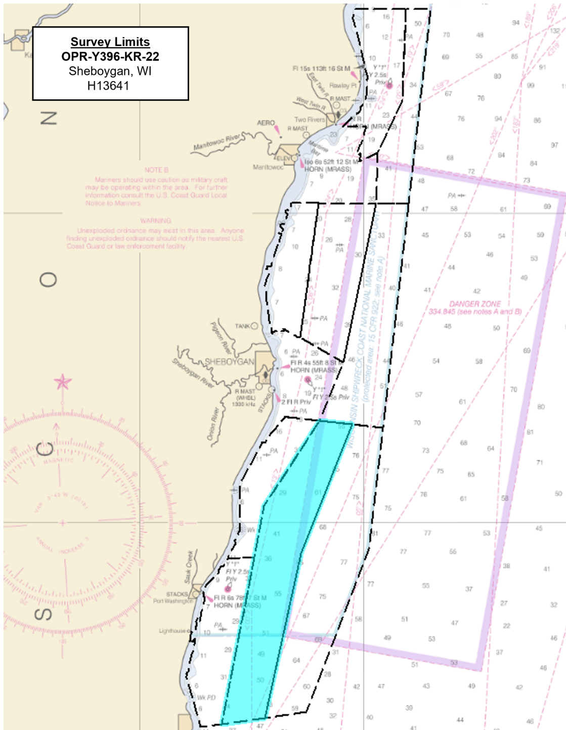
Figure 1: Overview of project survey limits (H13641 shown in blue), overlaid onto Chart 14901
