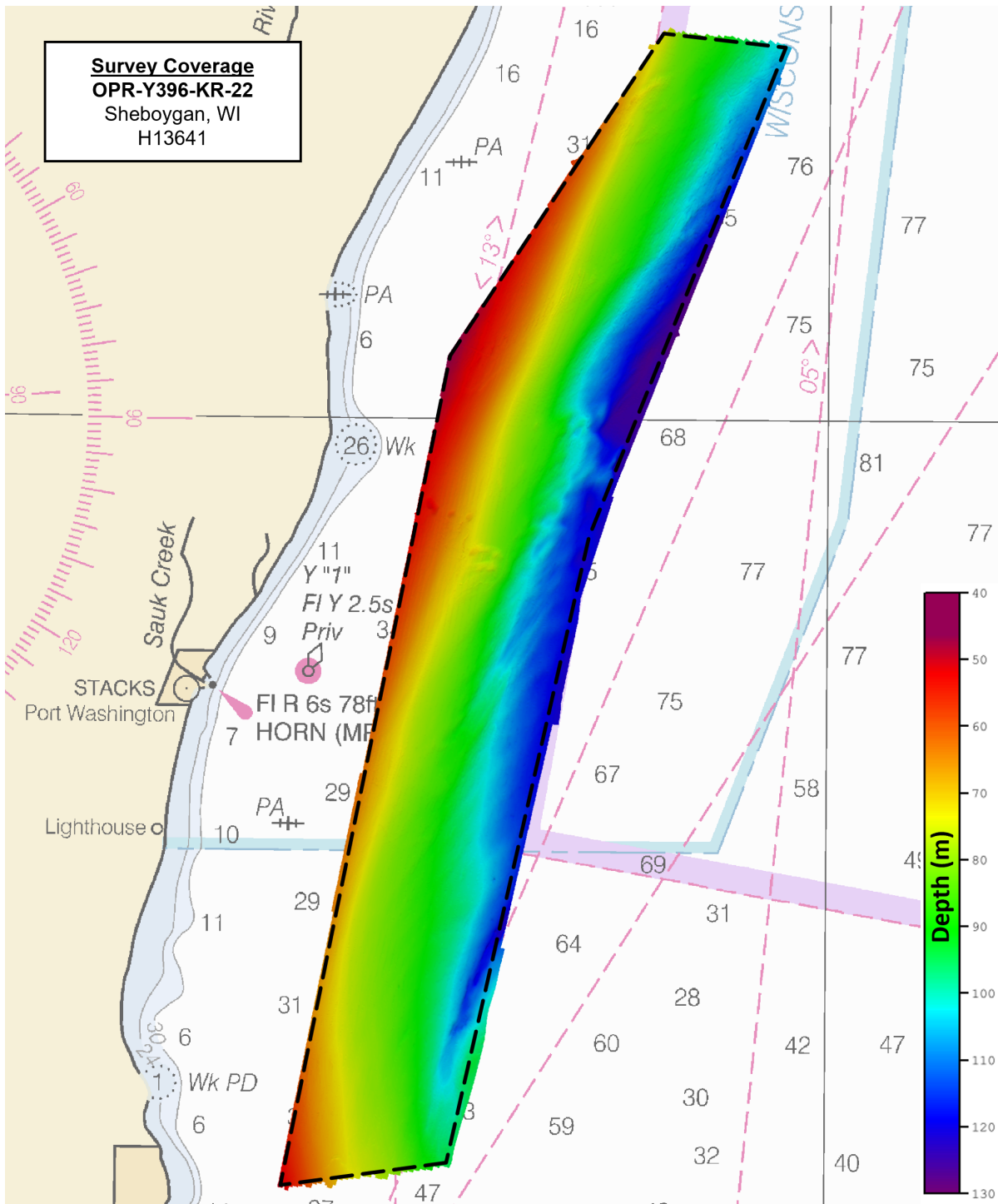
Figure 3: H13641 survey coverage overlaid onto Chart 14901
