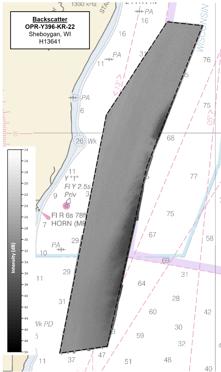
Figure 18: H13641 backscatter
