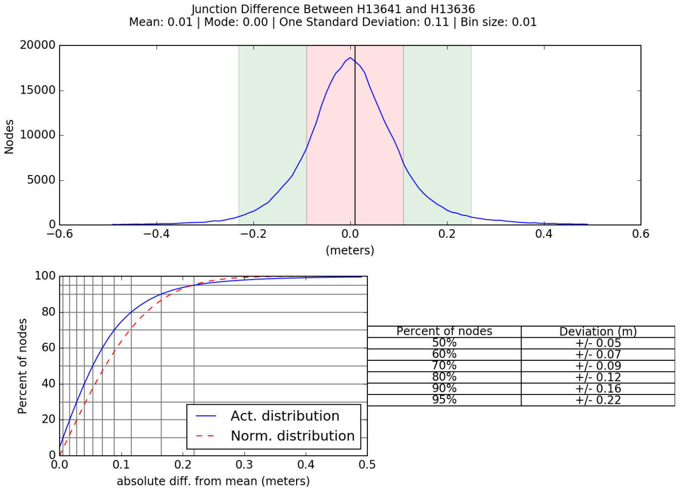
Figure 11: Junction analysis between H13641 and H13636
