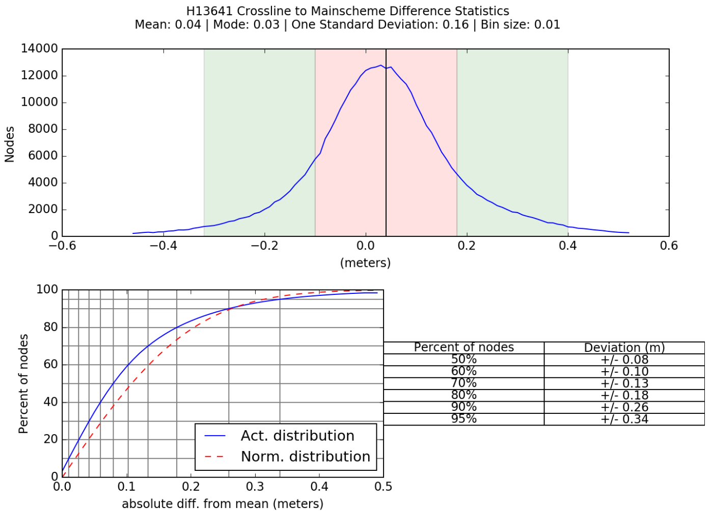
Figure 4: H13641 crossline to mainscheme difference statistics
