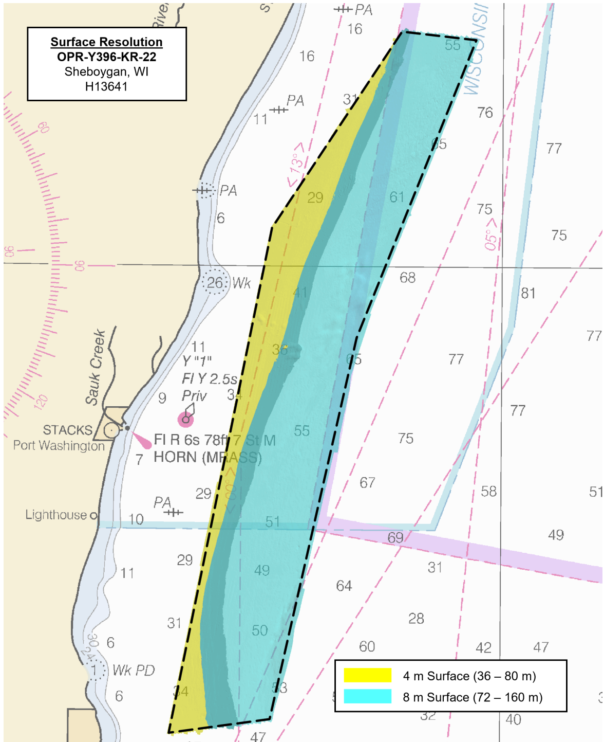
Figure 19: Image representing the finalized CUBE surface resolutions in H13641
