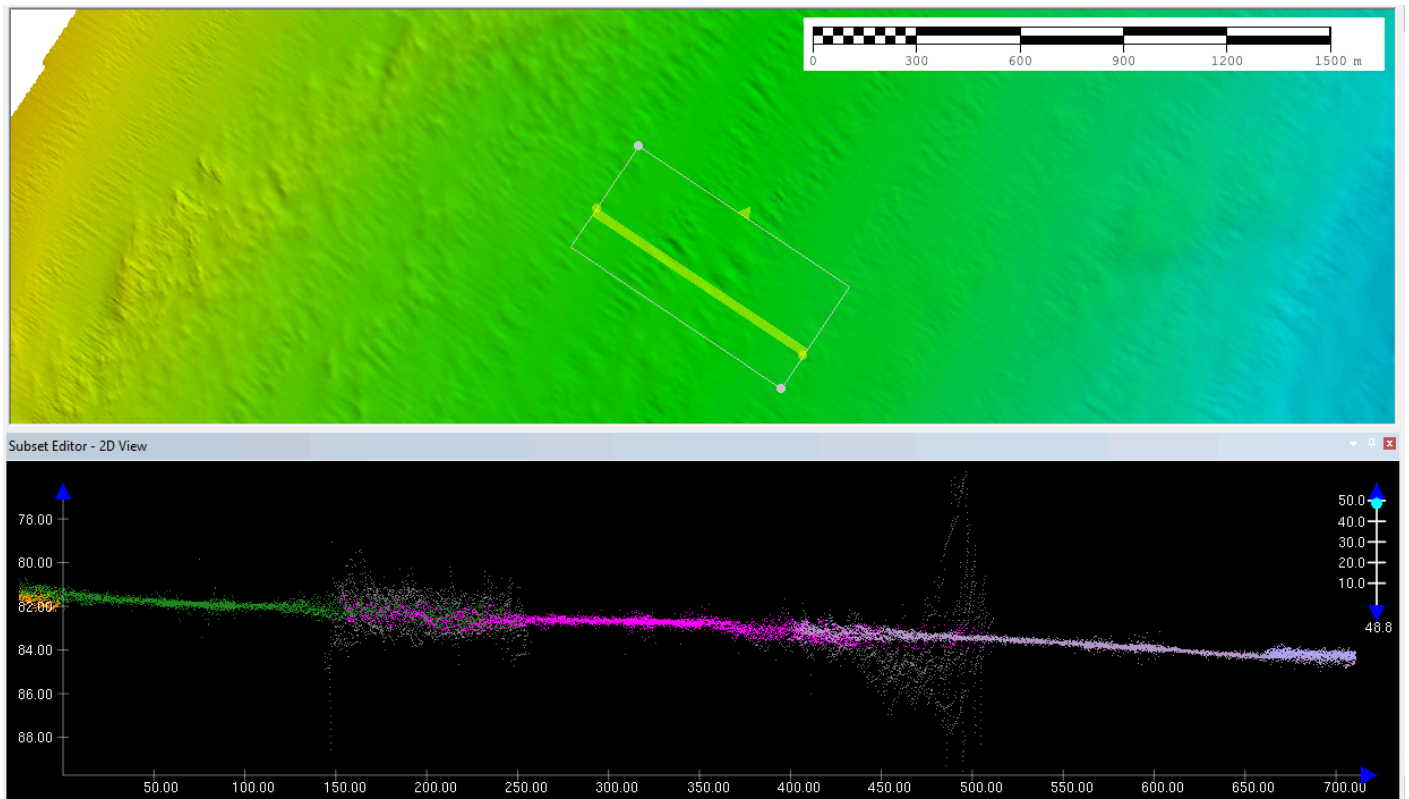
Figure 15: H13641 surface artifacts as a result of refraction causing outer beam noise
