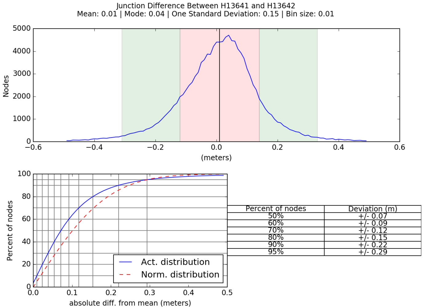
Figure 12: Junction analysis between H13641 and H13642
