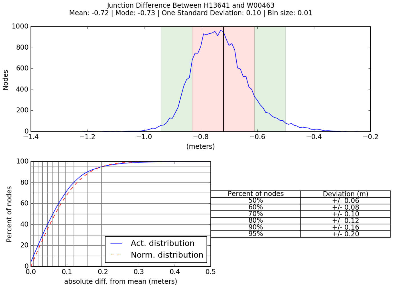
Figure 8: Junction analysis between H13641 and W00463
