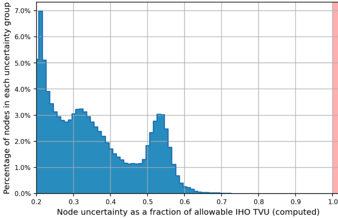
Figure 5: Finalized 4 m CUBE surface TVU statistics for H13641
