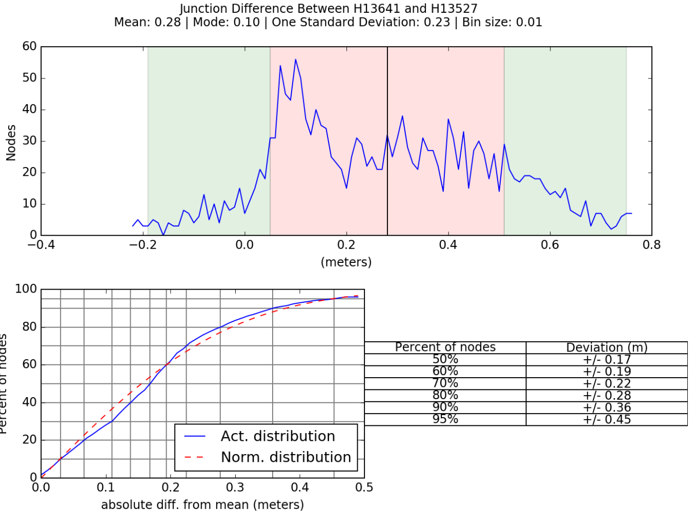
Figure 9: Junction analysis between H13641 and H13527
