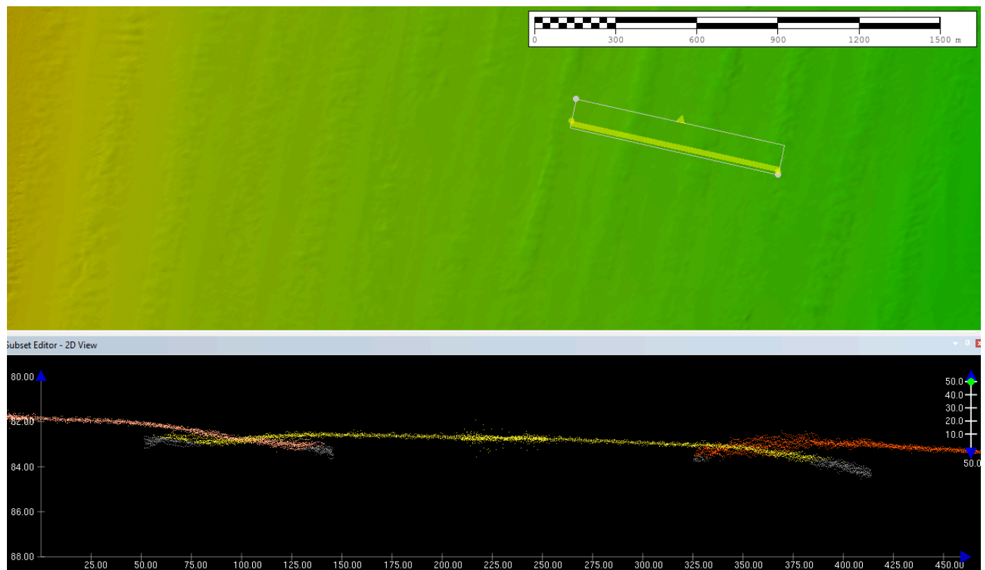
Figure 14: H13641 surface artifacts as a result of refraction causing the soundings to trend concave/convex
