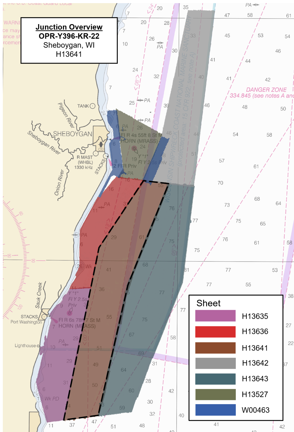
Figure 7: Overview of H13641 junction surveys
