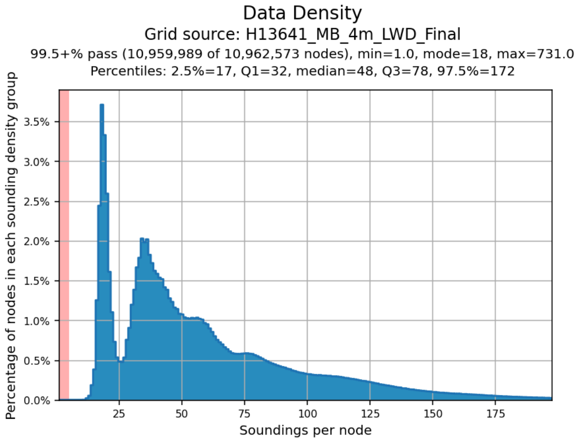
Figure 16: Finalized 4 m CUBE surface density statistics for H13641
