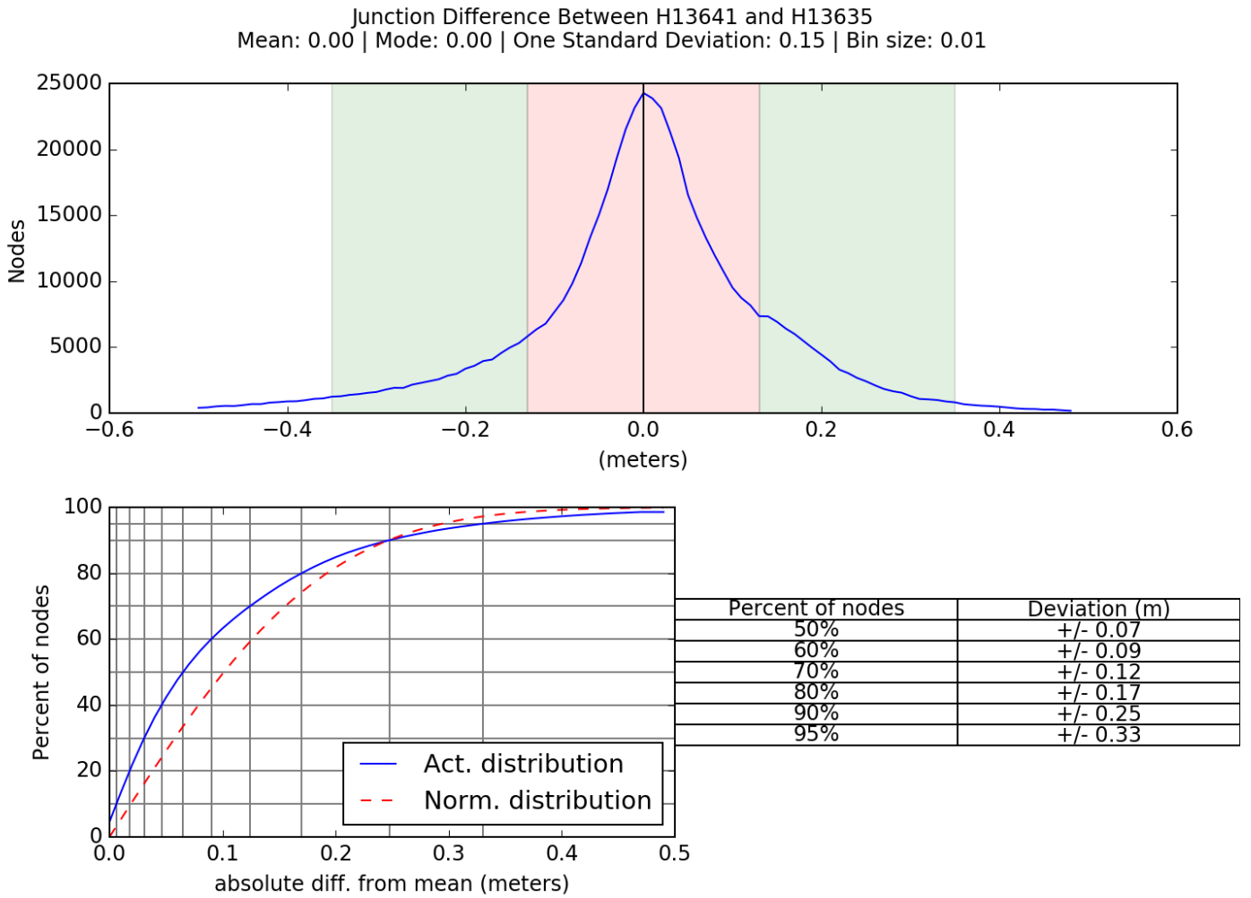
Figure 10: Junction analysis between H13641 and H13635
