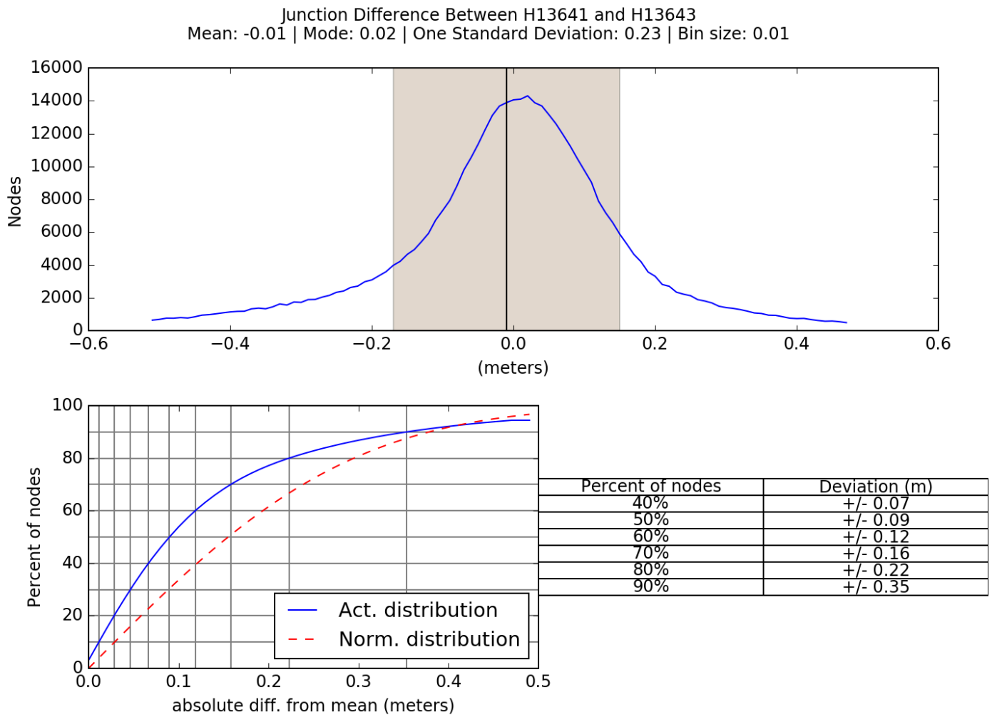
Figure 13: Junction analysis between H13641 and H13643
